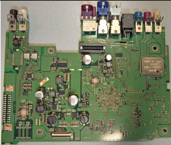
Powerboard TOP
