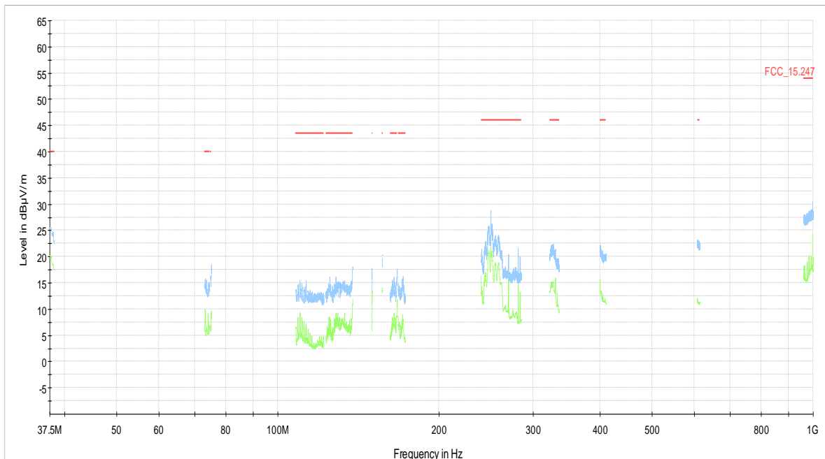
30 MHz – 1 GHz: BT GFSK (1-DH1), CH 39
