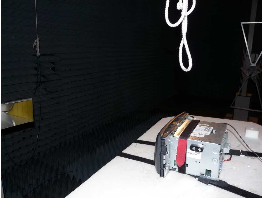
Photo 3: Setup for radiated measurements above 1 GHz
