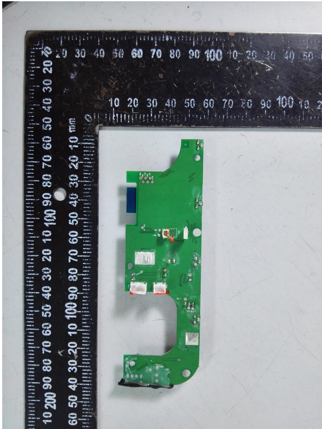
Fig. 2: Internal view
