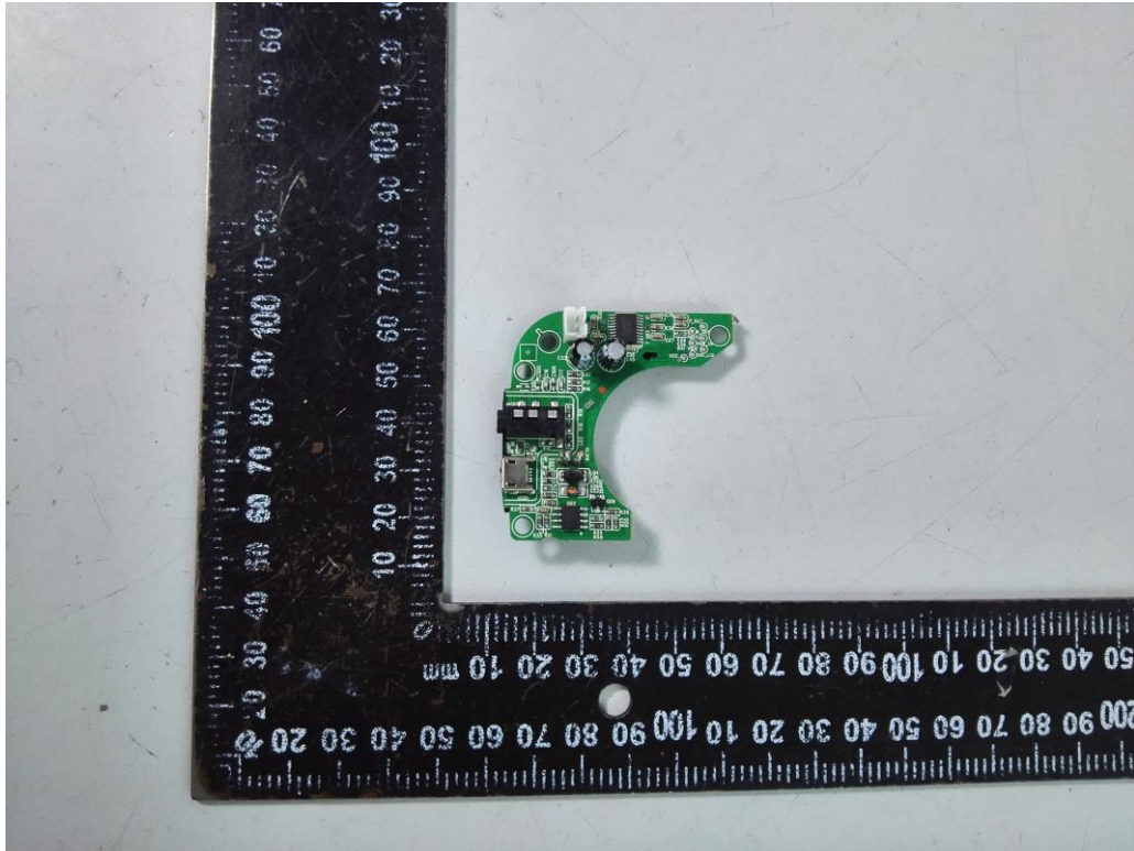
Fig. 5: Internal view
