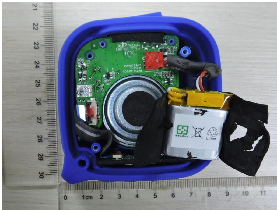
Fig. 2: Internal view
