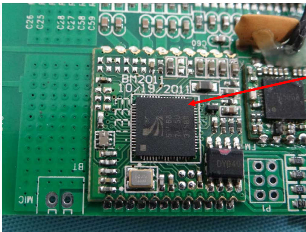
Bluetooth Chip
