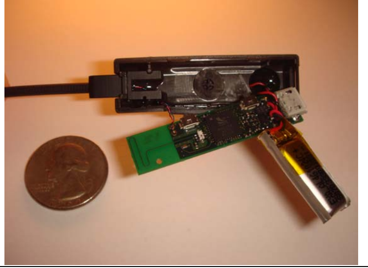
PWB Front View
