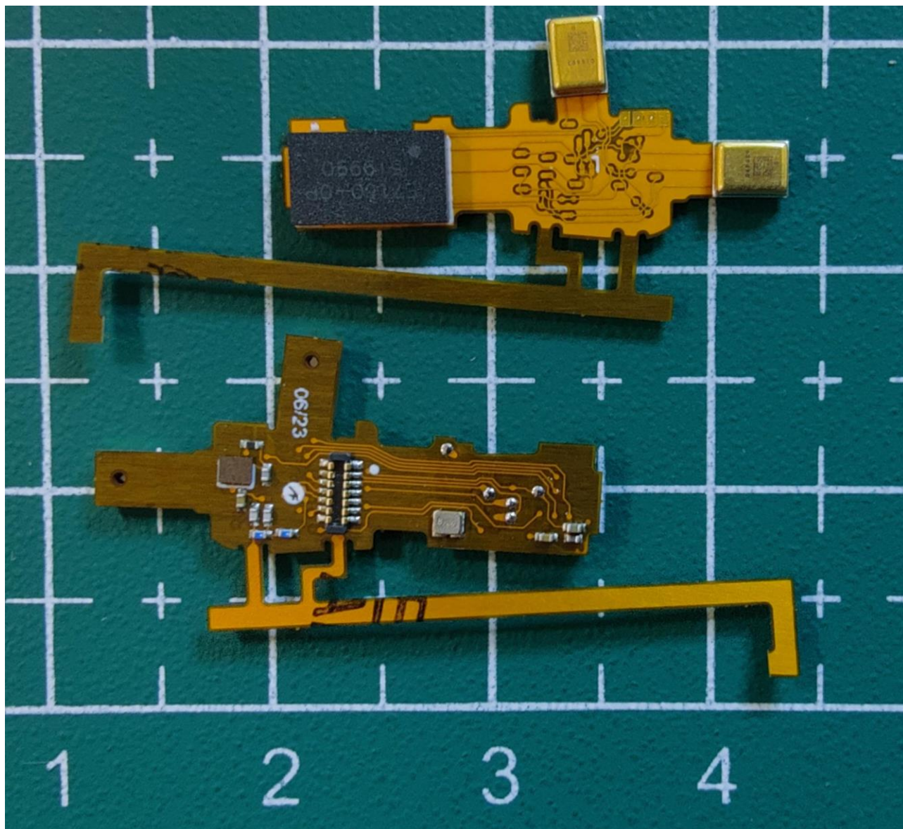
MAIN FLEX CIRCUIT (TOP AND BOTTOM) SHOWING ANTENNA
