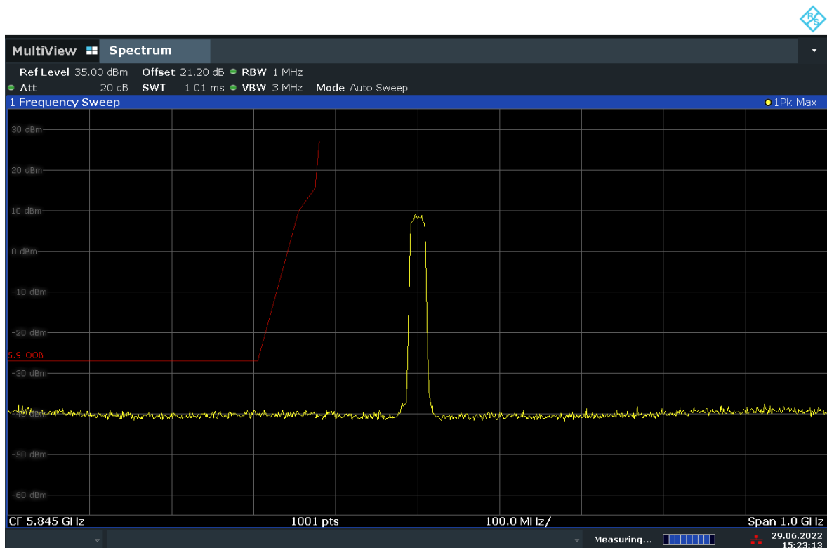
Fig. 25 Out of Band Emission - Conducted (802.11n-HT20, Ch169)
