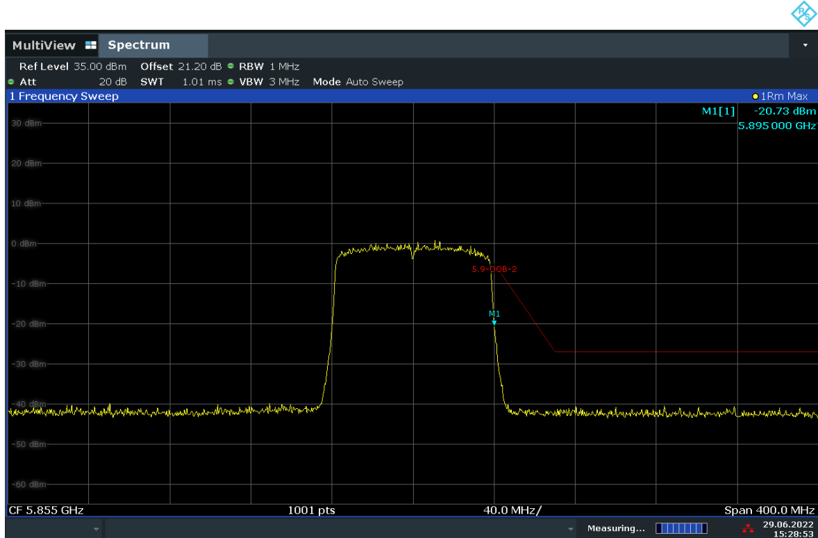
Fig. 47 Out of Band Emission - Conducted (802.11ac-VHT80, Ch171)
