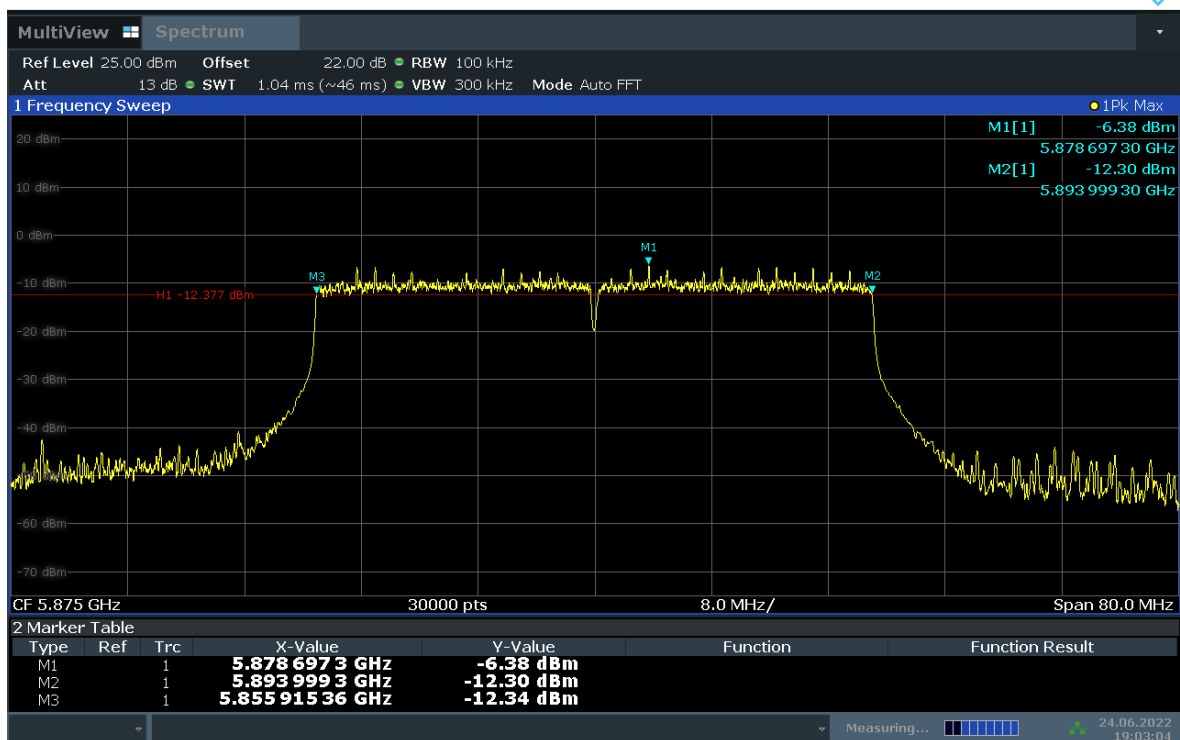
Fig. 8 Occupied 6dB Bandwidth (802.11ax-HE40, Ch 175)
