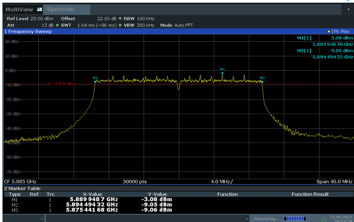
Fig. 6 Occupied 6dB Bandwidth (802.11ax-HE20, Ch 177)
