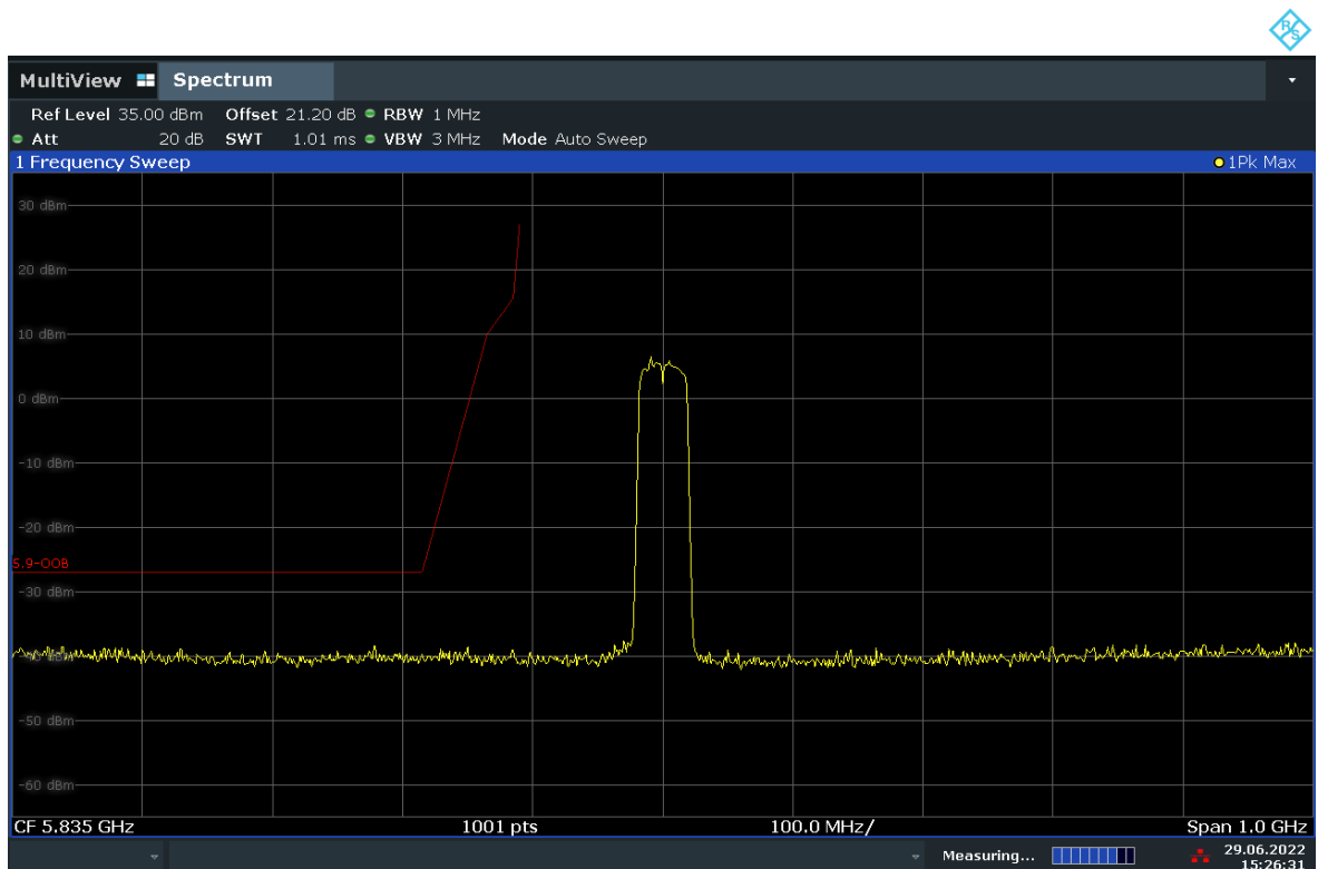
Fig. 29 Out of Band Emission - Conducted (802.11ac-VHT40, Ch167)
