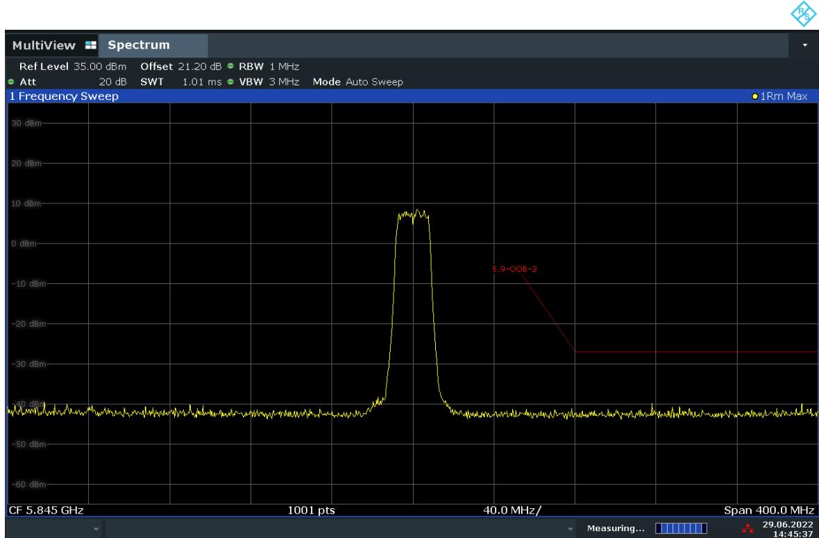
Fig. 49 Out of Band Emission - Conducted (802.11a, Ch169)
