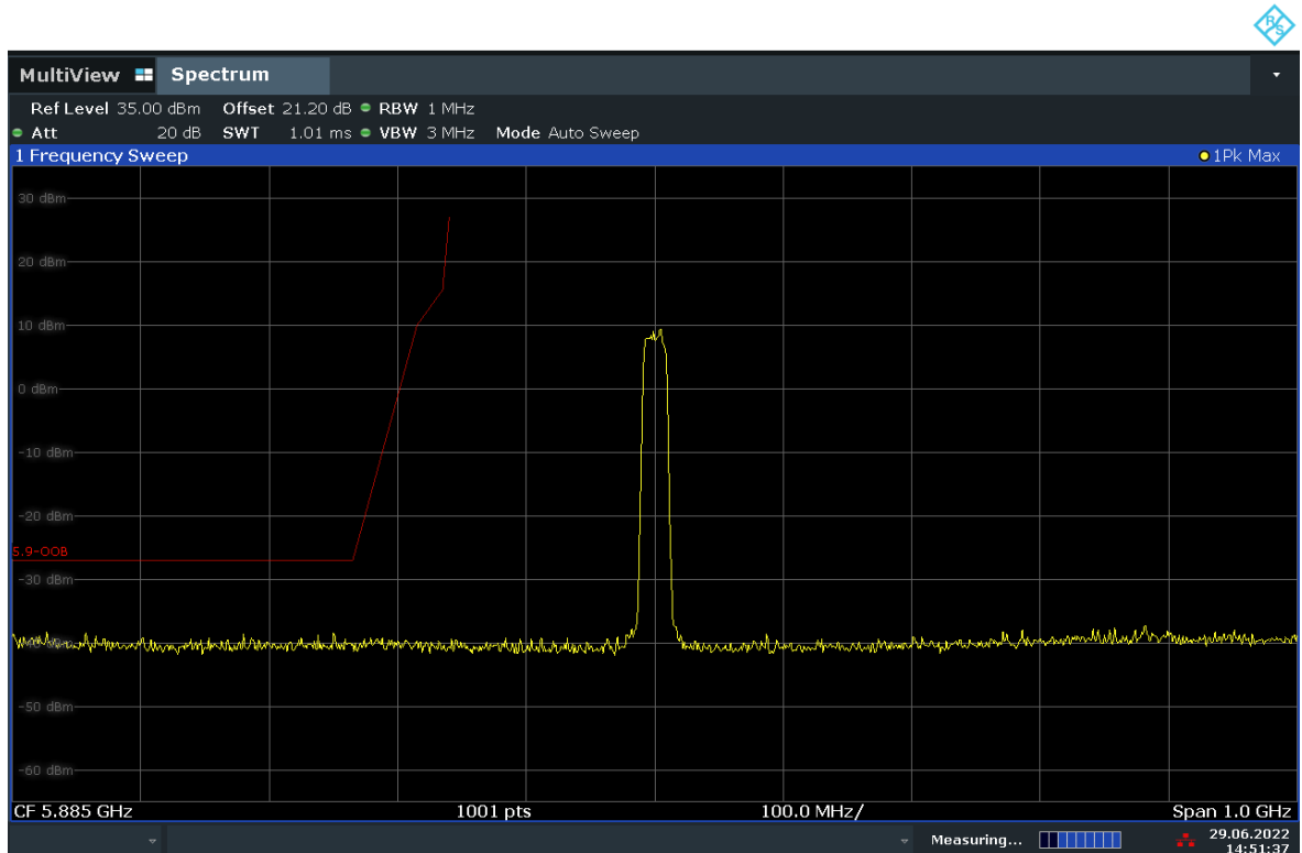
Fig. 54 Out of Band Emission - Conducted (802.11n-HT20, Ch169)
