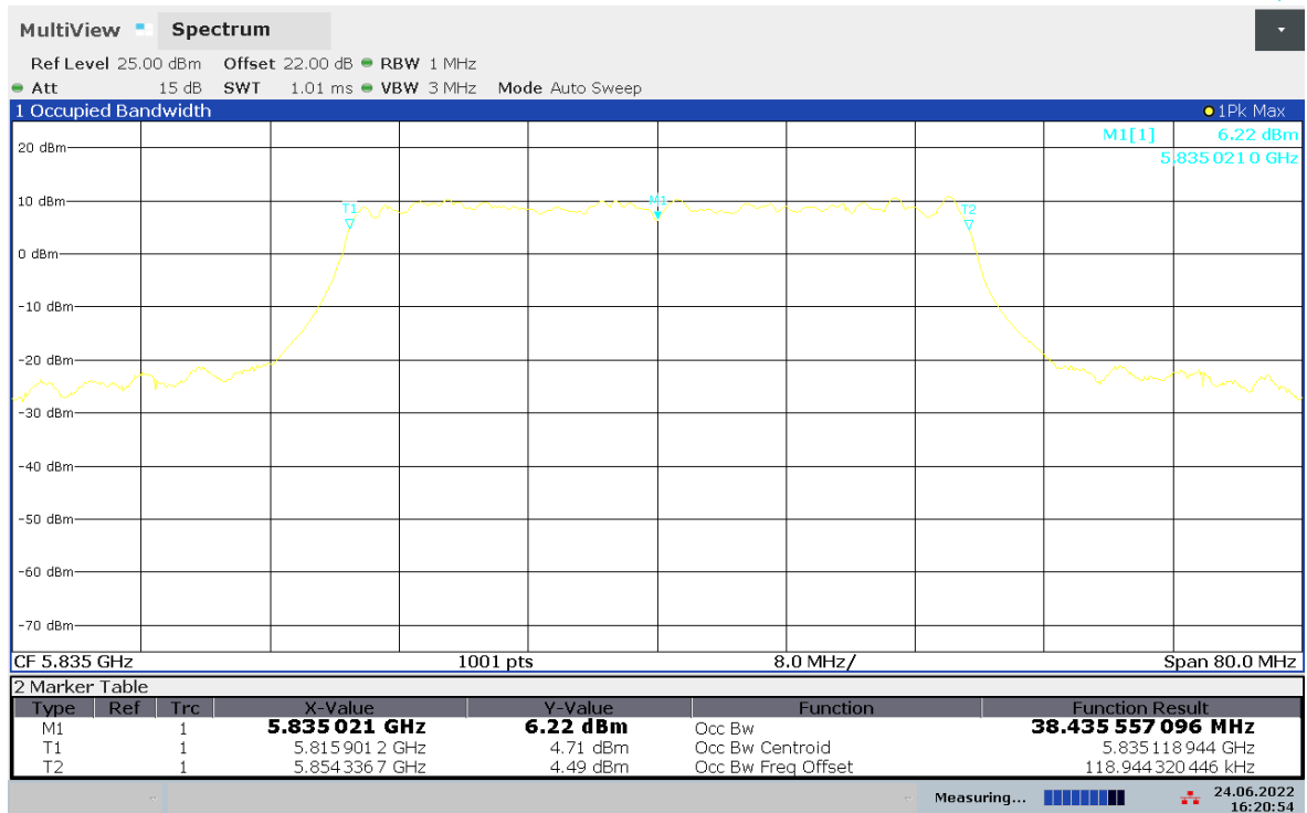
Fig. 17 99% Occupied Bandwidth (802.11ax-HE40, Ch 167)
