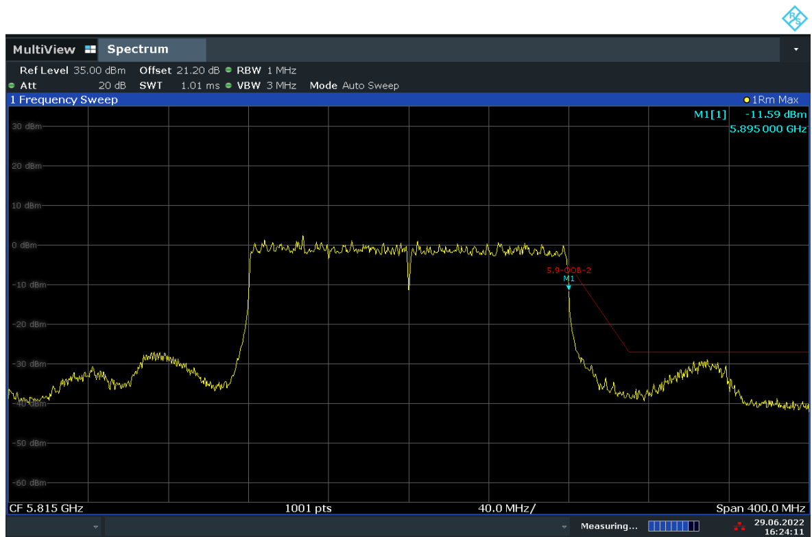
Fig. 46 Out of Band Emission - Conducted (802.11ax-HE160 full RU, Ch163)
