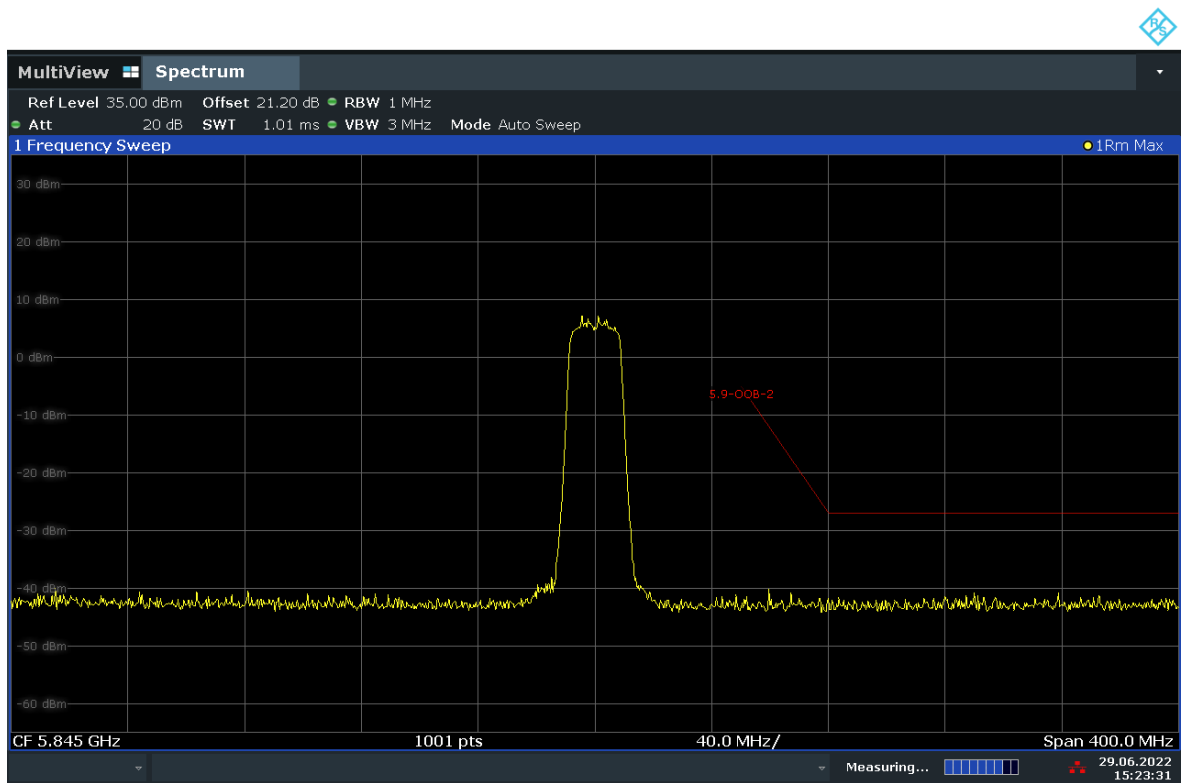
Fig. 26 Out of Band Emission - Conducted (802.11n-HT20, Ch169)
