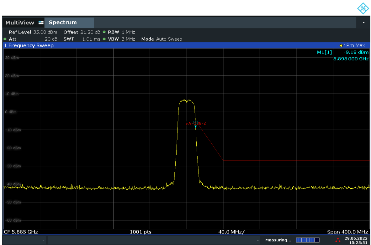
Fig. 28 Out of Band Emission - Conducted (802.11n-HT20, Ch177)
