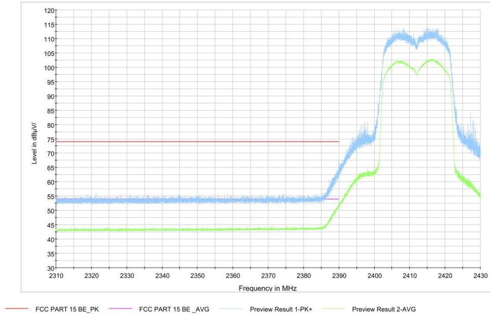
Fig.A.6.2.17 Transmitter Spurious Emission - Radiated (Power): 802.11ax-HT20, ch1, 2.31 GHz - 2.43GHz
