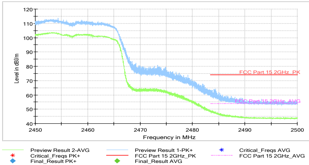
Fig.A.6.2.7 Transmitter Spurious Emission - Radiated (Power): 802.11n-HT20, ch10, 2.45 GHz - 2.50GHz
