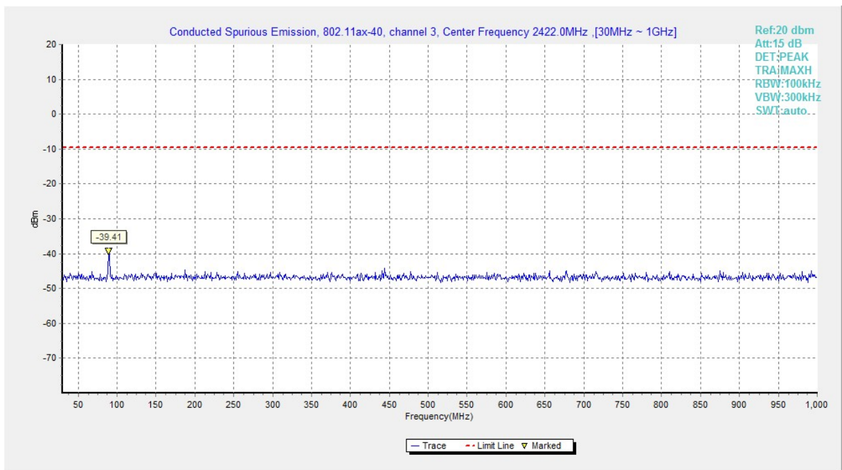
Fig.A.6.1.218 Transmitter Spurious Emission - Conducted (802.11ax-HE40, Ch3, 30 MHz-1 GHz)
