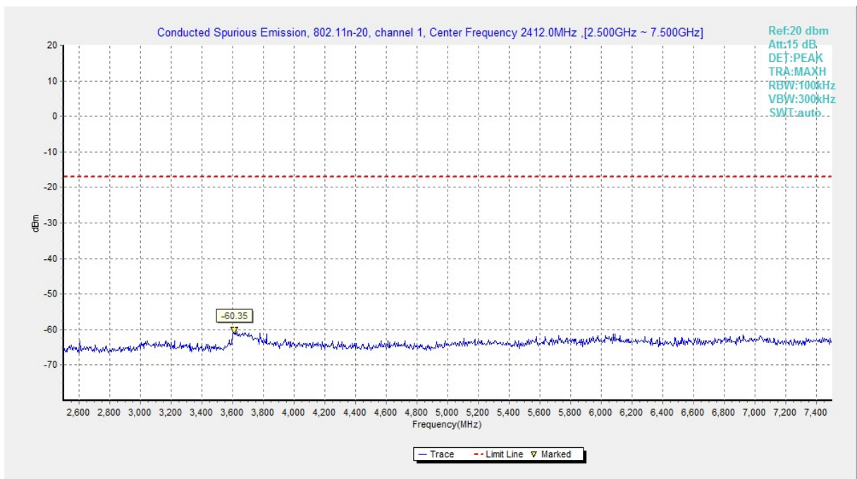
Fig.A.6.1.244 Transmitter Spurious Emission - Conducted (802.11n-HT20, Ch1, 2.5 GHz-7.5 GHz)
