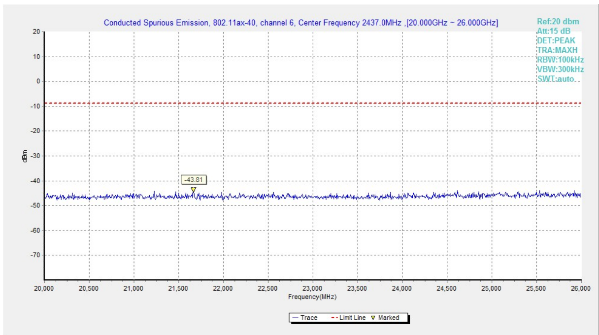
Fig.A.6.1.232 Transmitter Spurious Emission - Conducted (802.11ax-HE40, Ch6, 20 GHz-26 GHz)
