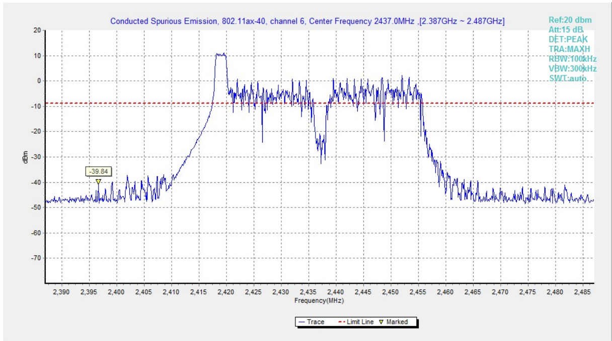
Fig.A.6.1.225 Transmitter Spurious Emission - Conducted (802.11ax-HE40, Ch6, Center Frequency)
