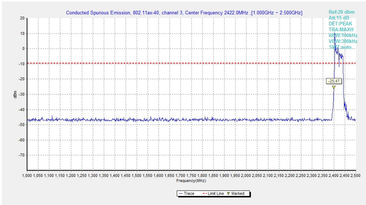
Fig.A.6.1.219 Transmitter Spurious Emission - Conducted (802.11ax-HE40, Ch3, 1 GHz-2.5 GHz)
