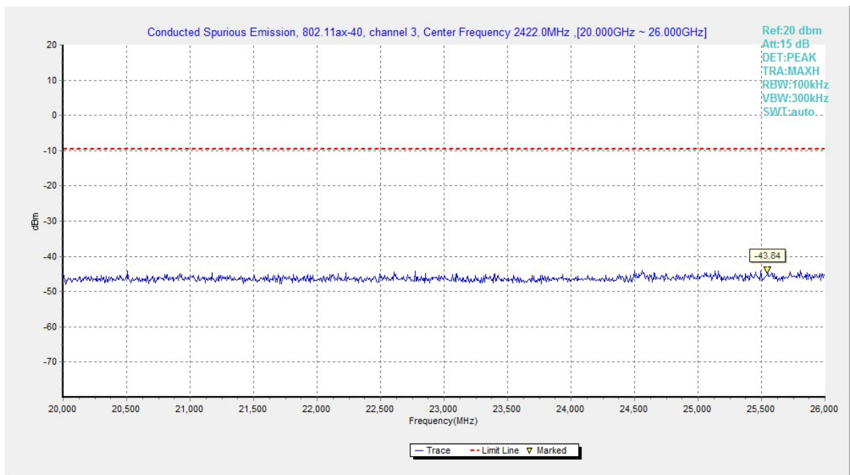
Fig.A.6.1.224 Transmitter Spurious Emission - Conducted (802.11ax-HE40, Ch3, 20 GHz-26 GHz)
