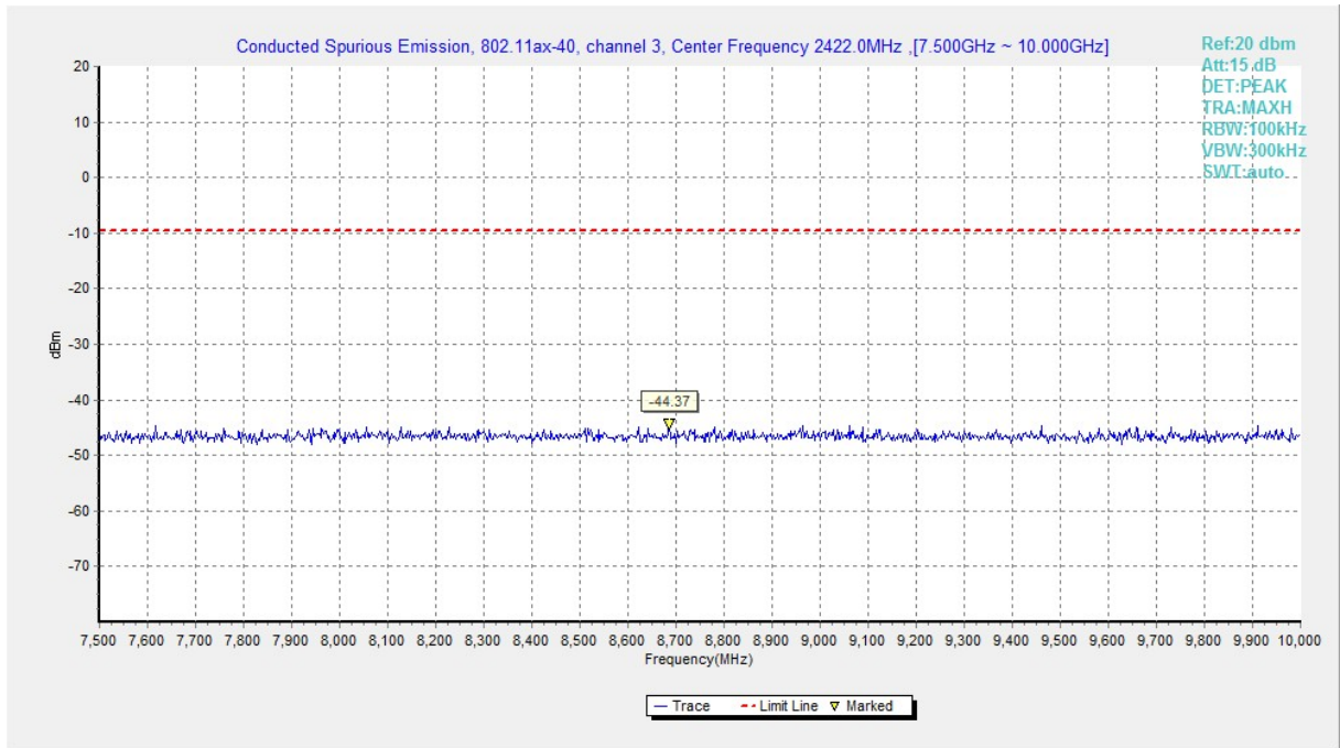
Fig.A.6.1.221 Transmitter Spurious Emission - Conducted (802.11ax-HE40, Ch3, 7.5 GHz-10 GHz)
