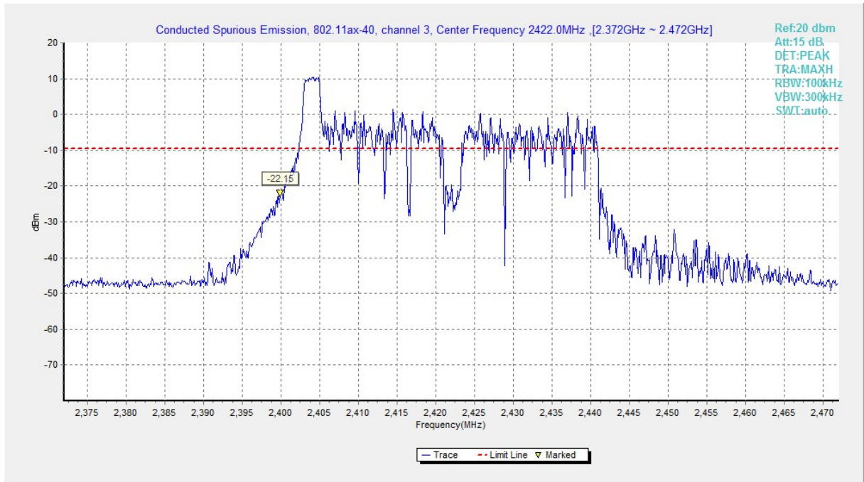
Fig.A.6.1.217 Transmitter Spurious Emission - Conducted (802.11ax-HE40, Ch3, Center Frequency)
