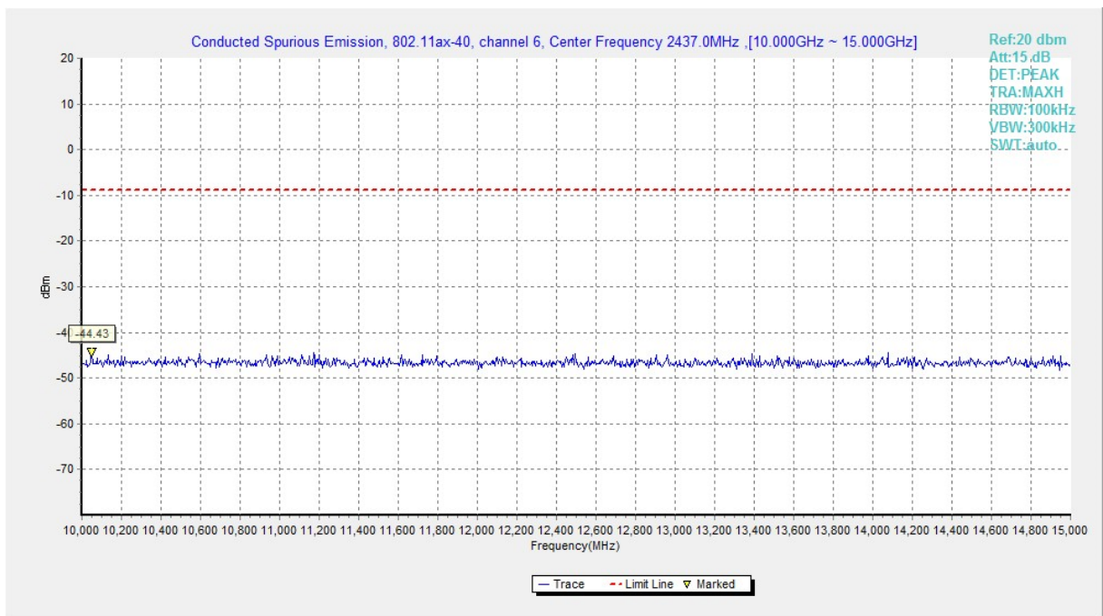
Fig.A.6.1.230 Transmitter Spurious Emission - Conducted (802.11ax-HE40, Ch6, 10 GHz-15 GHz)
