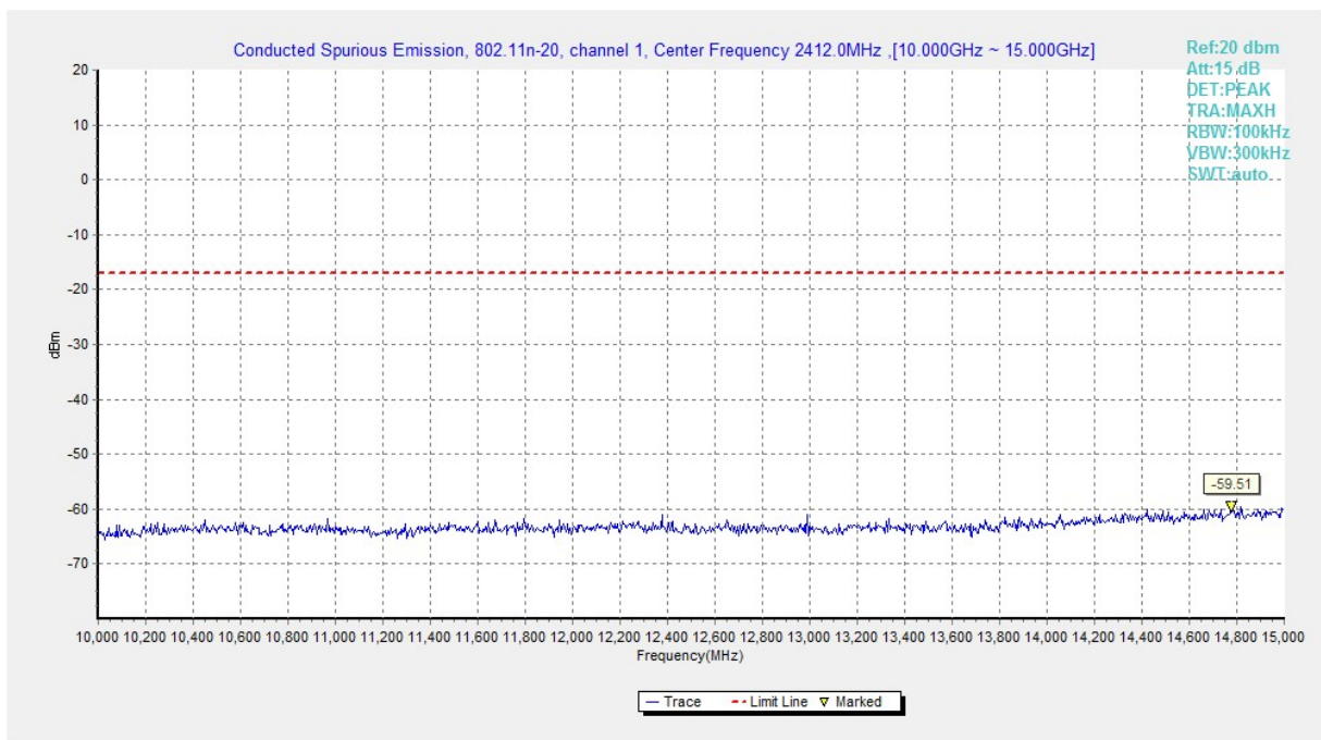
Fig.A.6.1.246 Transmitter Spurious Emission - Conducted (802.11n-HT20, Ch1, 10 GHz-15 GHz)
