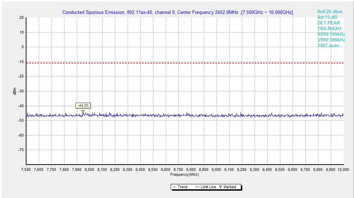
Fig.A.6.1.237 Transmitter Spurious Emission - Conducted (802.11ax-HE40, Ch9, 7.5 GHz-10 GHz)
