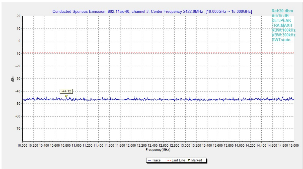
Fig.A.6.1.222 Transmitter Spurious Emission - Conducted (802.11ax-HE40, Ch3, 10 GHz-15 GHz)
