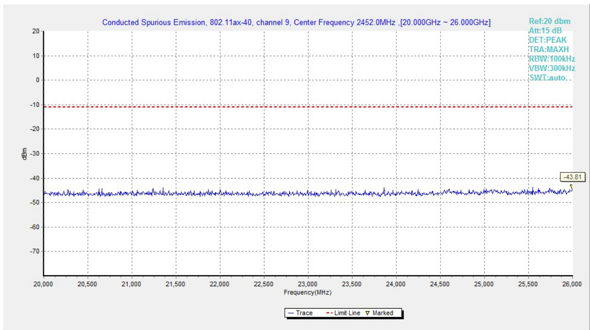
Fig.A.6.1.240 Transmitter Spurious Emission - Conducted (802.11ax-HE40, Ch9, 20 GHz-26 GHz)
