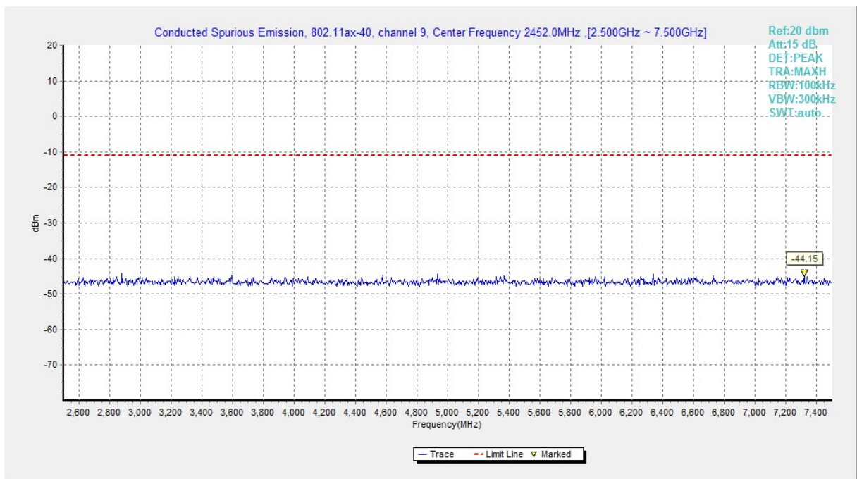
Fig.A.6.1.236 Transmitter Spurious Emission - Conducted (802.11ax-HE40, Ch9, 2.5 GHz-7.5 GHz)
