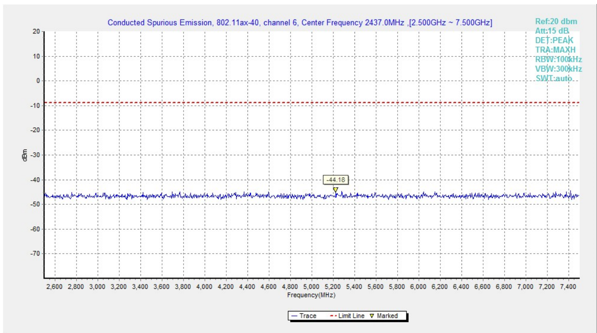
Fig.A.6.1.228 Transmitter Spurious Emission - Conducted (802.11ax-HE40, Ch6, 2.5 GHz-7.5 GHz)
