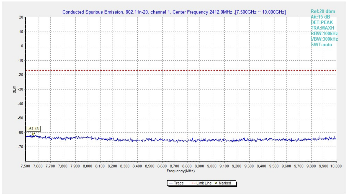
Fig.A.6.1.245 Transmitter Spurious Emission - Conducted (802.11n-HT20, Ch1, 7.5 GHz-10 GHz)
