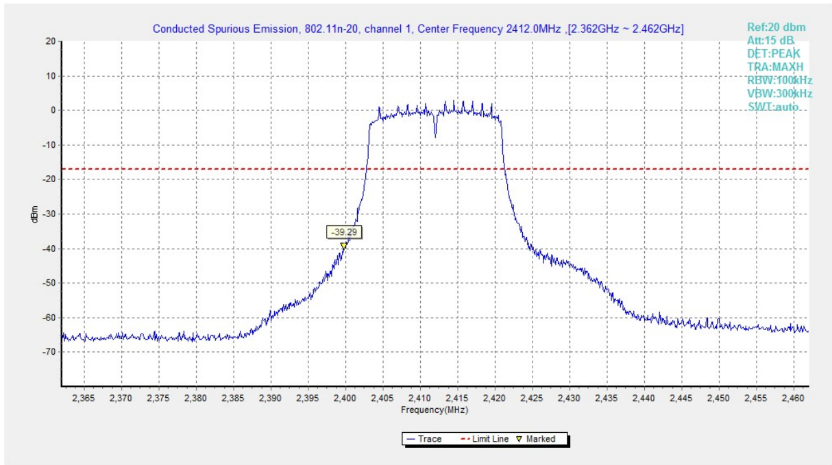
Fig.A.6.1.241 Transmitter Spurious Emission - Conducted (802.11n-HT20, Ch1, Center Frequency)
