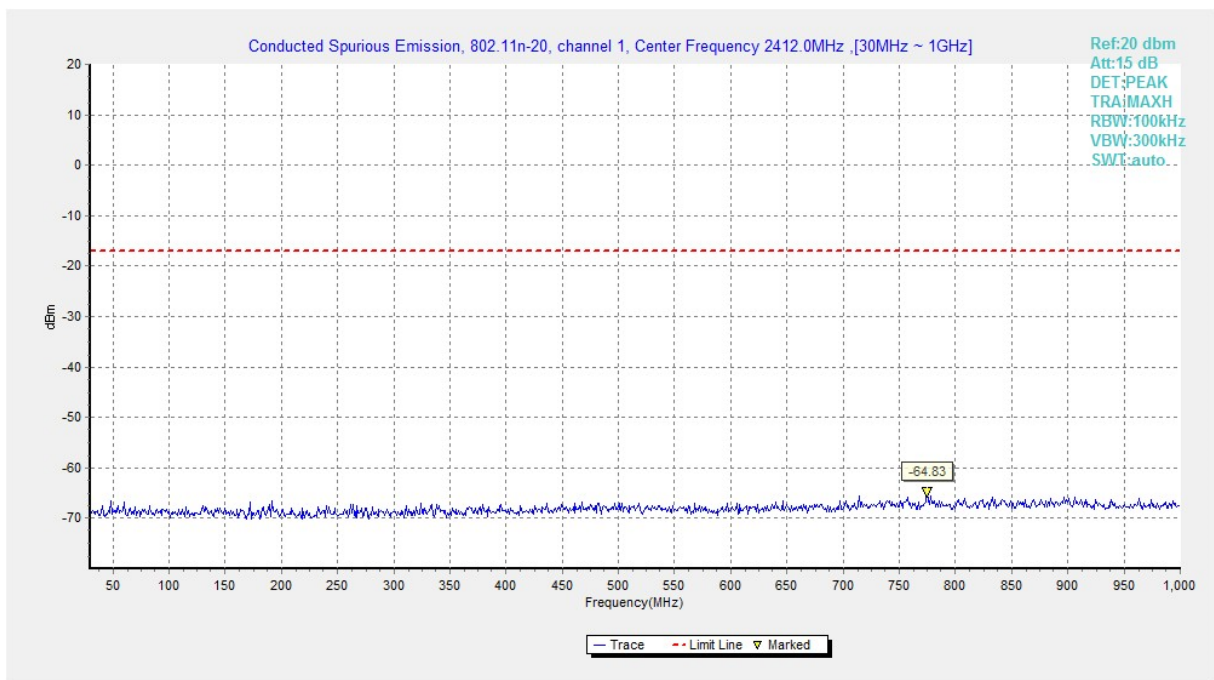
Fig.A.6.1.242 Transmitter Spurious Emission - Conducted (802.11n-HT20, Ch1, 30 MHz-1 GHz)
