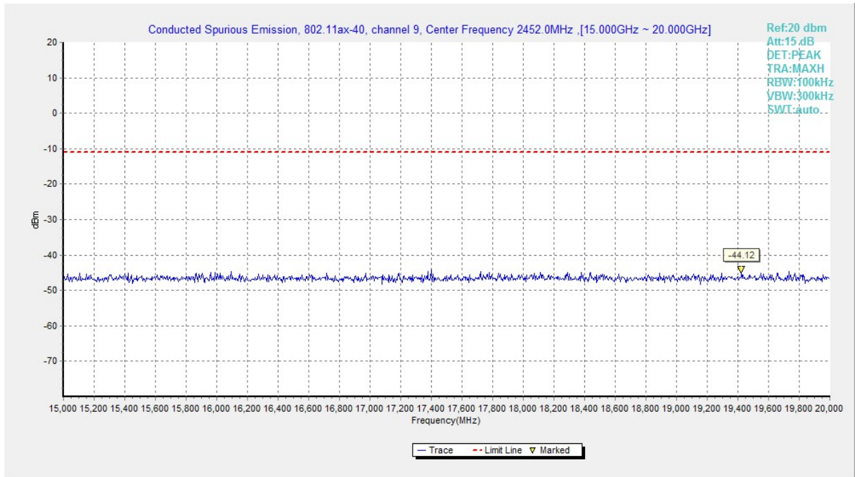
Fig.A.6.1.239 Transmitter Spurious Emission - Conducted (802.11ax-HE40, Ch9, 15 GHz-20 GHz)
