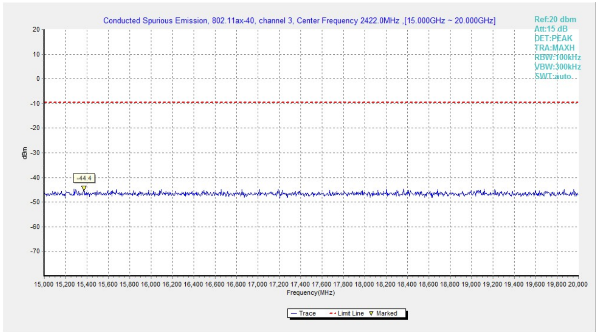
Fig.A.6.1.223 Transmitter Spurious Emission - Conducted (802.11ax-HE40, Ch3, 15 GHz-20 GHz)
