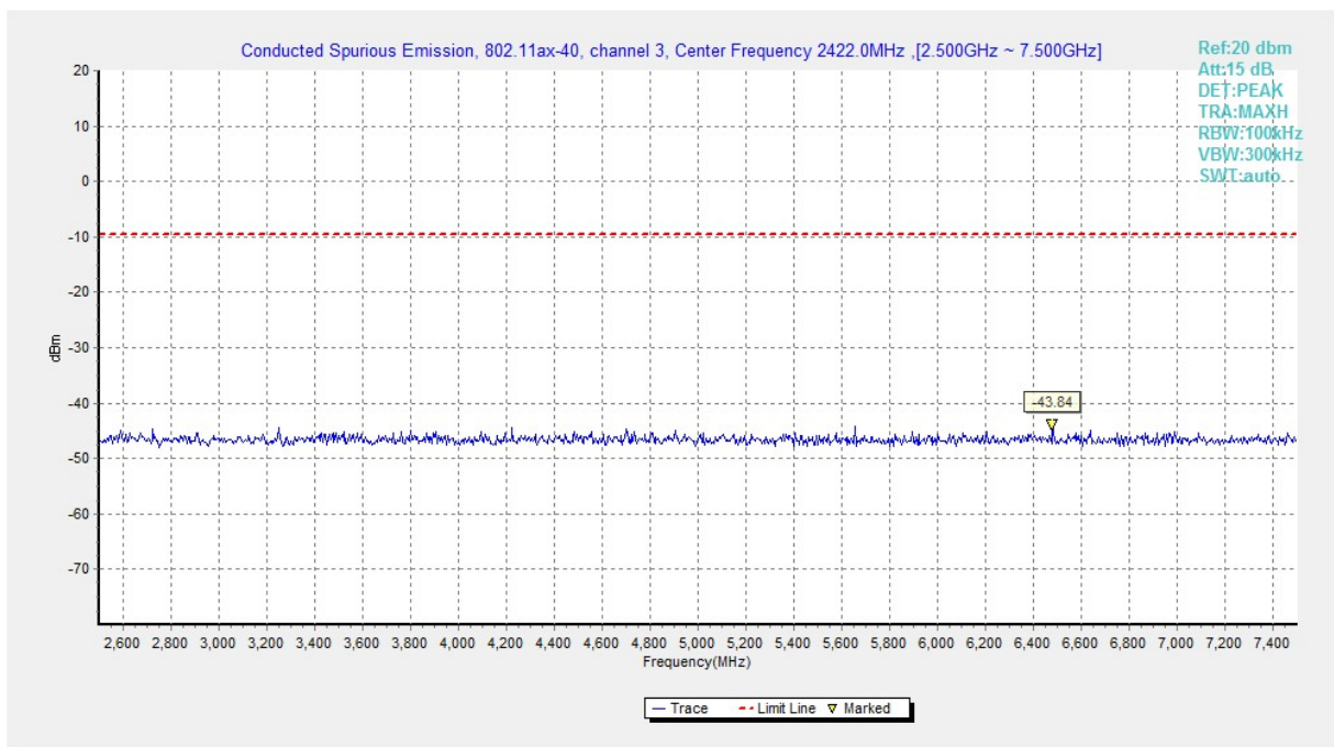
Fig.A.6.1.220 Transmitter Spurious Emission - Conducted (802.11ax-HE40, Ch3, 2.5 GHz-7.5 GHz)
