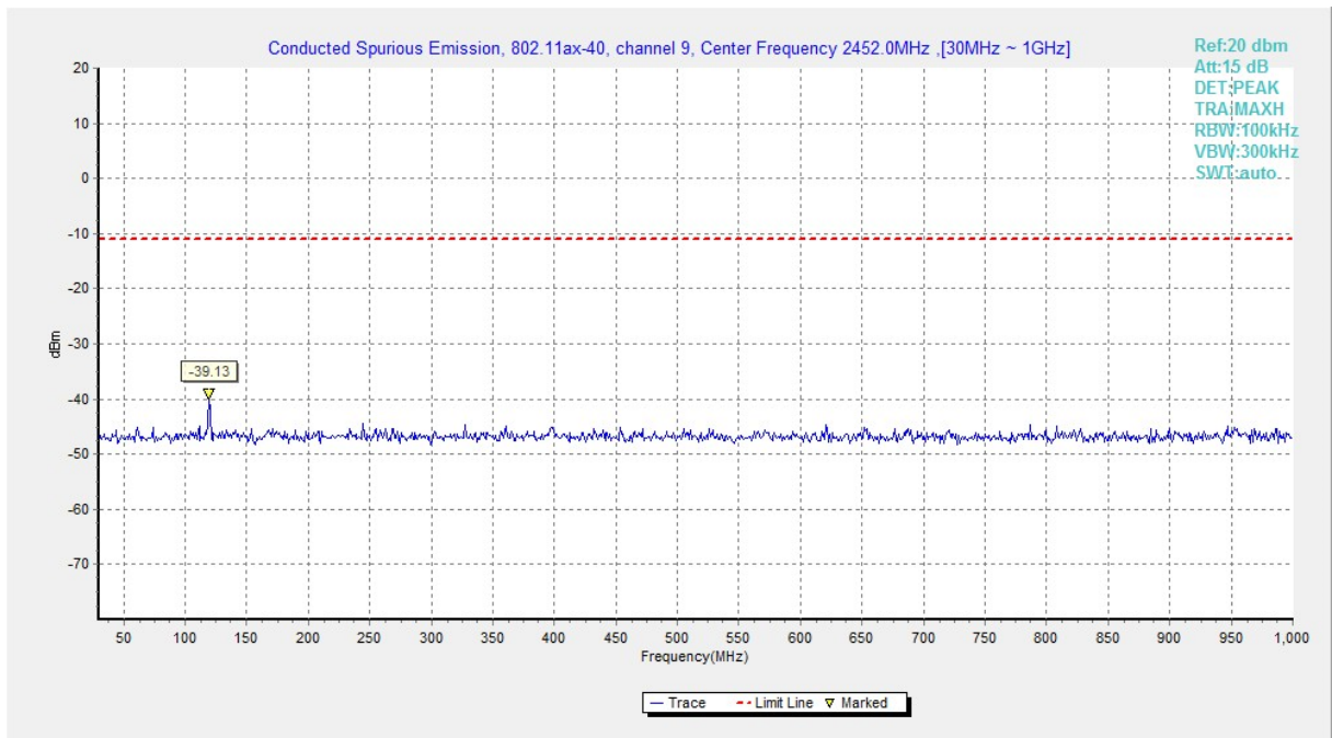
Fig.A.6.1.234 Transmitter Spurious Emission - Conducted (802.11ax-HE40, Ch9, 30 MHz-1 GHz)
