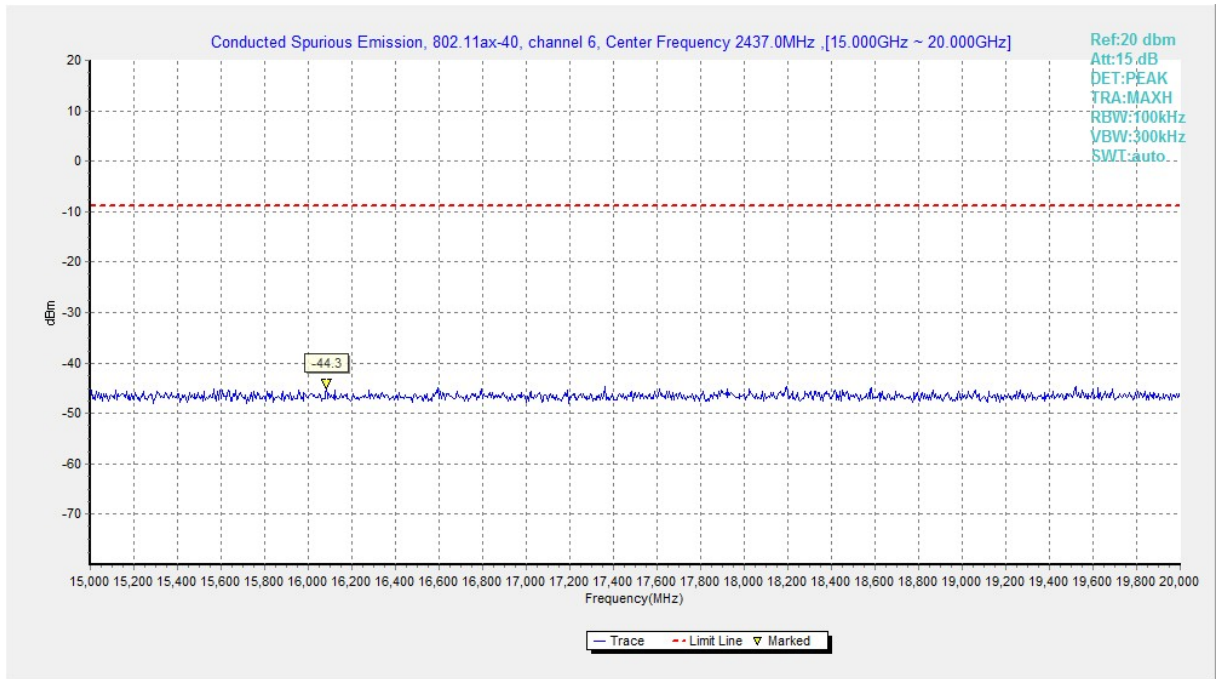
Fig.A.6.1.231 Transmitter Spurious Emission - Conducted (802.11ax-HE40, Ch6, 15 GHz-20 GHz)
