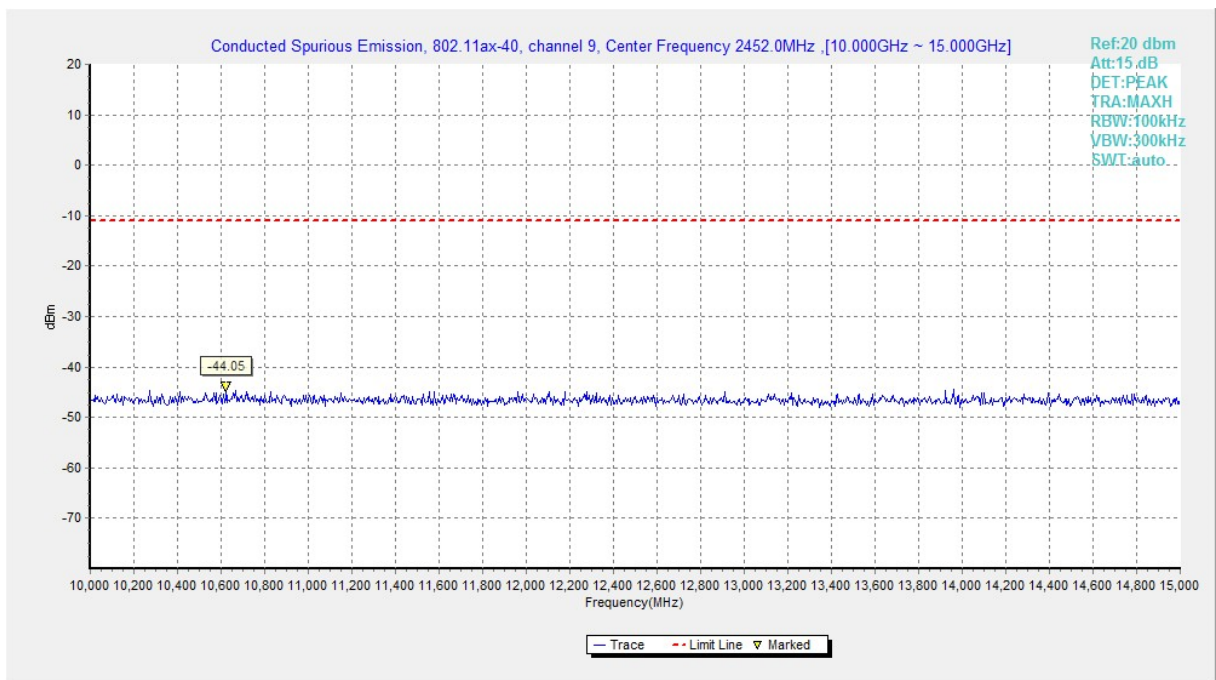
Fig.A.6.1.238 Transmitter Spurious Emission - Conducted (802.11ax-HE40, Ch9, 10 GHz-15 GHz)
