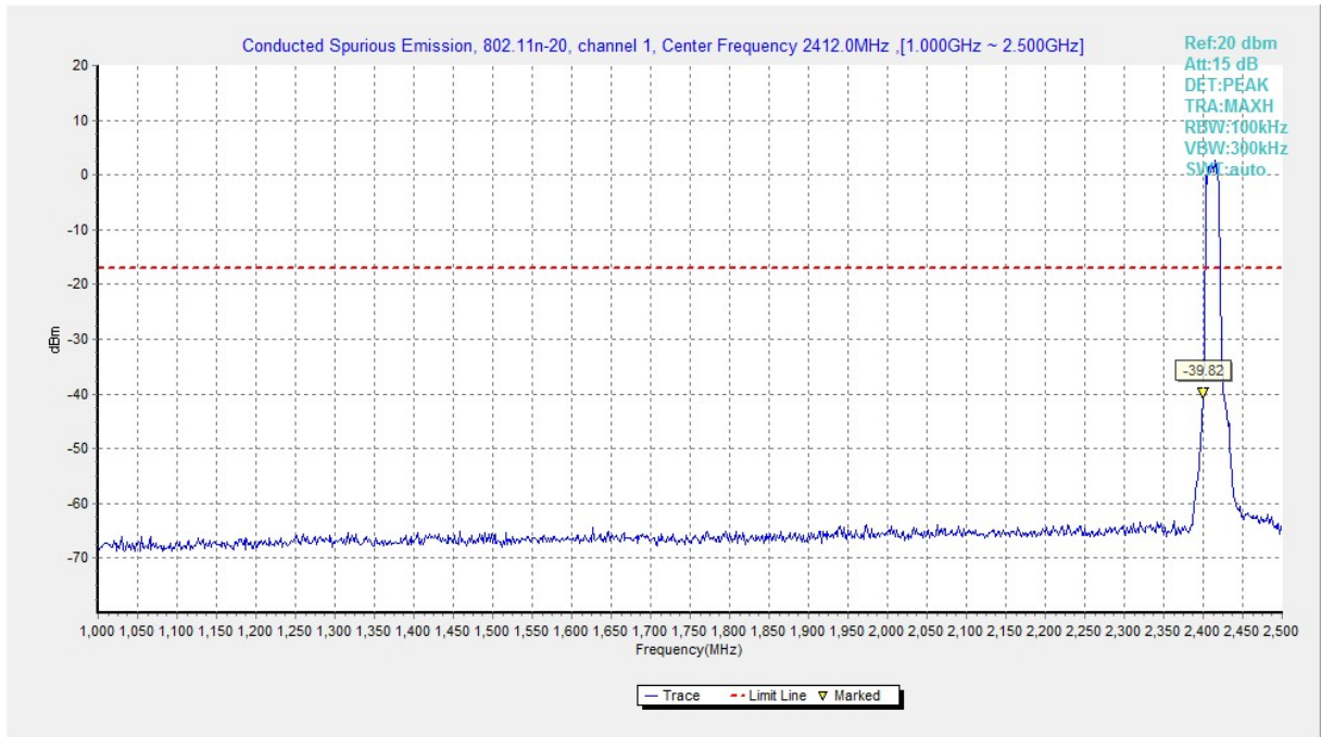
Fig.A.6.1.243 Transmitter Spurious Emission - Conducted (802.11n-HT20, Ch1, 1 GHz-2.5 GHz)
