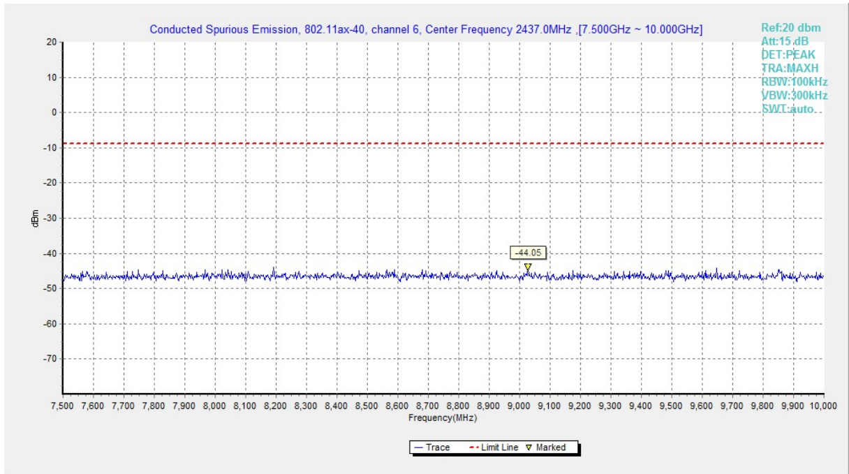
Fig.A.6.1.229 Transmitter Spurious Emission - Conducted (802.11ax-HE40, Ch6, 7.5 GHz-10 GHz)
