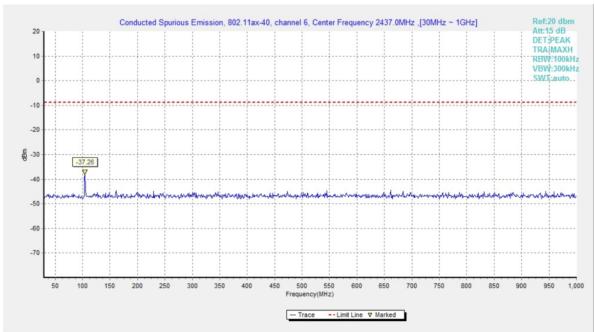
Fig.A.6.1.226 Transmitter Spurious Emission - Conducted (802.11ax-HE40, Ch6, 30 MHz-1 GHz)
