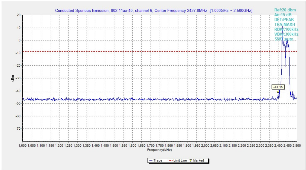
Fig.A.6.1.227 Transmitter Spurious Emission - Conducted (802.11ax-HE40, Ch6, 1 GHz-2.5 GHz)
