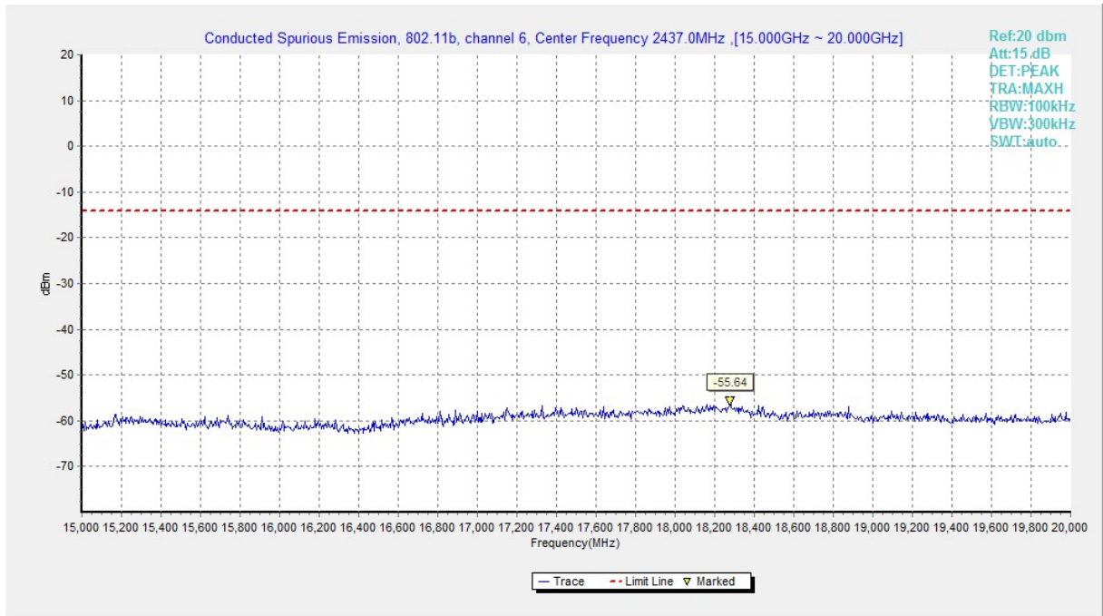
Fig.A.6.1.159 Transmitter Spurious Emission - Conducted (802.11b, Ch6, 15 GHz-20 GHz)
