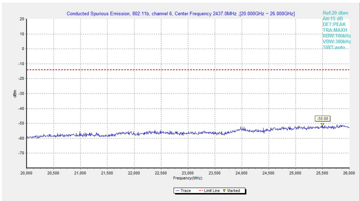
Fig.A.6.1.160 Transmitter Spurious Emission - Conducted (802.11b, Ch6, 20 GHz-26 GHz)
