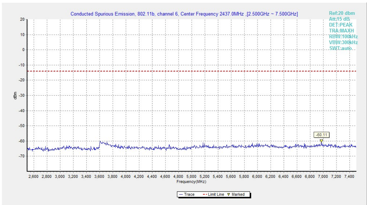
Fig.A.6.1.156 Transmitter Spurious Emission - Conducted (802.11b, Ch6, 2.5 GHz-7.5 GHz)
