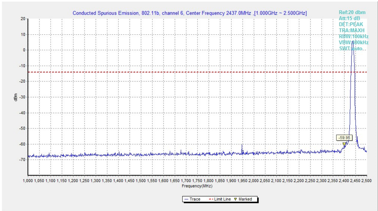
Fig.A.6.1.155 Transmitter Spurious Emission - Conducted (802.11b, Ch6, 1 GHz-2.5 GHz)
