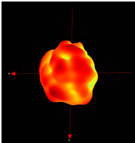
ANT4_6E(Frequency=6800MHz)
