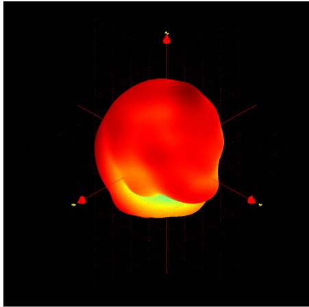
ANT4_5G(Frequency=5500MHz)
