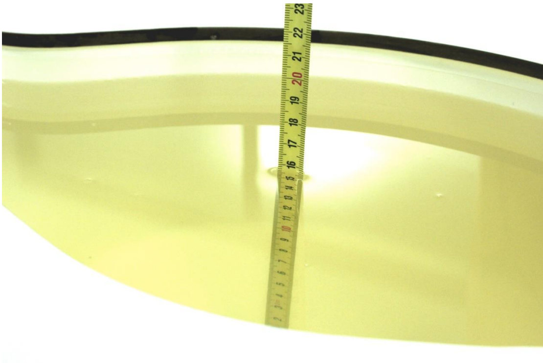
Picture 8-6 Liquid depth in the Head Phantom (2600 MHz)
