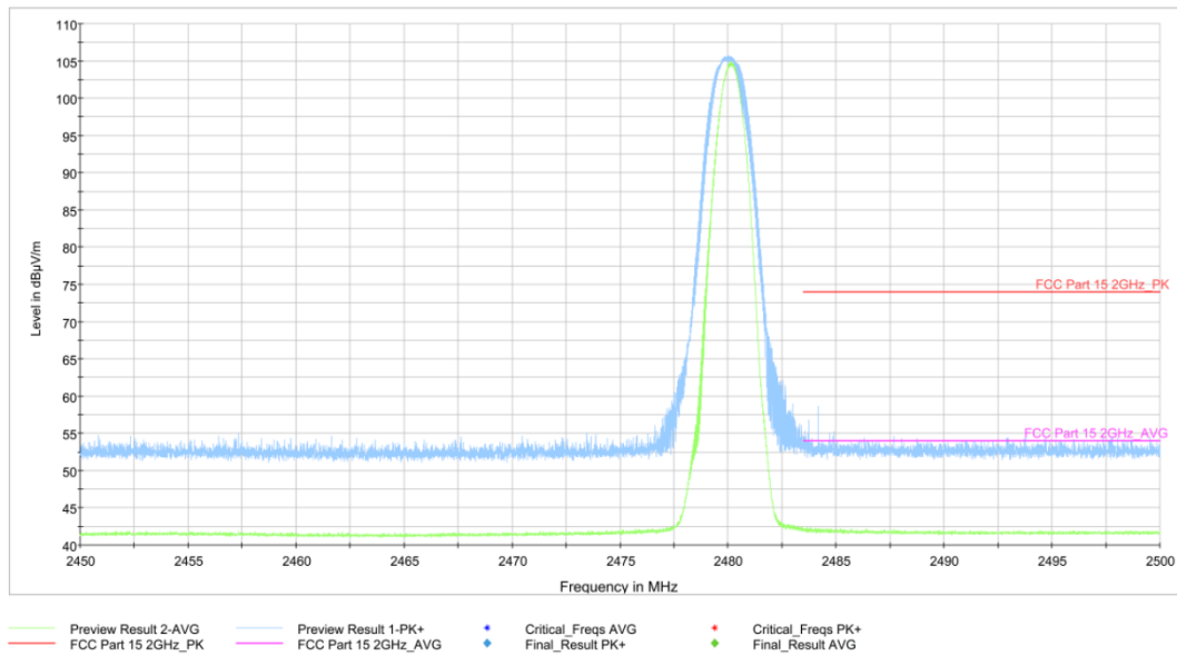
Fig.16. Frequency Band Edges: \pi/4 DQPSK, Channel 78, Hopping Off, 2.45 GHz - 2.50GHz
