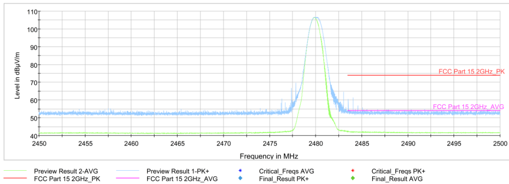
Fig.14. Frequency Band Edges: GFSK, Channel 78, Hopping Off, ch11, 2.45 GHz - 2.50GHz
