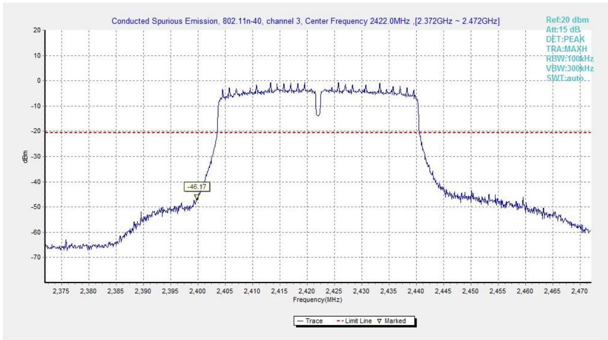
Fig.A.6.1.265 Transmitter Spurious Emission - Conducted (802.11n-HT40, Ch3, Center Frequency)
