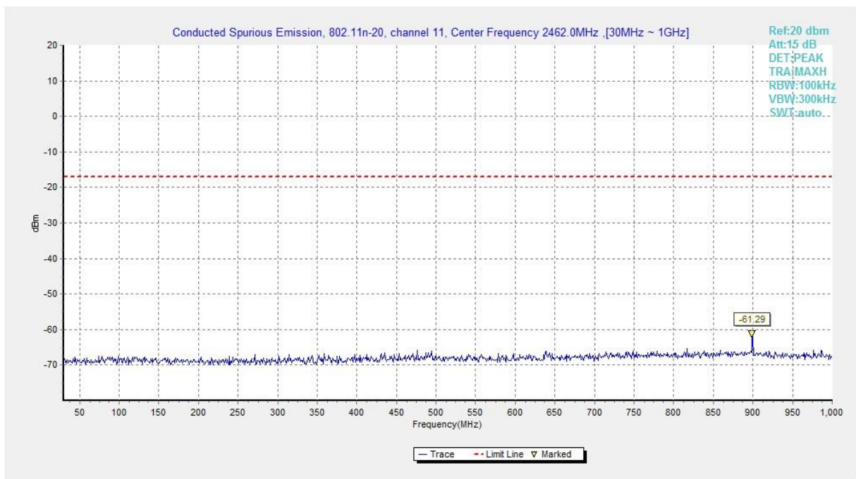
Fig.A.6.1.258 Transmitter Spurious Emission - Conducted (802.11n-HT20, Ch11, 30 MHz-1 GHz)
