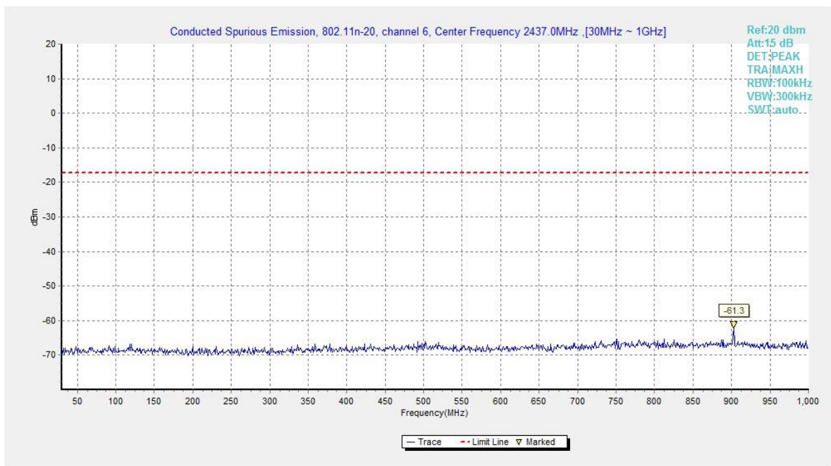
Fig.A.6.1.250 Transmitter Spurious Emission - Conducted (802.11n-HT20, Ch6, 30 MHz-1 GHz)
