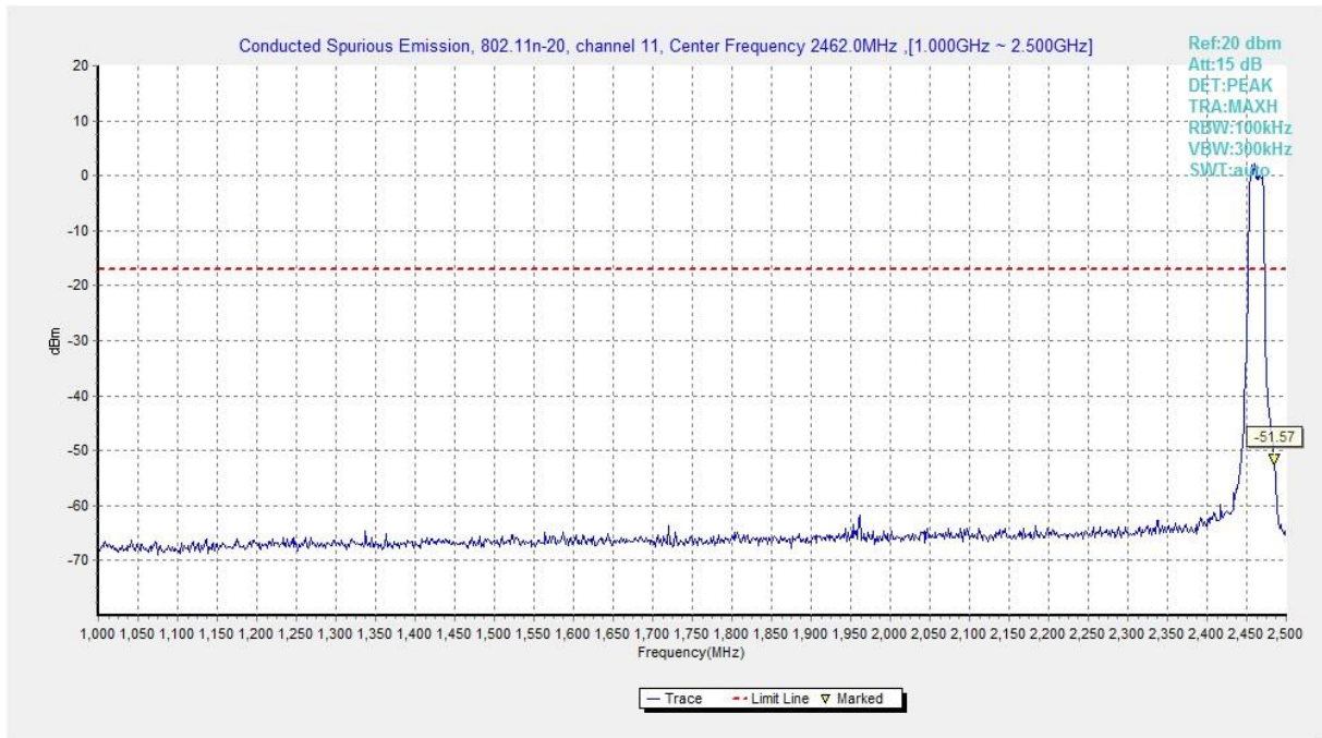
Fig.A.6.1.259 Transmitter Spurious Emission - Conducted (802.11n-HT20, Ch11, 1 GHz-2.5 GHz)
