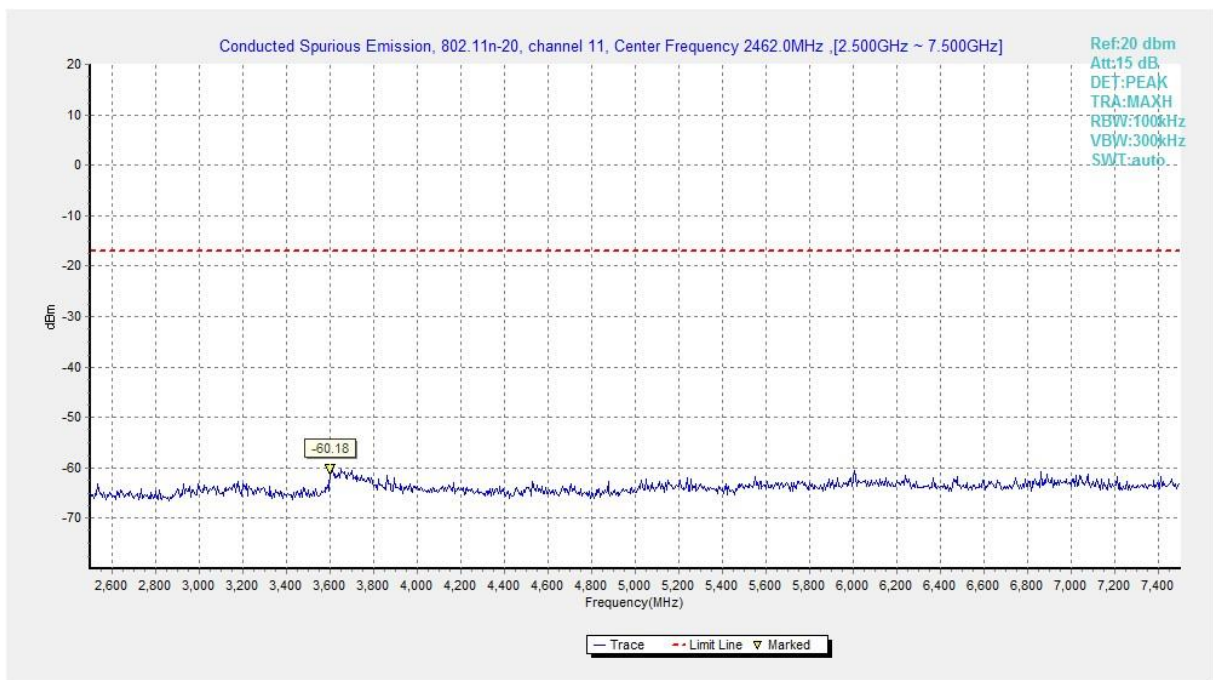
Fig.A.6.1.260 Transmitter Spurious Emission - Conducted (802.11n-HT20, Ch11, 2.5 GHz-7.5 GHz)
