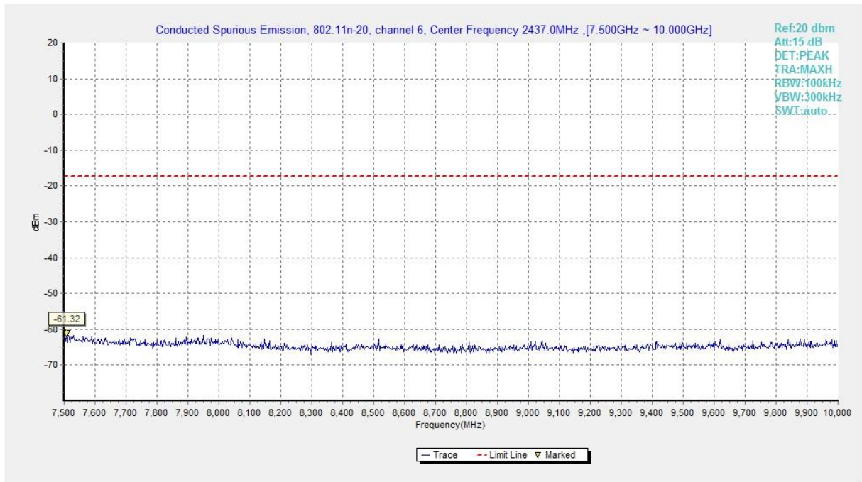
Fig.A.6.1.253 Transmitter Spurious Emission - Conducted (802.11n-HT20, Ch6, 7.5 GHz-10 GHz)
