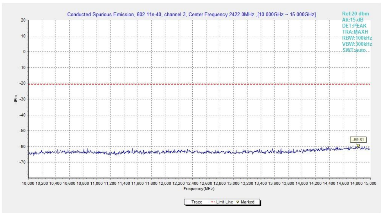
Fig.A.6.1.270 Transmitter Spurious Emission - Conducted (802.11n-HT40, Ch3, 10 GHz-15 GHz)
