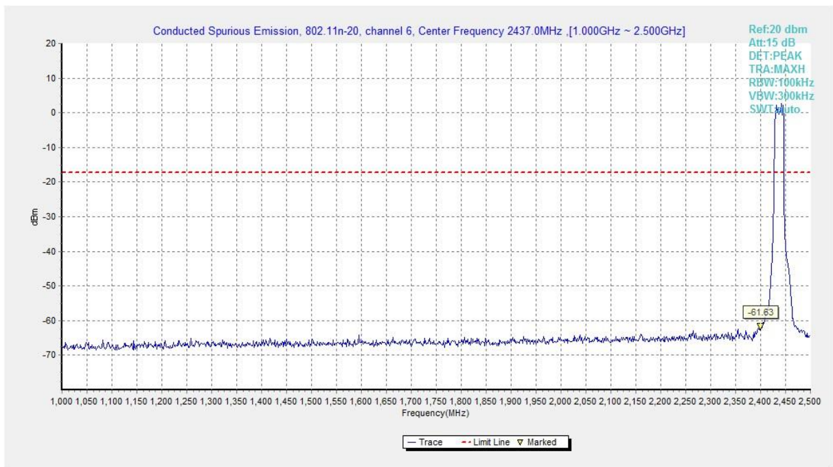
Fig.A.6.1.251 Transmitter Spurious Emission - Conducted (802.11n-HT20, Ch6, 1 GHz-2.5 GHz)
