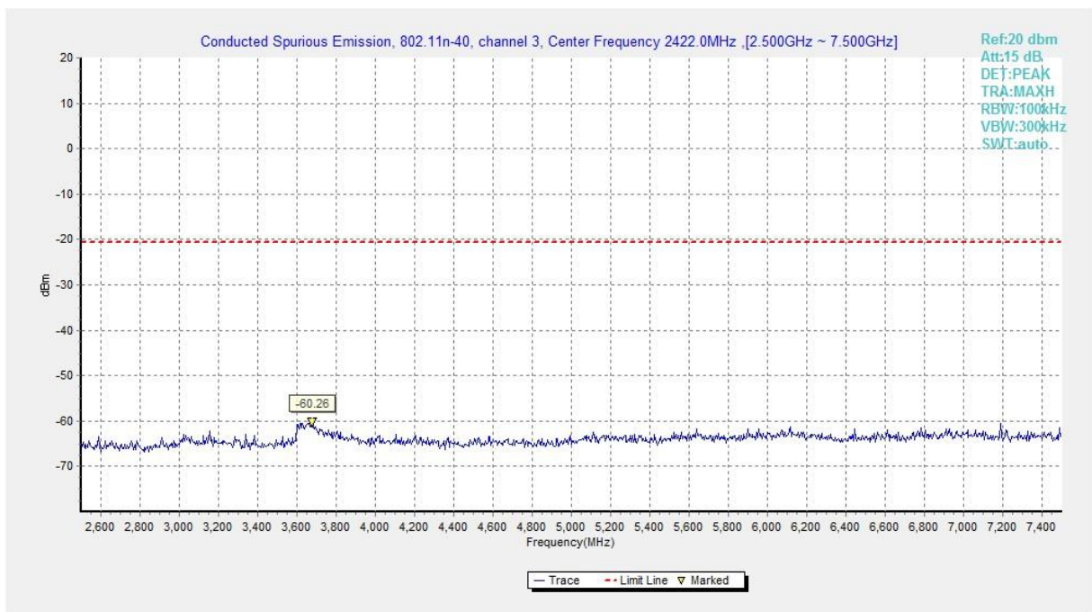
Fig.A.6.1.268 Transmitter Spurious Emission - Conducted (802.11n-HT40, Ch3, 2.5 GHz-7.5 GHz)
