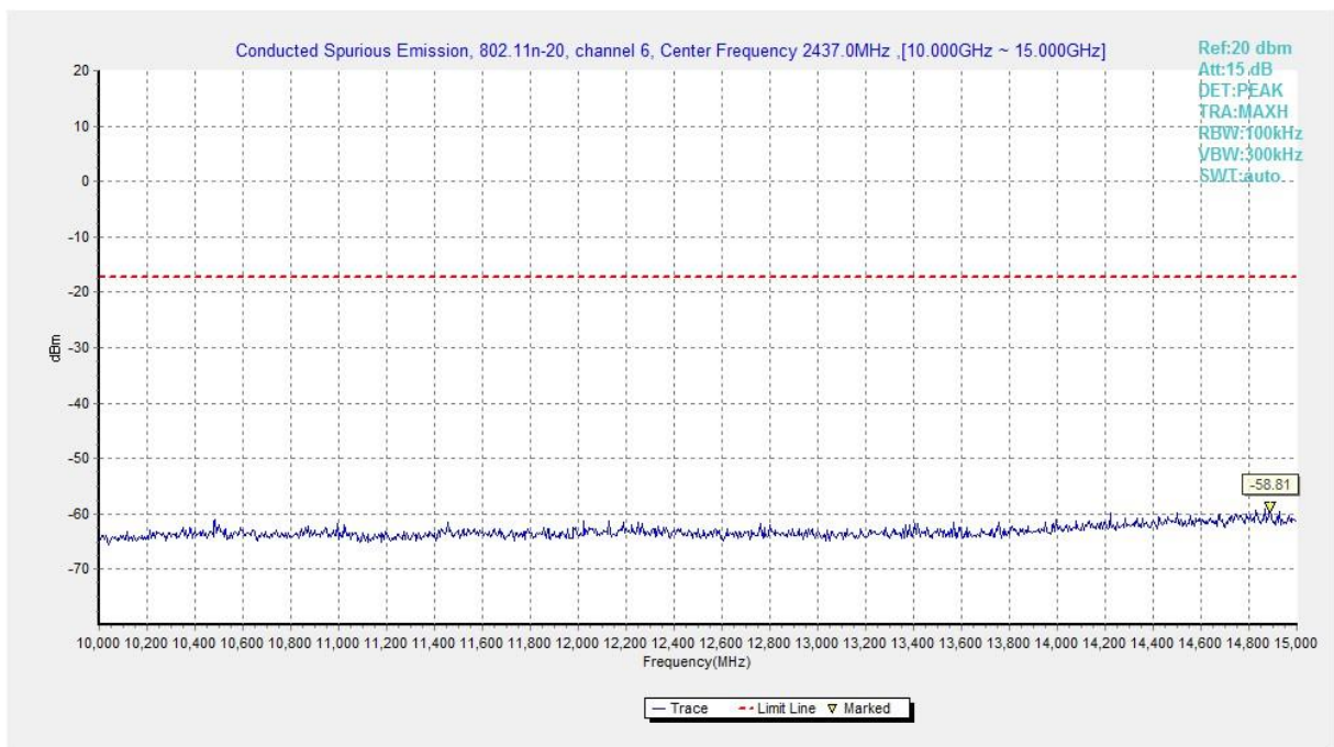
Fig.A.6.1.254 Transmitter Spurious Emission - Conducted (802.11n-HT20, Ch6, 10 GHz-15 GHz)
