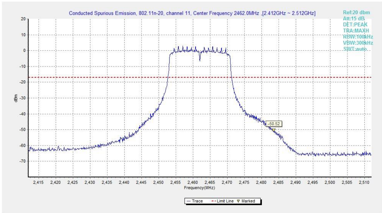
Fig.A.6.1.257 Transmitter Spurious Emission - Conducted (802.11n-HT20, Ch11, Center Frequency)
