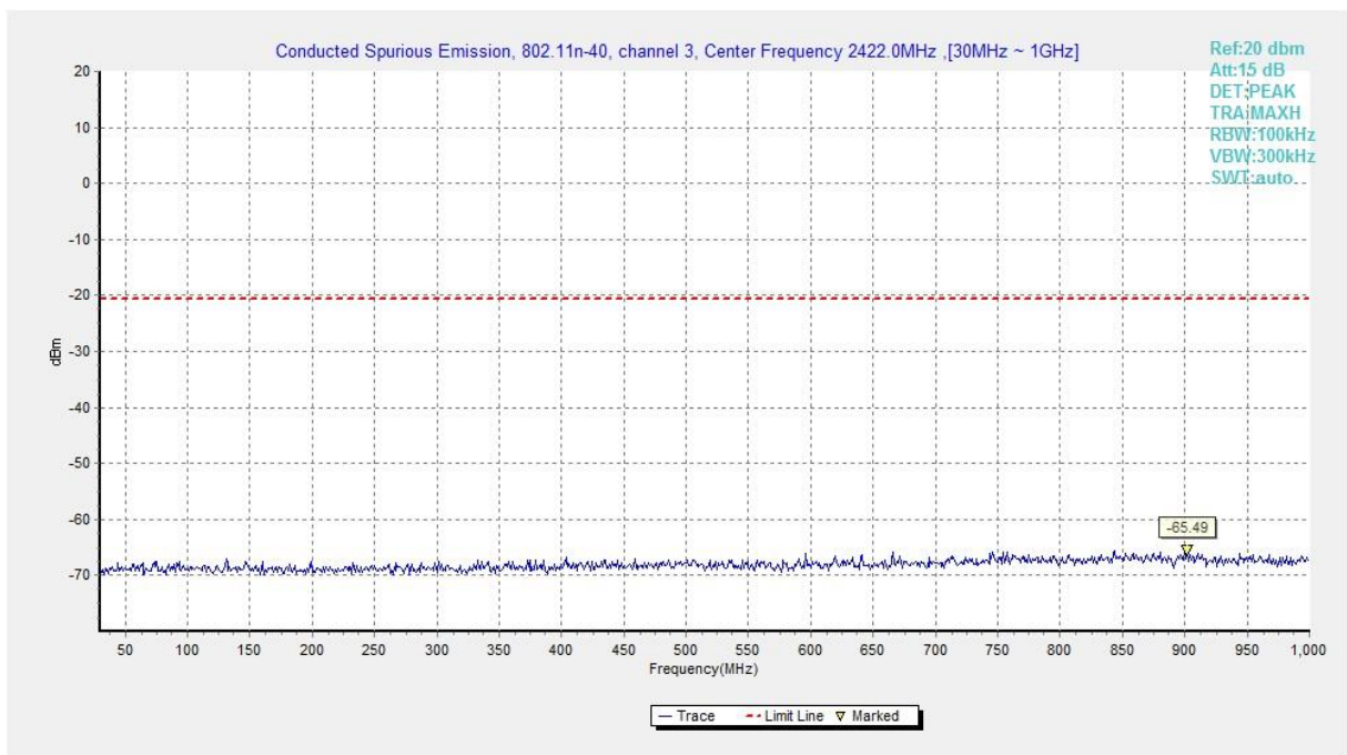
Fig.A.6.1.266 Transmitter Spurious Emission - Conducted (802.11n-HT40, Ch3, 30 MHz-1 GHz)
