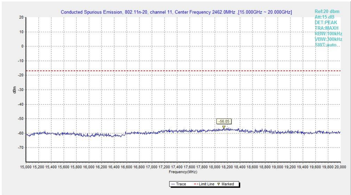
Fig.A.6.1.263 Transmitter Spurious Emission - Conducted (802.11n-HT20, Ch11, 15 GHz-20 GHz)
