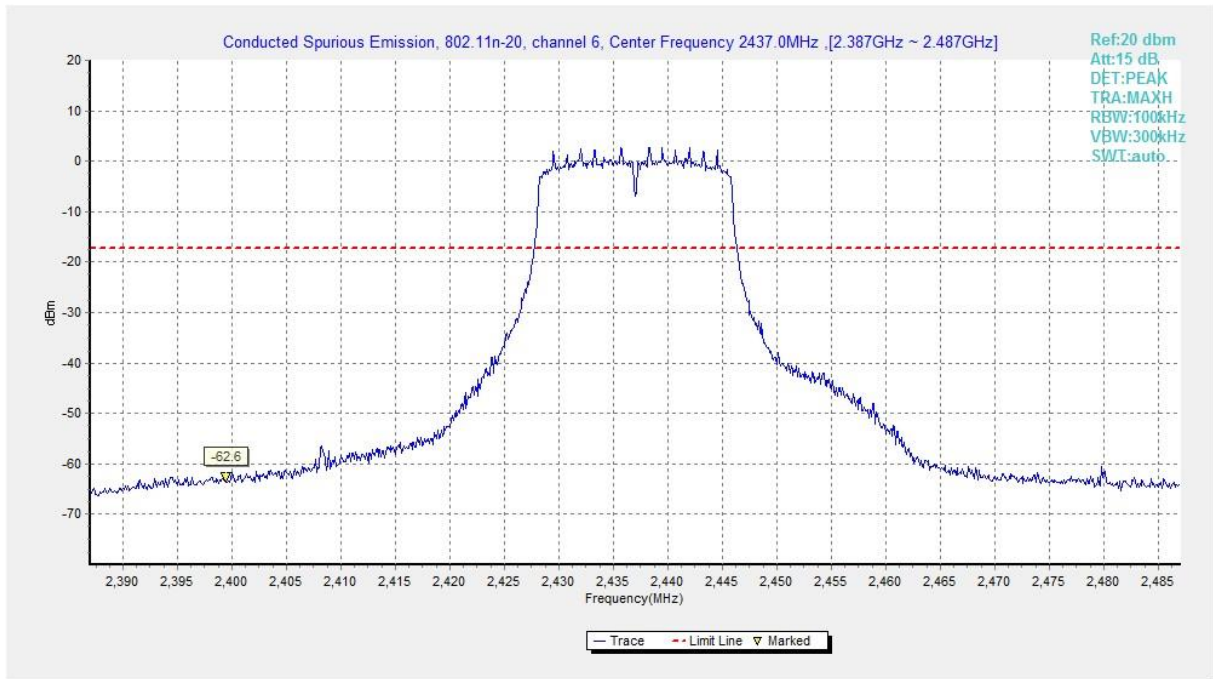
Fig.A.6.1.249 Transmitter Spurious Emission - Conducted (802.11n-HT20, Ch6, Center Frequency)
