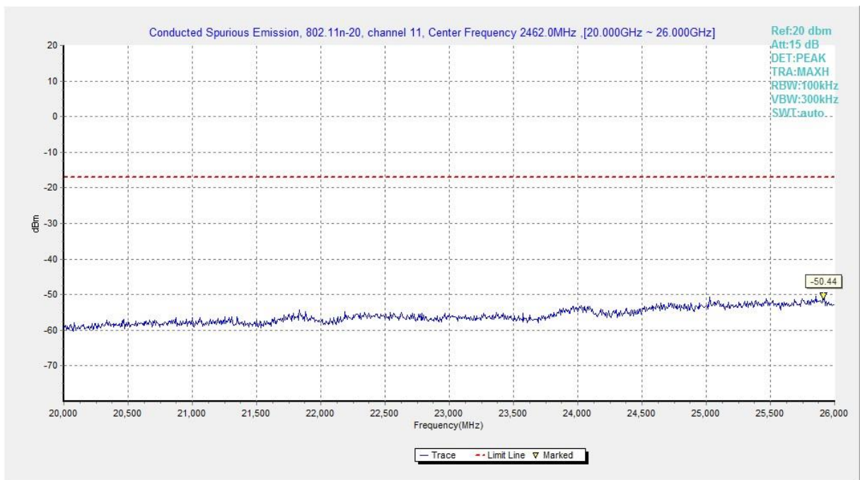
Fig.A.6.1.264 Transmitter Spurious Emission - Conducted (802.11n-HT20, Ch11, 20 GHz-26 GHz)
