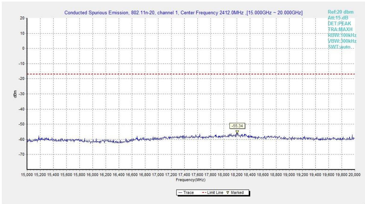
Fig.A.6.1.247 Transmitter Spurious Emission - Conducted (802.11n-HT20, Ch1, 15 GHz-20 GHz)
