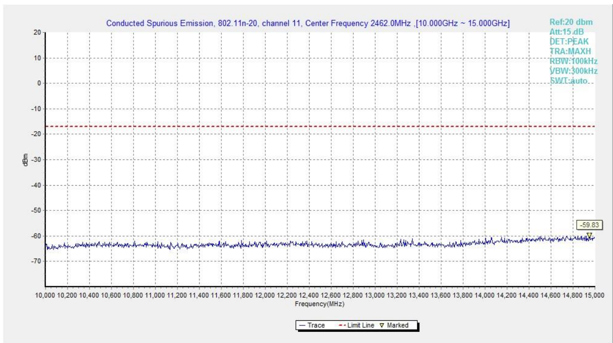
Fig.A.6.1.262 Transmitter Spurious Emission - Conducted (802.11n-HT20, Ch11, 10 GHz-15 GHz)
