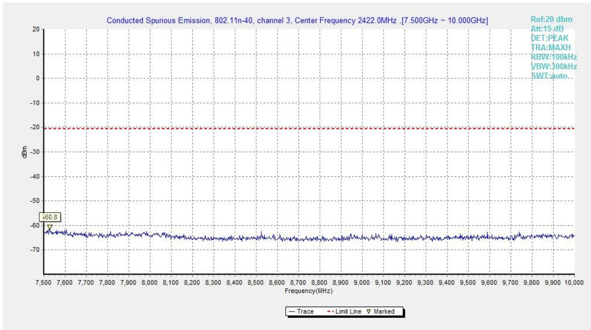
Fig.A.6.1.269 Transmitter Spurious Emission - Conducted (802.11n-HT40, Ch3, 7.5 GHz-10 GHz)
