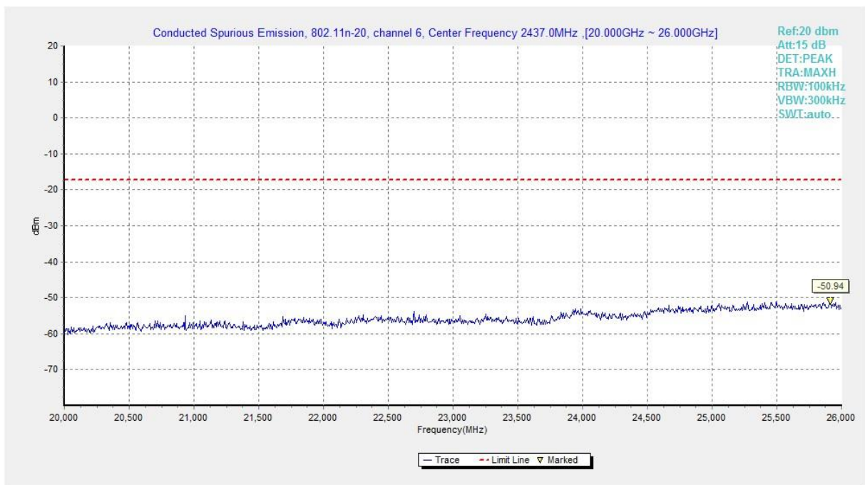
Fig.A.6.1.256 Transmitter Spurious Emission - Conducted (802.11n-HT20, Ch6, 20 GHz-26 GHz)
