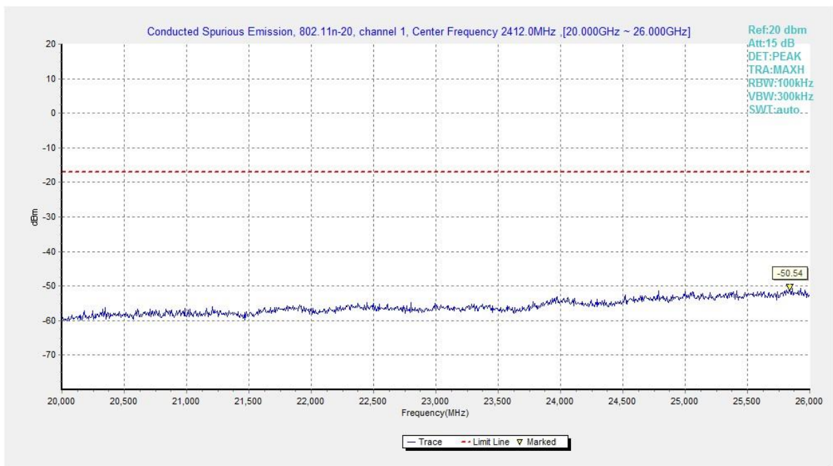
Fig.A.6.1.248 Transmitter Spurious Emission - Conducted (802.11n-HT20, Ch1, 20 GHz-26 GHz)
