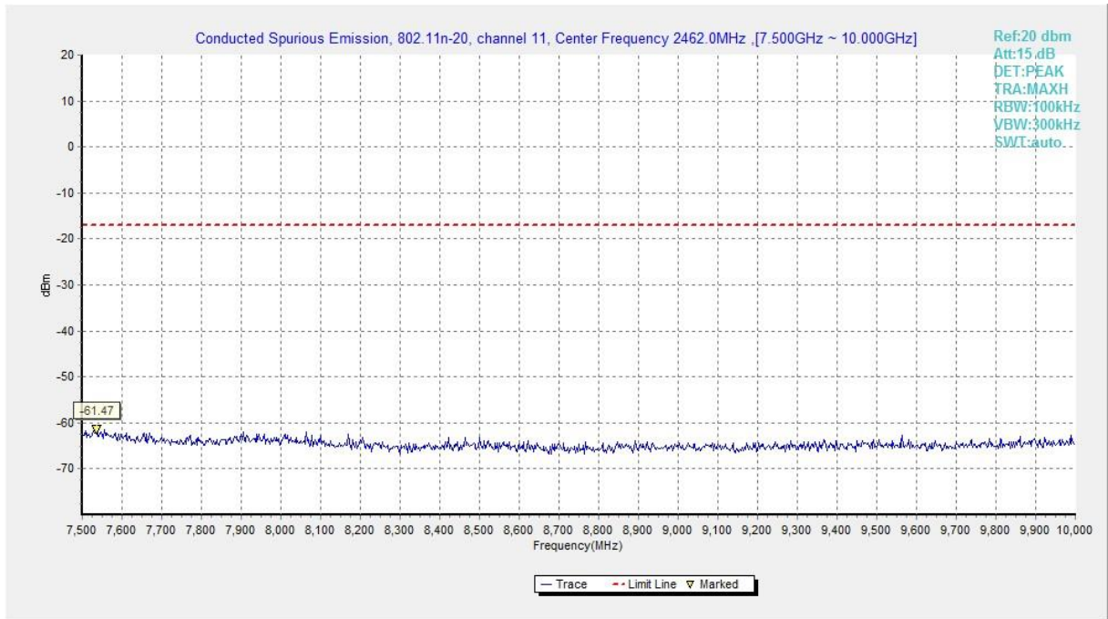
Fig.A.6.1.261 Transmitter Spurious Emission - Conducted (802.11n-HT20, Ch11, 7.5 GHz-10 GHz)
