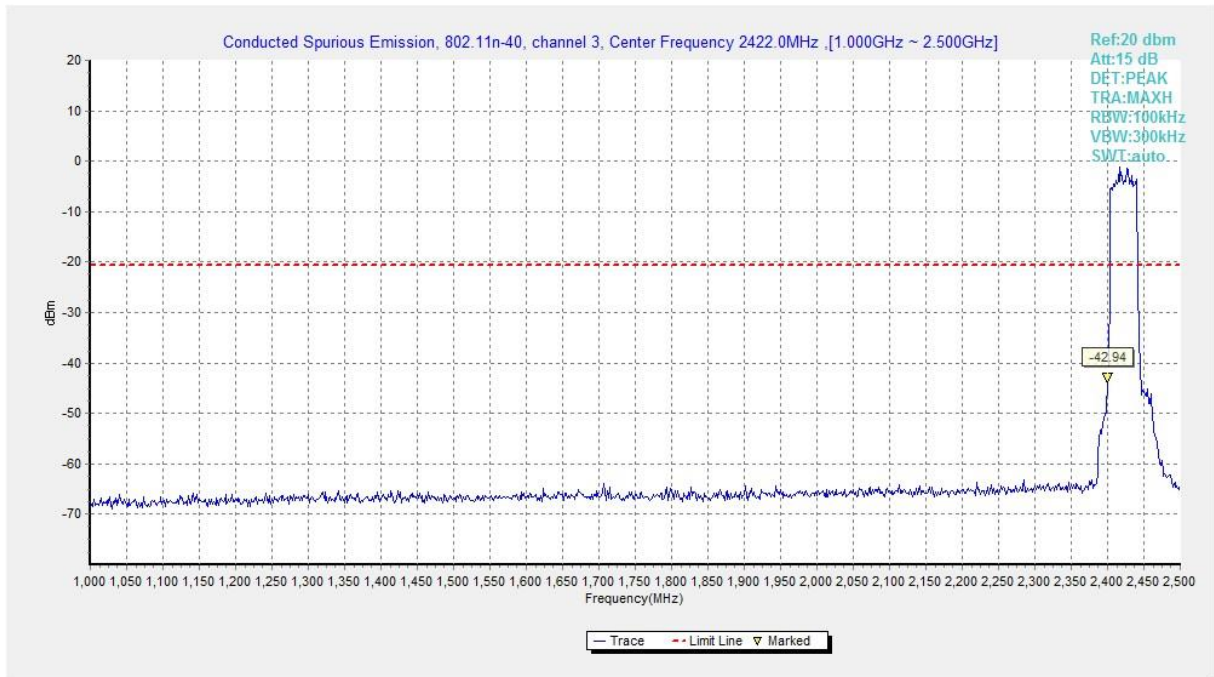
Fig.A.6.1.267 Transmitter Spurious Emission - Conducted (802.11n-HT40, Ch3, 1 GHz-2.5 GHz)
