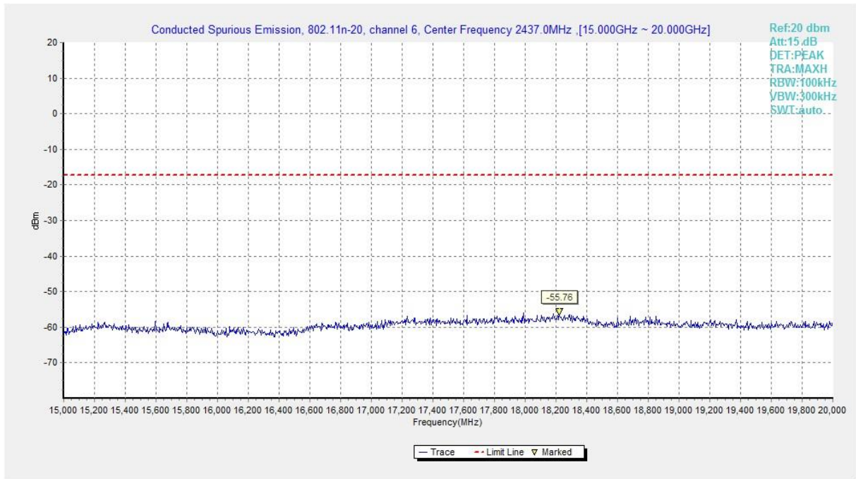
Fig.A.6.1.255 Transmitter Spurious Emission - Conducted (802.11n-HT20, Ch6, 15 GHz-20 GHz)
