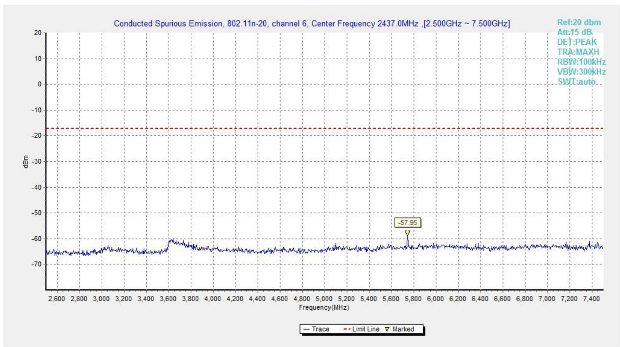
Fig.A.6.1.252 Transmitter Spurious Emission - Conducted (802.11n-HT20, Ch6, 2.5 GHz-7.5 GHz)
