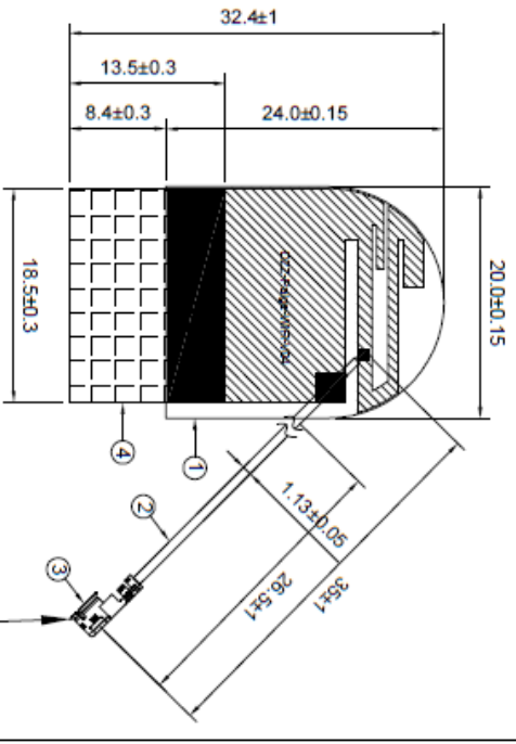
端子口侧立向下，如图所示 RF Plug side standing downwards
