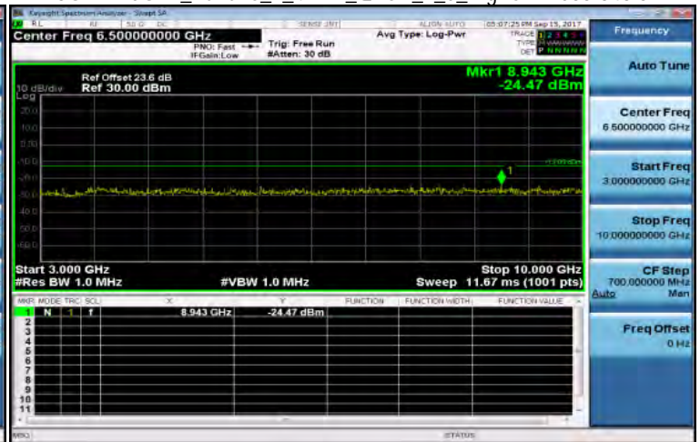
3GHz~10GHz_Band26_1_4MHz_QPSK_1_0_HighCH27033-848.3
