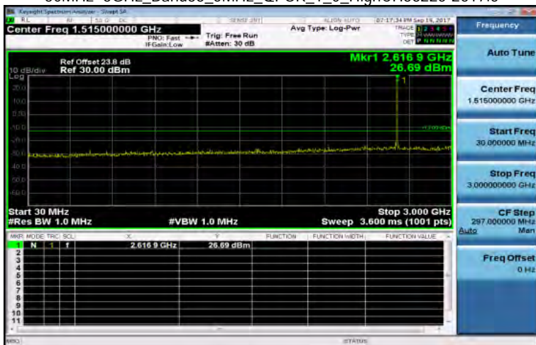
30MHz~3GHz_Band38_5MHz_QPSK_1_0_HighCH38225-2617.5
