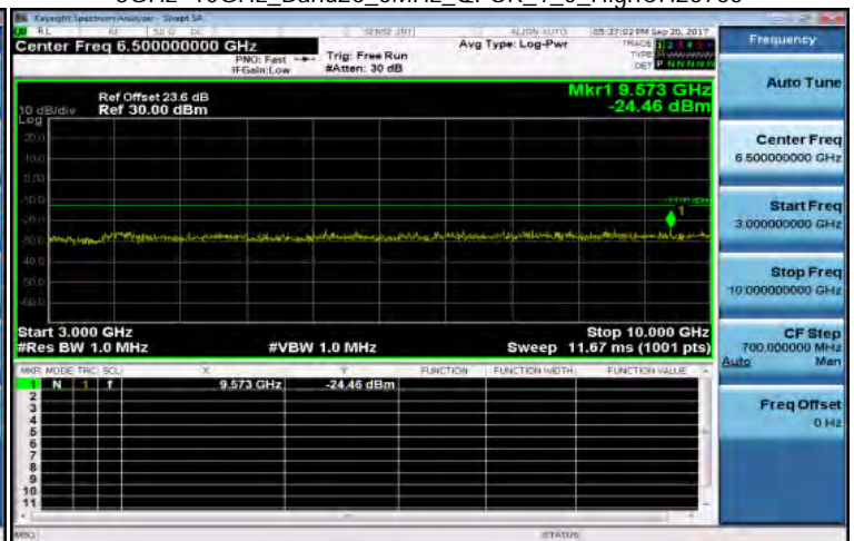
3GHz-10GHz_Band26_5MHz_QPSK_1_0_HighCH26765
