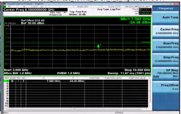
3GHz~10GHz_Band26_10MHz_QPSK_1_0_HighCH26990-844
