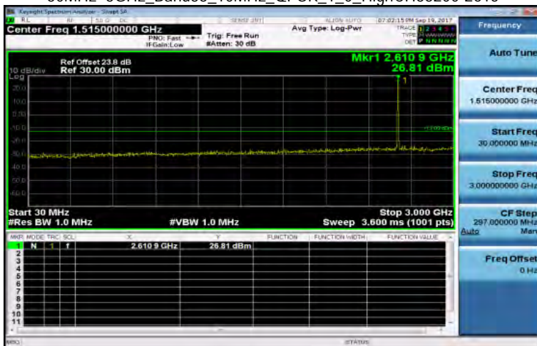
30MHz-3GHz_Band38_10MHz_QPSK_1_0_HighCH38200-2615
