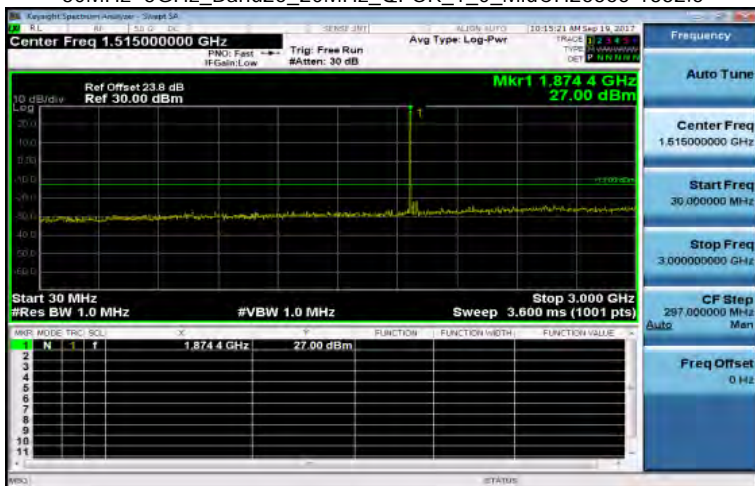
30MHz-3GHz_Band25_20MHz_QPSK_1_0_MidCH26365-1882.5
