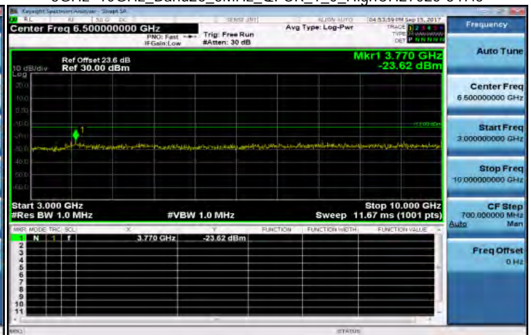
3GHz-10GHz_Band26_3MHz_QPSK_1_0_HighCH27025-847.5
