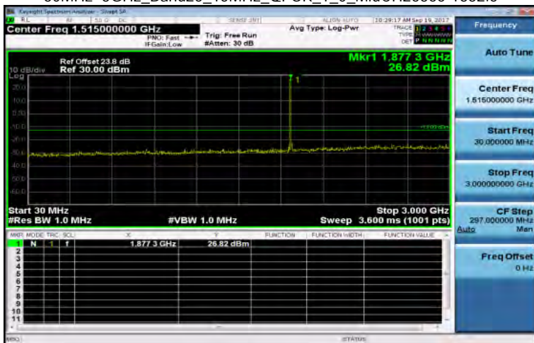
30MHz~3GHz_Band25_15MHz_QPSK_1_0_MidCH26365-1882.5
