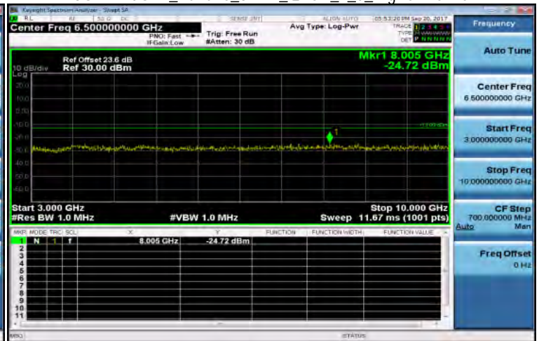
3GHz-10GHz_Band26_3MHz_QPSK_1_0_HighCH26775
