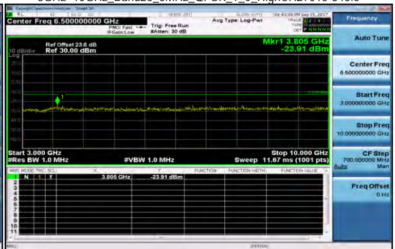
3GHz-10GHz_Band26_5MHz_QPSK_1_0_HighCH27015-846.5
