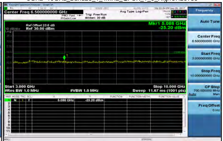
3GHz-10GHz_Band26_1_4MHz_QPSK_1_0_HighCH26783
