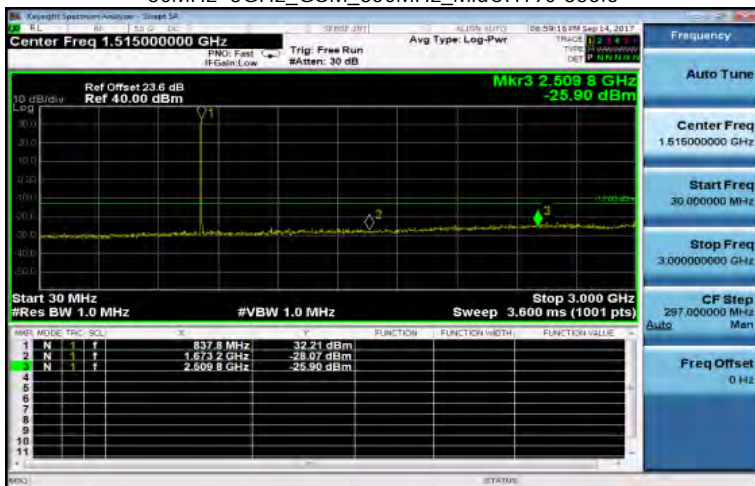
30MHz-3GHz_GSM_850MHz_MidCH190-836.6
