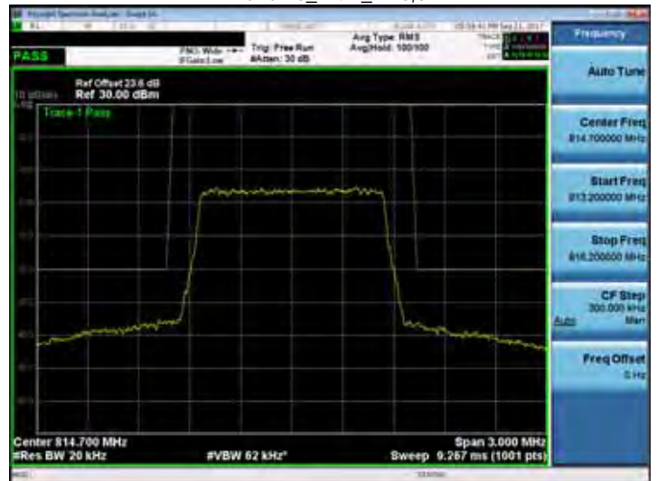
Band 26_1.4M_RB6,0
