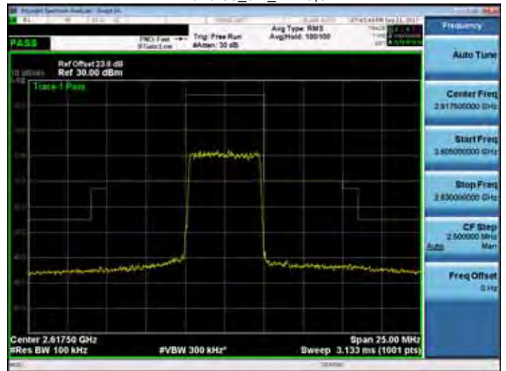
Band 38_5M_RB25,0
