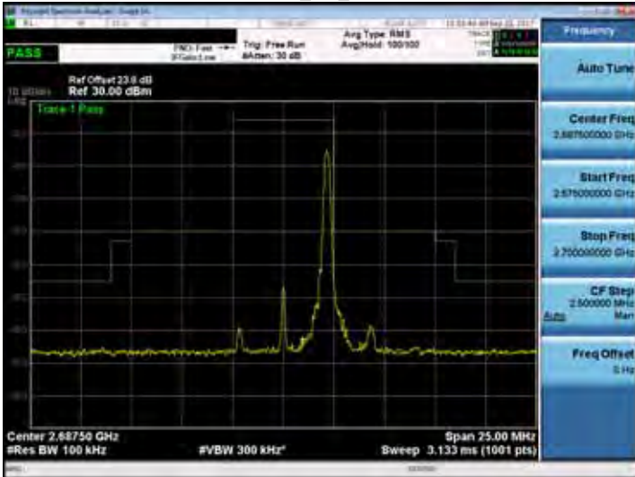
Band 41_5M_RB25,0
