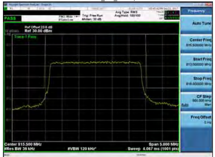
Band 26_3M_RB15,0
