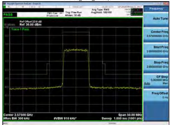
Band 38_10M_RB50,0
