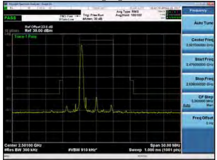
Band 41_10M_RB1,49
