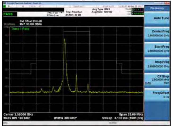
Band 41_5M_RB1,24
