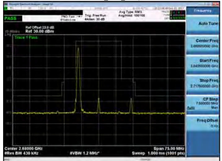
Band 41_20M_RB1,99
