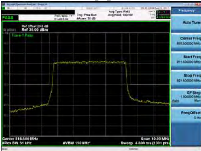
Band 26_5M_RB25,0
