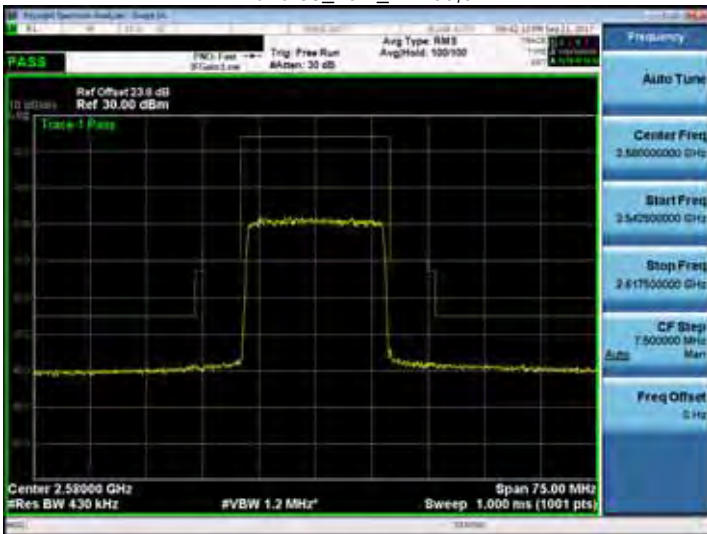
Band 38_20M_RB100,0
