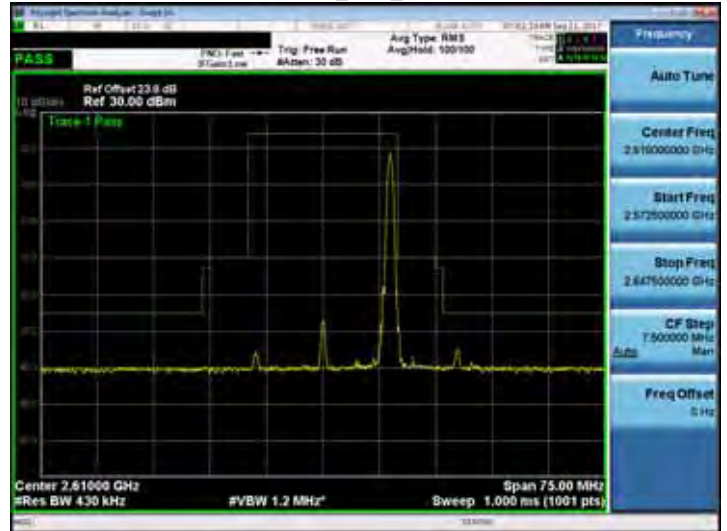
Band 38_20M_RB100,0
