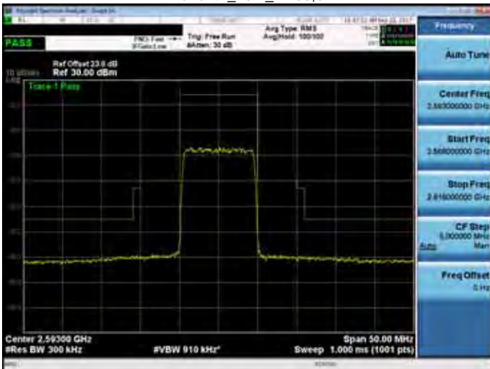
Band 41_10M_RB50,0
