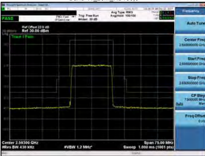
Band 41_20M_RB100,0
