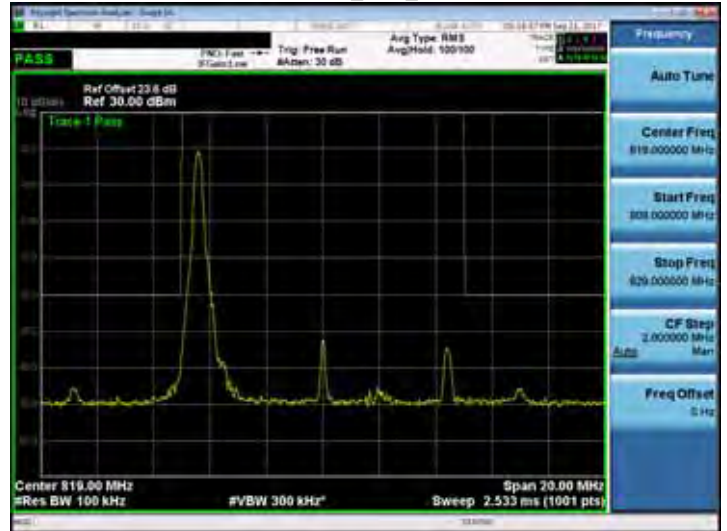
Band 26_10M_RB50,0
