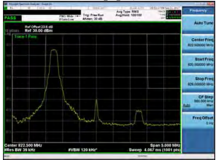
Band 26_3M_RB1,14
