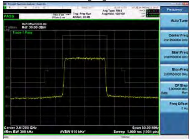
Band 38_15M_RB75,0
