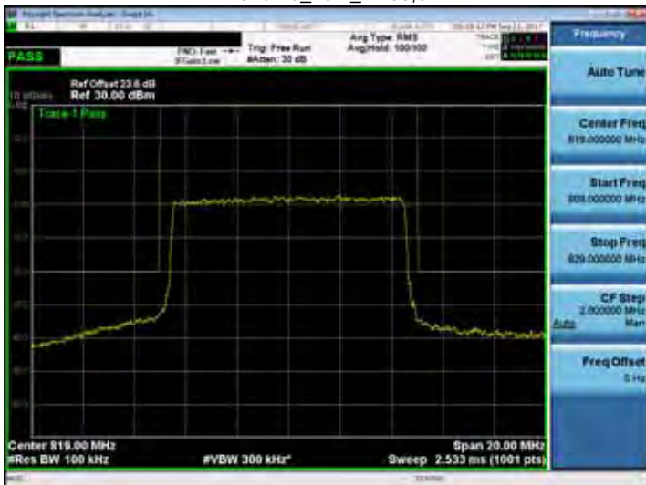
Band 26_10M_RB50,0
