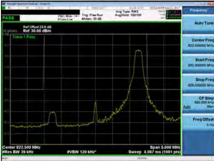
Band 26_3M_RB15,0
