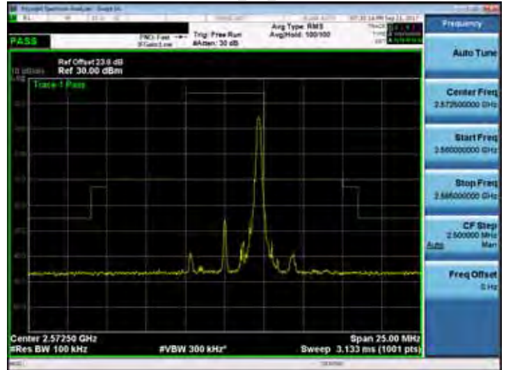
Band 38_5M_RB25,0
