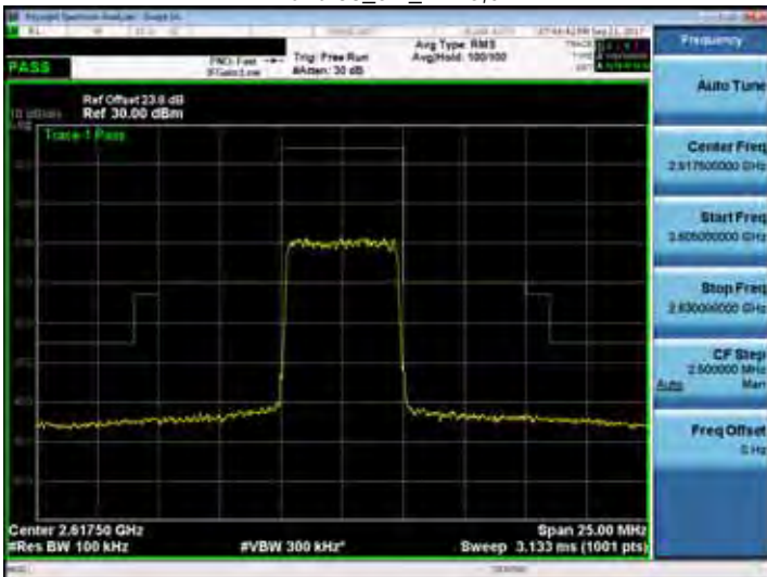
Band 38_5M_RB25,0
