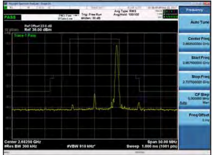
Band 41_15M_RB75,0
