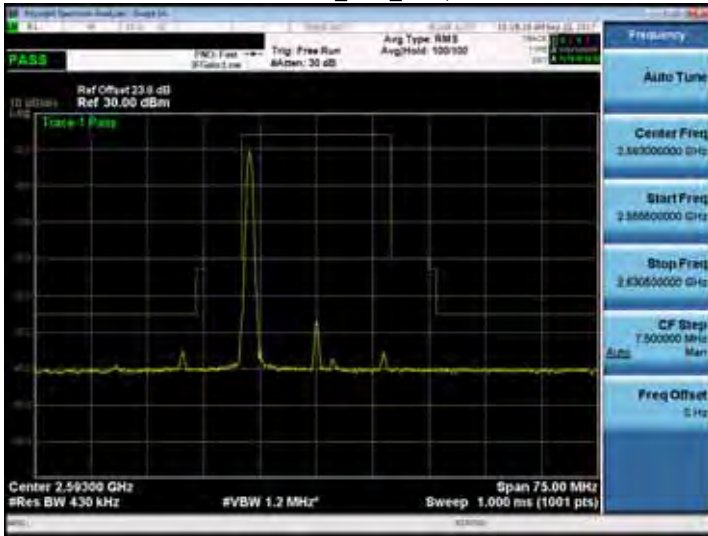
Band 41_20M_RB1,99
