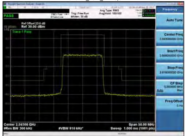
Band 41_15M_RB75,0
