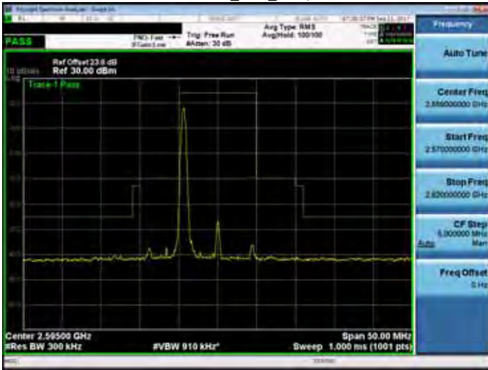
Band 38_10M_RB1,49
