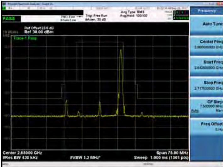
Band 41_20M_RB100,0
