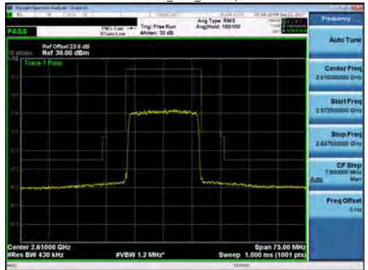
Band 38_20M_RB100,0
