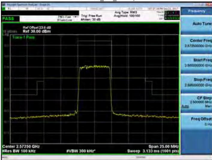
Band 38_5M_RB25,0
