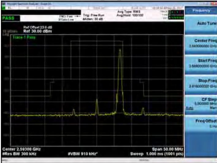
Band 41_15M_RB75,0
