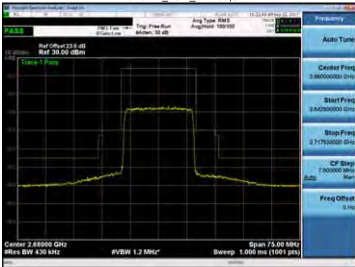
Band 41_20M_RB100,0
