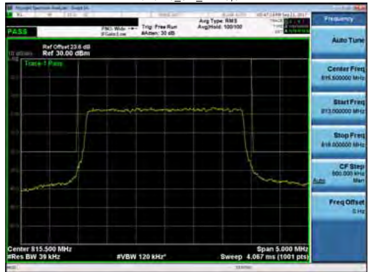
Band 26_3M_RB15,0
