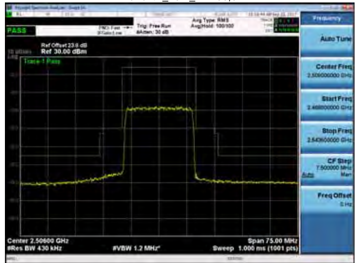
Band 41_20M_RB100,0
