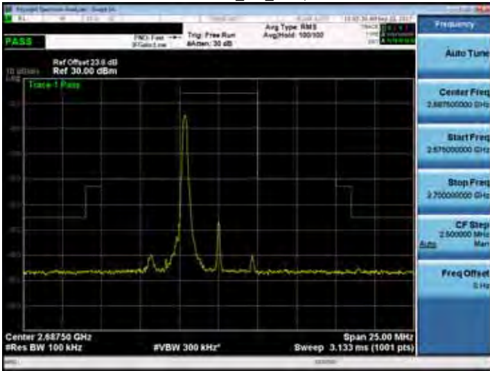
Band 41_5M_RB1,24
