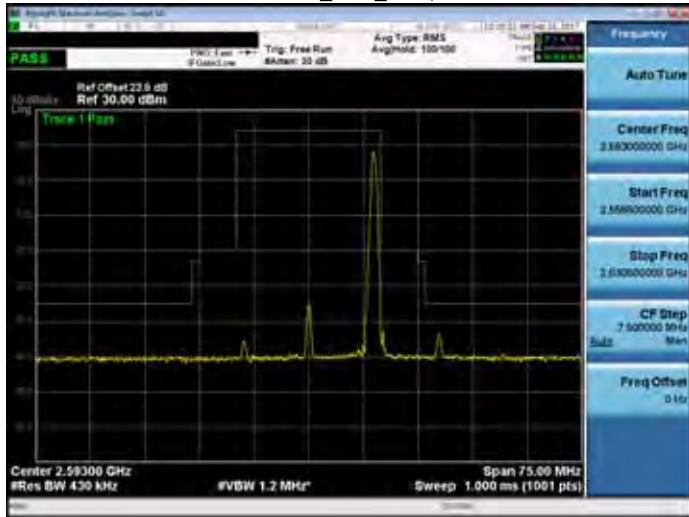
Band 41_20M_RB100,0
