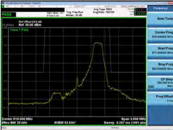
Band 26_1.4M_RB6,0
