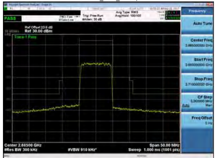
Band 41_10M_RB50,0
