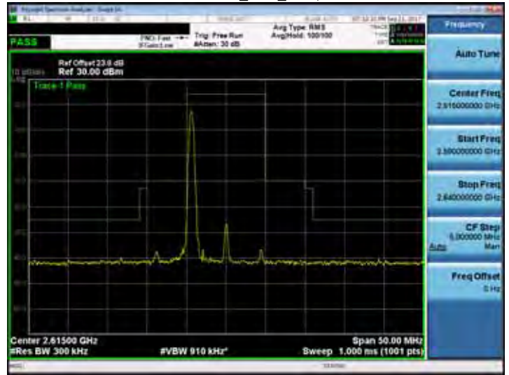
Band 38_10M_RB1,49
