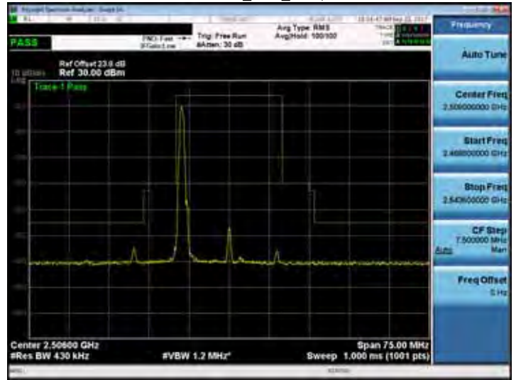
Band 41_20M_RB1,99
