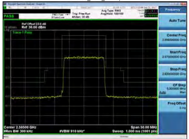
Band 38_15M_RB75,0
