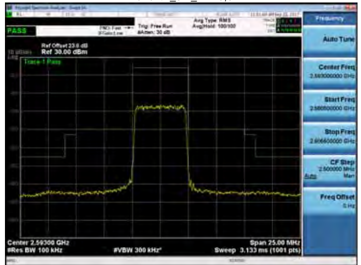
Band 41_5M_RB25,0
