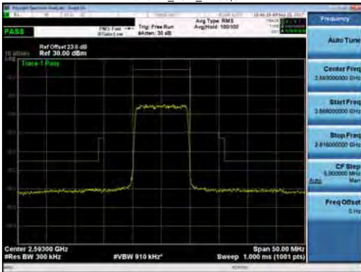
Band 41_10M_RB50,0
