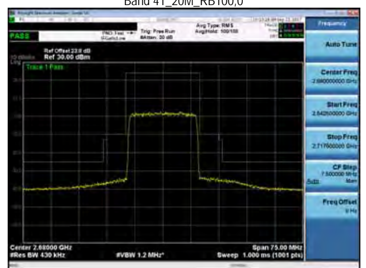
Band 41_20M_RB100,0
