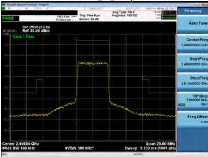
Band 41_5M_RB25,0
