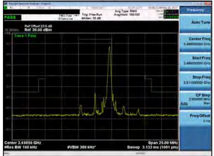
Band 41_5M_RB25,0
