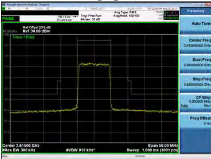
Band 38_10M_RB50,0
