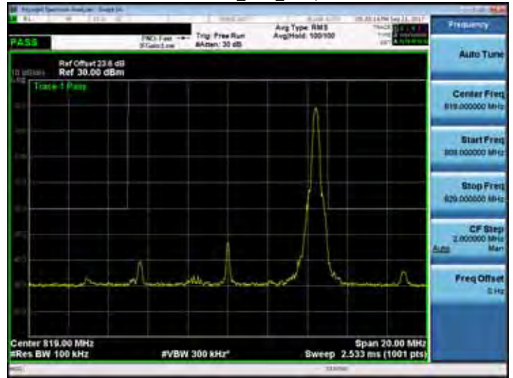
Band 26_10M_RB1
