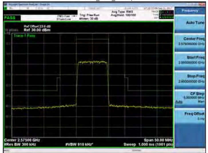
Band 38_10M_RB50,0
