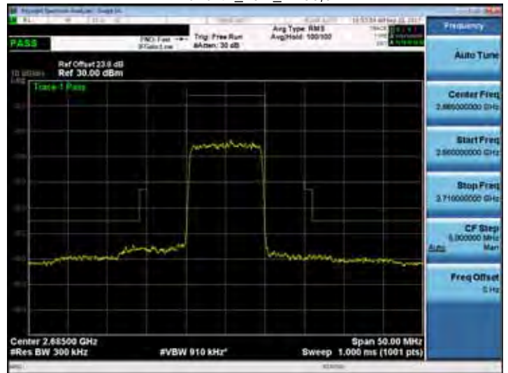
Band 41_10M_RB50,0
