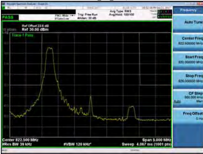
Band 26_3M_RB1,14
