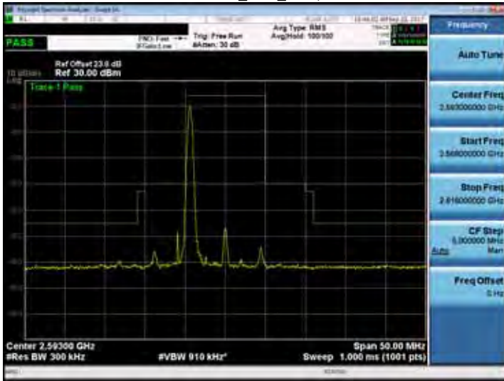
Band 41_10M_RB1,49
