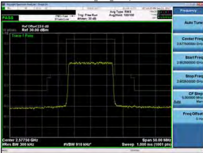
Band 38_15M_RB75,0
