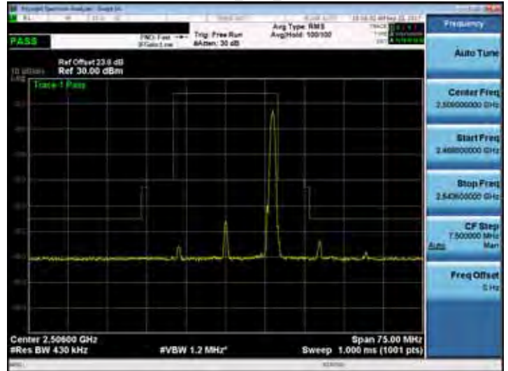
Band 41_20M_RB100,0
