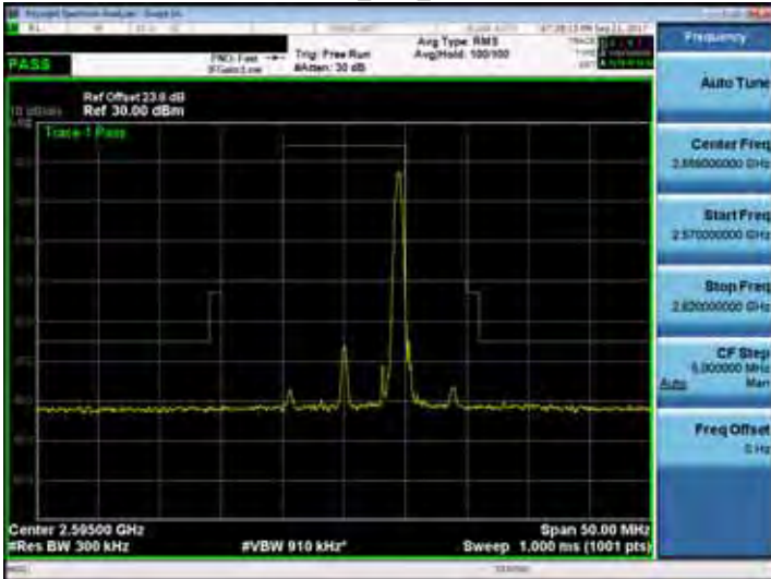
Band 38_10M_RB50,0
