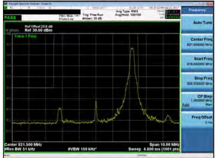
Band 26_5M_RB25,0
