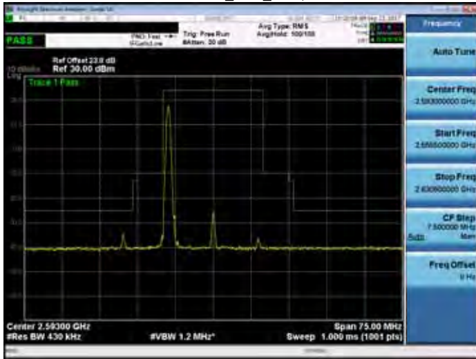
Band 41_20M_RB1,99
