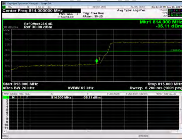
Part 90_Band26_1_4MHz_QPSK_6_0_LowCH26697
