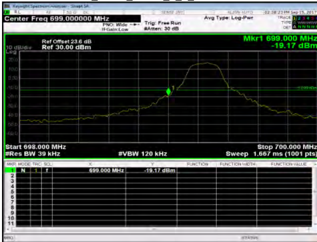
Band12_3MHz_QPSK_1_0_LowCH23025-700.5
