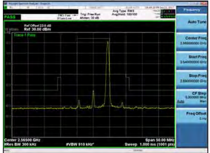
Band 7_10M_RB50,0
