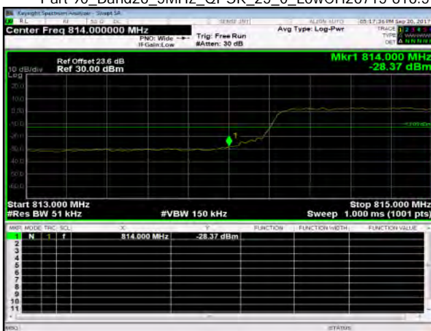
Part 90_Band26_5MHz_QPSK_25_0_LowCH26715-816.5
