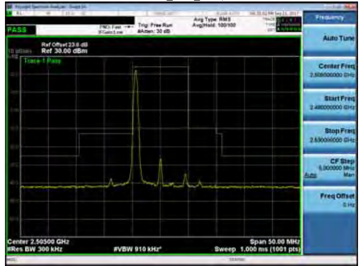
Band 7_10M_RB1,49
