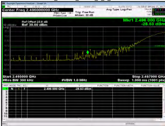
Band41_20MHz_QPSK_1_0_LowCH39750
