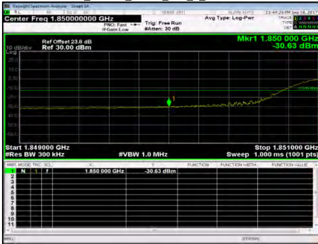
Band25_20MHz_QPSK_100_0_LowCH26140-1860
