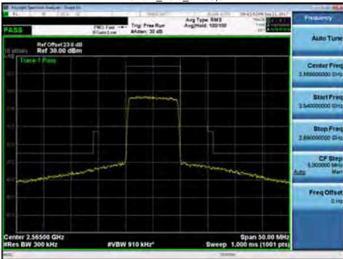
Band 7_10M_RB50,0
