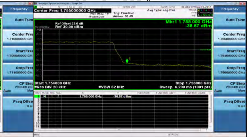
Band4_1_4MHz_QPSK_6_0_HighCH20393-1754.3
