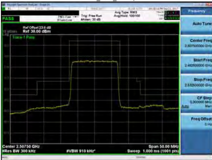
Band 7_15M_RB75,0
