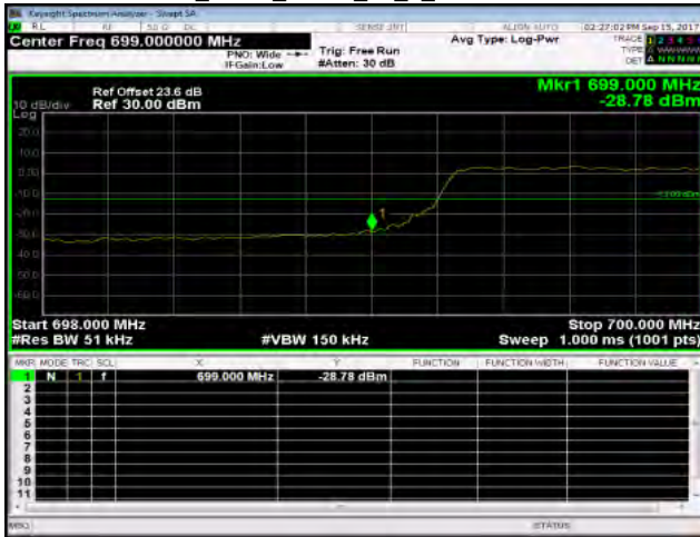
Band12_5MHz_QPSK_25_0_LowCH23035-701.5
