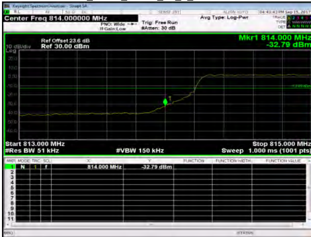
Band26_5MHz_QPSK_25_0_LowCH26715-816.5
