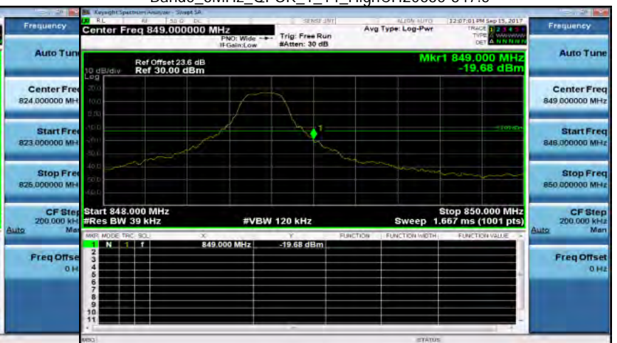
Band5_3MHz_QPSK_1_14_HighCH20635-847.5
