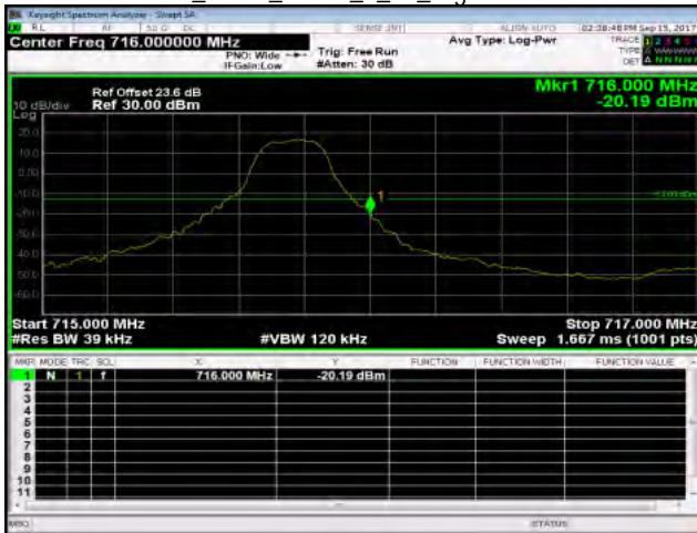
Band12_3MHz_QPSK_1_14_HighCH23165-714.5
