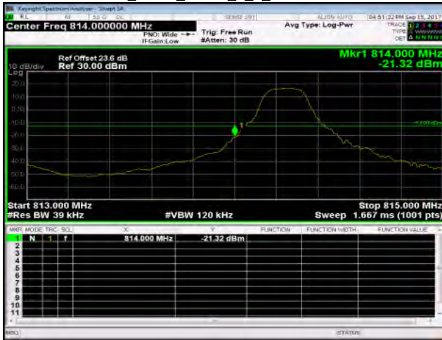
Band26_3MHz_QPSK_1_0_LowCH26705-815.5
