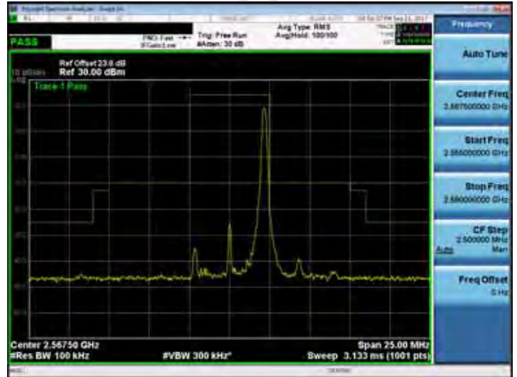
Band 7_5M_RB25,0
