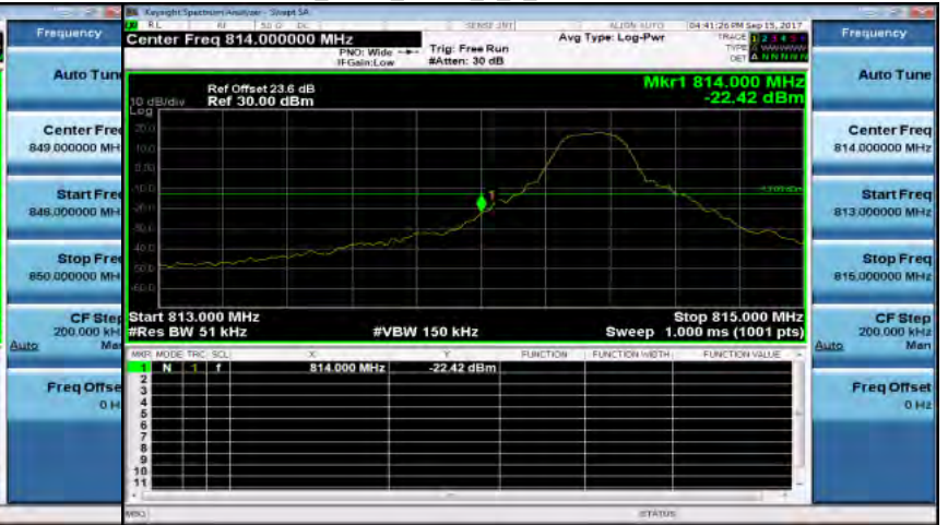
Band26_5MHz_QPSK_1_0_LowCH26715-816.5
