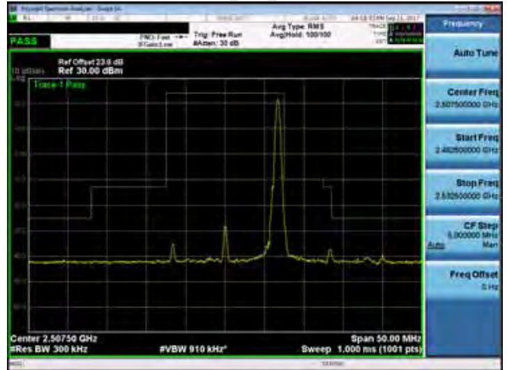
Band 7_15M_RB75,0
