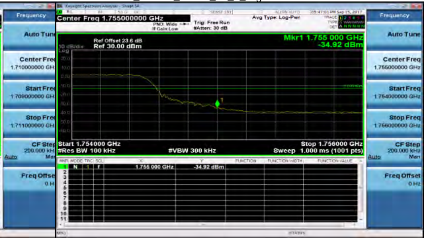
Band4_10MHz_QPSK_50_0_HighCH20350-1750
