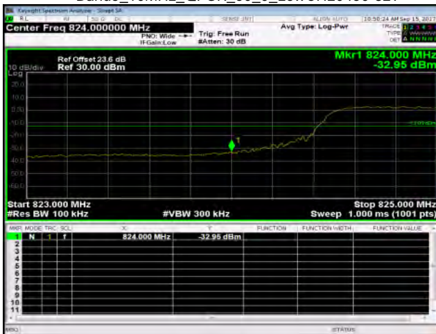
Band5_10MHz_QPSK_50_0_LowCH20450-829
