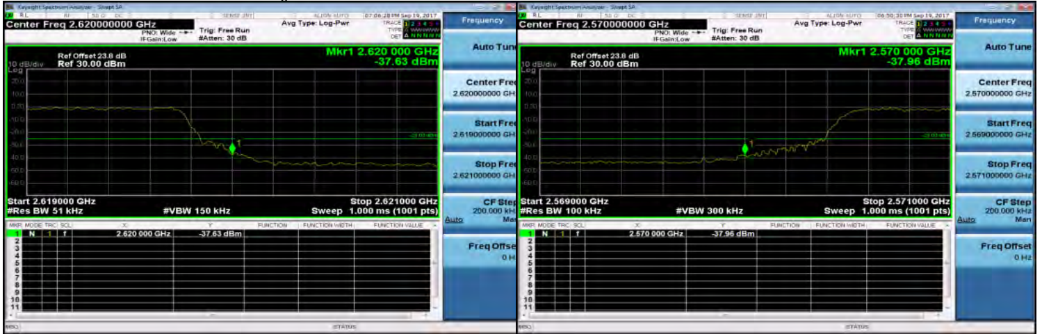
Band38_5MHz_QPSK_25_0_HighCH38225-2617.5
