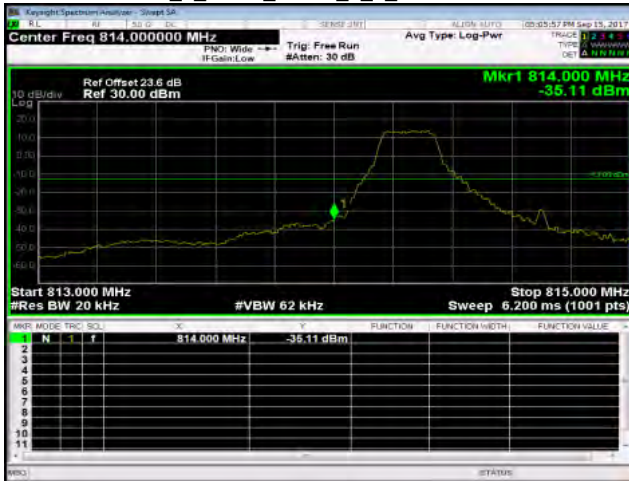
Band26_1_4MHz_QPSK_1_0_LowCH26697-814.7
