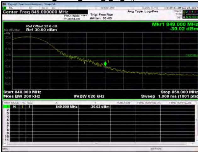
Band26_15MHz_QPSK_1_74_HighCH26965-841.5
