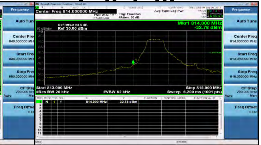
Part 90_Band26_1_4MHz_QPSK_1_0_LowCH26697
