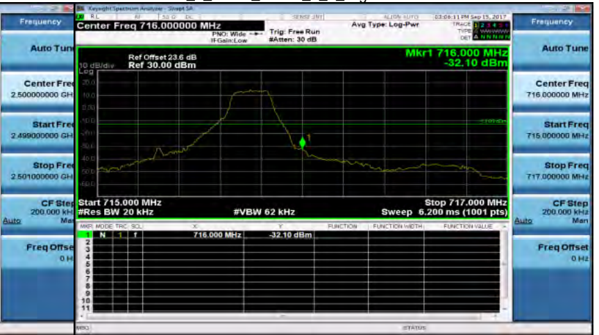
Band12_1_4MHz_QPSK_1_5_HighCH23173-715.3
