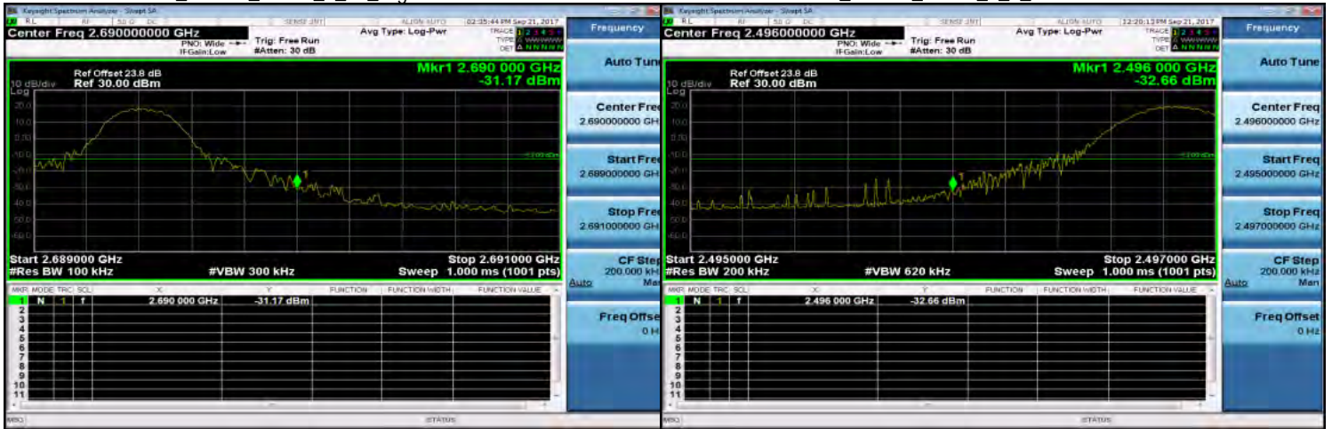
Band41_10MHz_QPSK_1_49_HighCH41540
