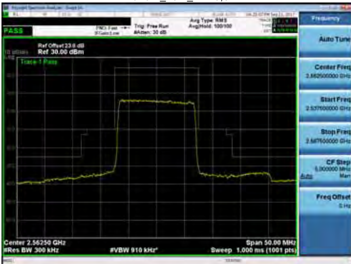
Band 7_15M_RB75,0
