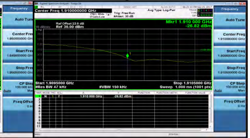
HSDPA_B2_HighCH9538-1907.6
