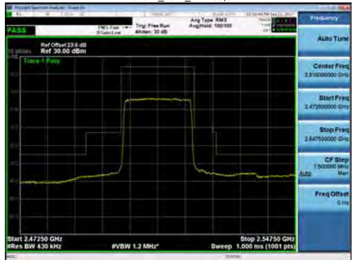
Band 7_20M_RB100,0
