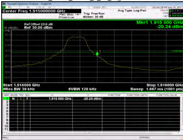
Band25_3MHz_QPSK_1_14_HighCH26675-1913.5
