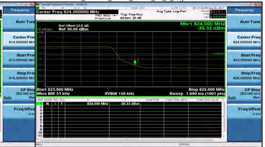
Part 90_Band26_5MHz_QPSK_25_0_HighCH26765
