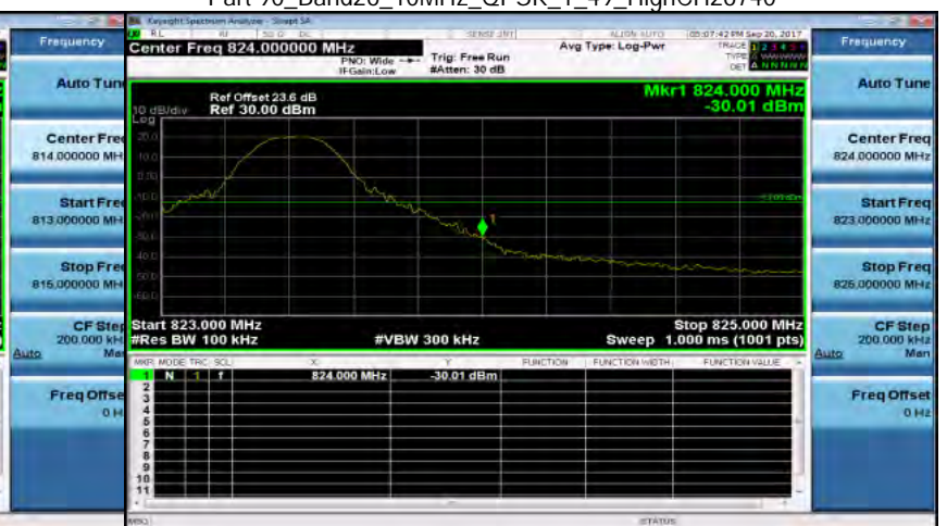
Part 90_Band26_10MHz_QPSK_1_49_HighCH26740
