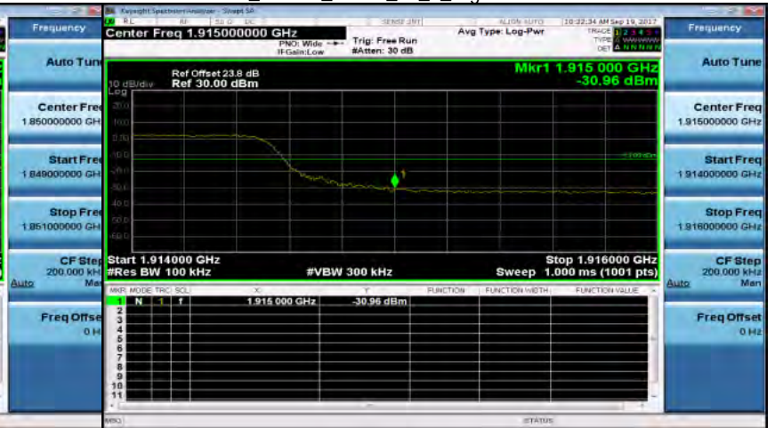
Band25_10MHz_QPSK_50_0_HighCH26640-1910
