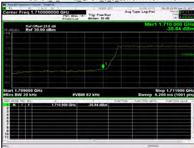
Band4_1_4MHz_QPSK_6_0_LowCH19957-1710.7
