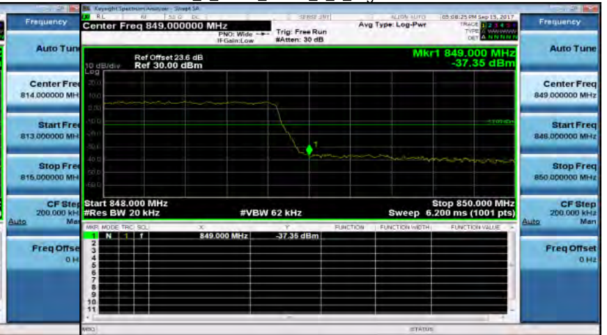
Band26_1_4MHz_QPSK_6_0_HighCH27033-848.3
