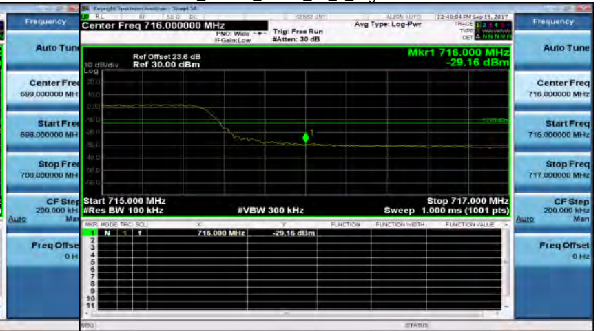
Band12_10MHz_QPSK_50_0_HighCH23130-711
