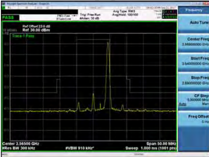
Band 7_10M_RB50,0
