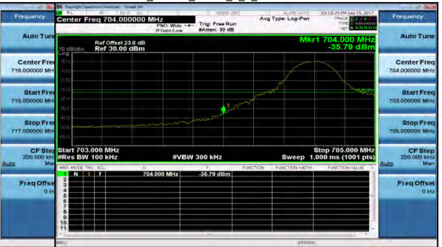
Band17_10MHz_QPSK_1_0_LowCH23780-709
