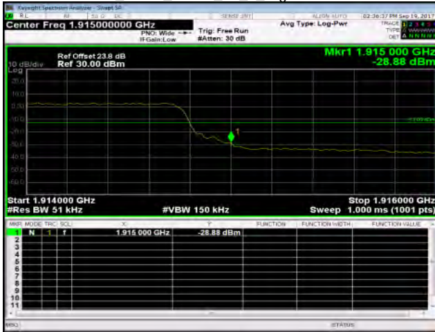
Band25_5MHz_QPSK_25_0_HighCH26665-1912.5
