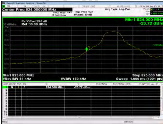
Band5_5MHz_QPSK_1_0_LowCH20425-826.5
