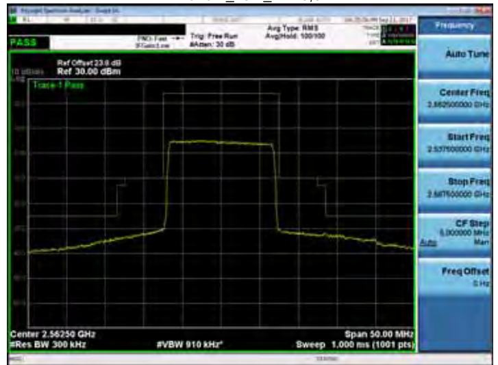
Band 7_15M_RB75,0
