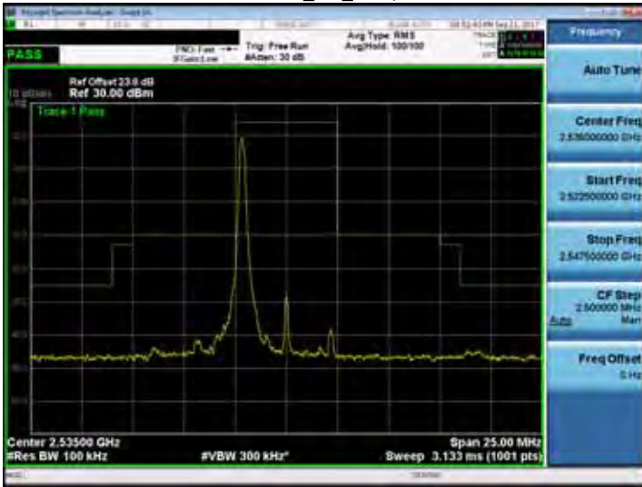
Band 7_5M_RB1,24
