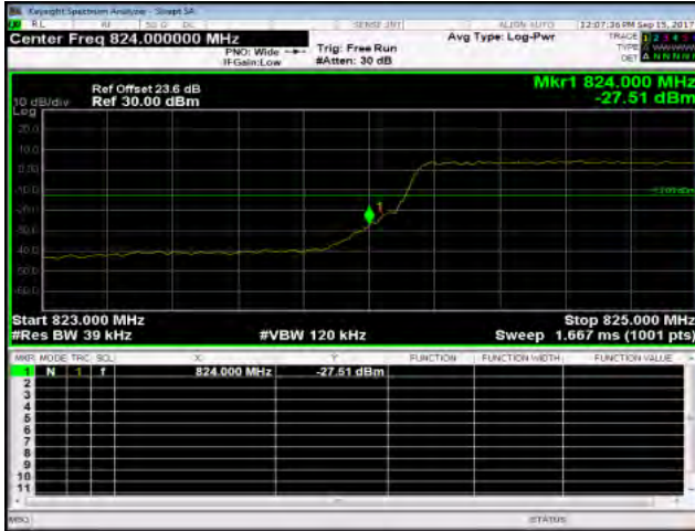
Band5_3MHz_QPSK_15_0_LowCH20415-825.5
