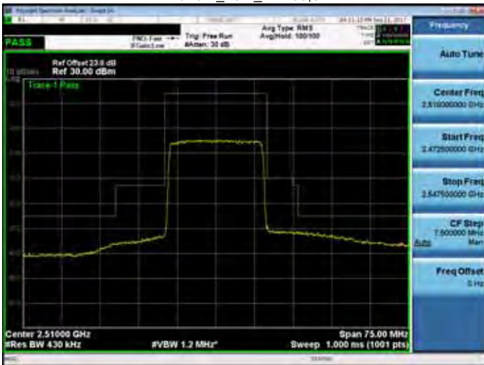
Band 7_20M_RB100,0
