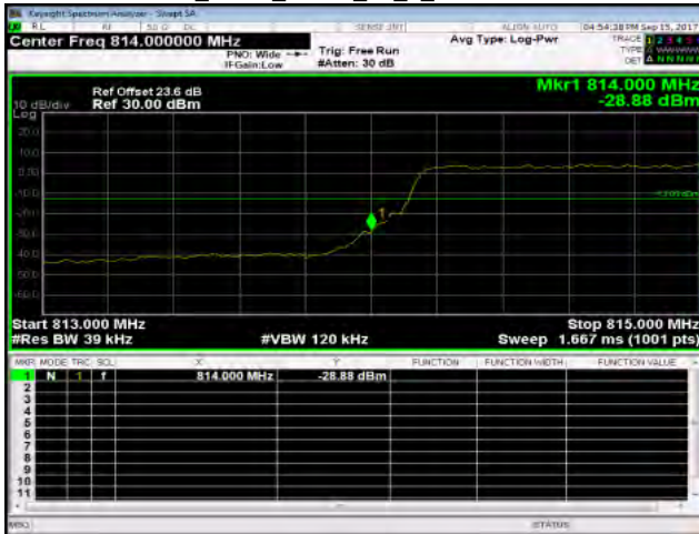
Band26_3MHz_QPSK_15_0_LowCH26705-815.5
