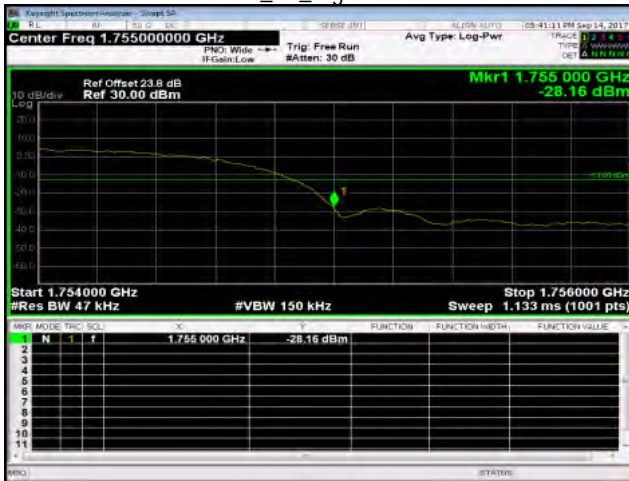
WCDMA_B4_HighCH1513-1752.6
