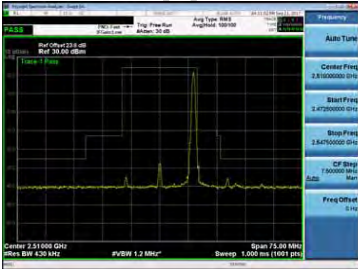
Band 7_20M_RB100,0
