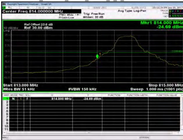
Part 90_Band26_5MHz_QPSK_1_0_LowCH26715-816.5
