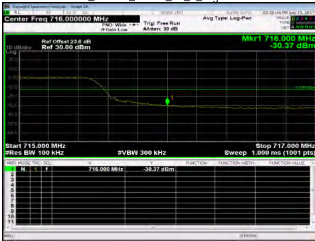
Band17_10MHz_QPSK_50_0_HighCH23800-711
