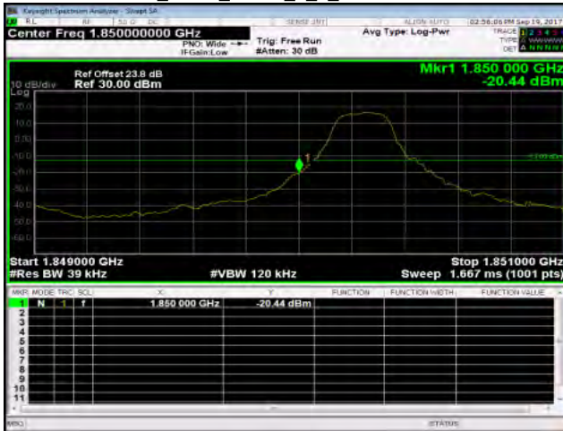
Band25_3MHz_QPSK_1_0_LowCH26055-1851.5
