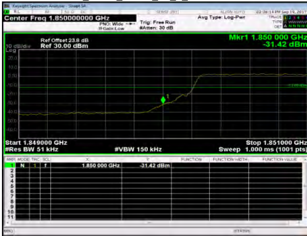
Band25_5MHz_QPSK_25_0_LowCH26065-1852.5
