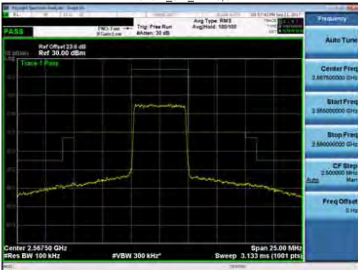
Band 7_5M_RB25,0
