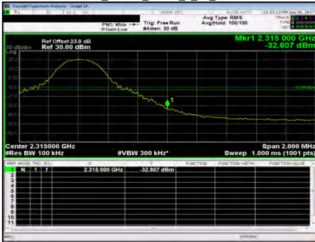
Band30_10MHz_QPSK_1_49_MidCH27710
