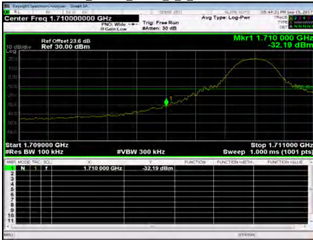
Band4_10MHz_QPSK_1_0_LowCH20000-1715
