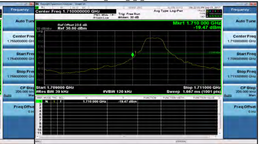
Band4_3MHz_QPSK_1_0_LowCH19965-1711.5
