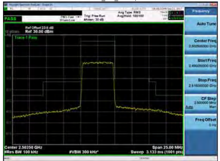
Band 7_5M_RB25,0
