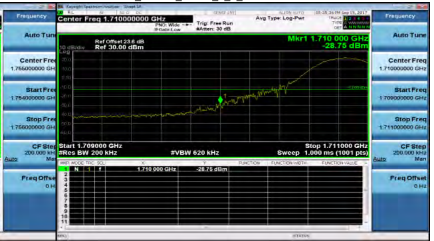
Band4_15MHz_QPSK_1_0_LowCH20025-1717.5
