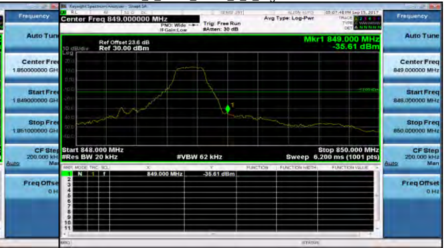
Band26_1_4MHz_QPSK_1_5_HighCH27033-848.3
