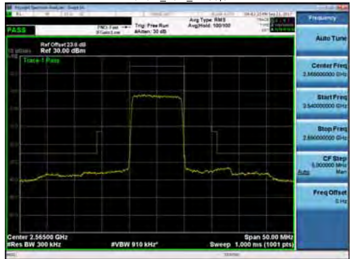
Band 7_10M_RB50,0
