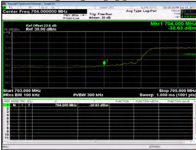
Band17_10MHz_QPSK_50_0_LowCH23780-709
