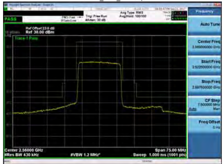
Band 7_20M_RB100,0
