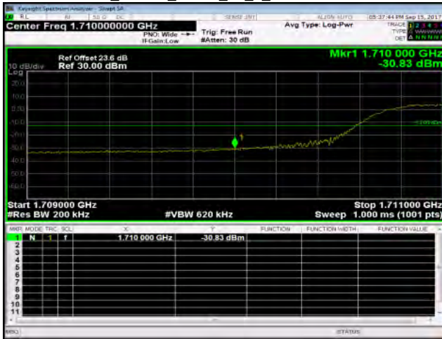
Band4_15MHz_QPSK_75_0_LowCH20025-1717.5
