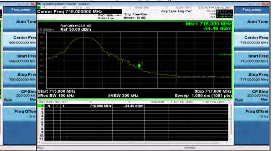
Band12_10MHz_QPSK_1_49_HighCH23130-711
