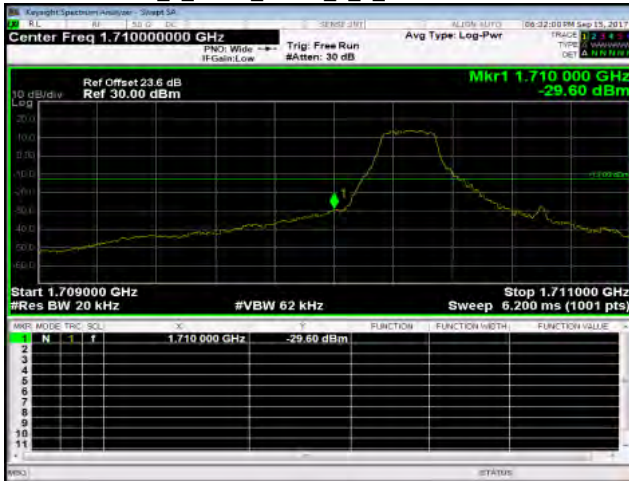
Band4_1_4MHz_QPSK_1_0_LowCH19957-1710.7
