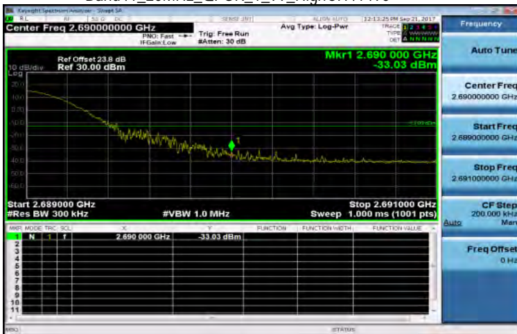
Band41_20MHz_QPSK_1_99_HighCH41490
