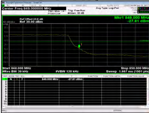
Band5_3MHz_QPSK_15_0_HighCH20635-847.5
