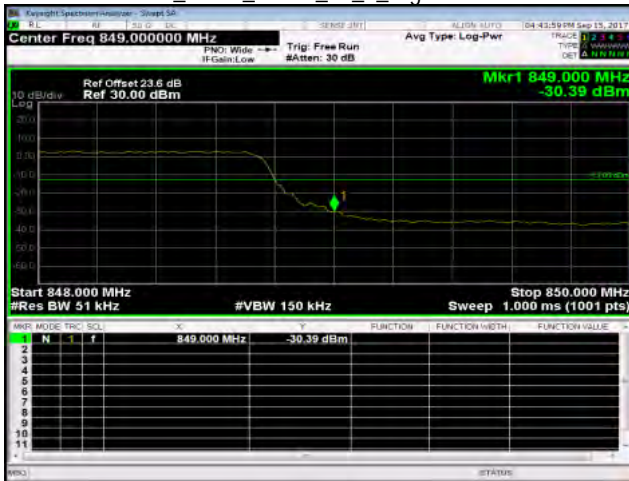
Band26_5MHz_QPSK_25_0_HighCH27015-846.5
