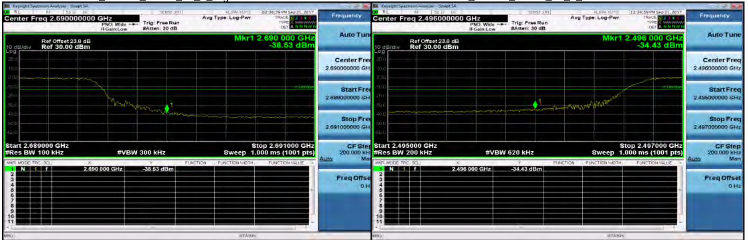
Band41_10MHz_QPSK_50_0_HighCH41540
