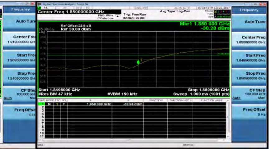
HSUPA_B2_LowCH9262-1852.4
