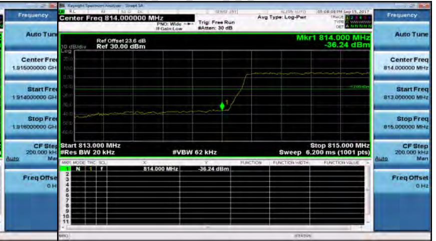
Band26_1_4MHz_QPSK_6_0_LowCH26697-814.7
