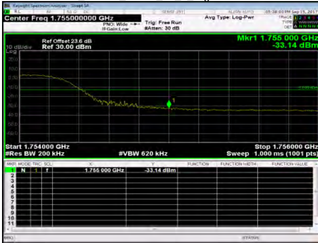
Band4_15MHz_QPSK_75_0_HighCH20325-1747.5
