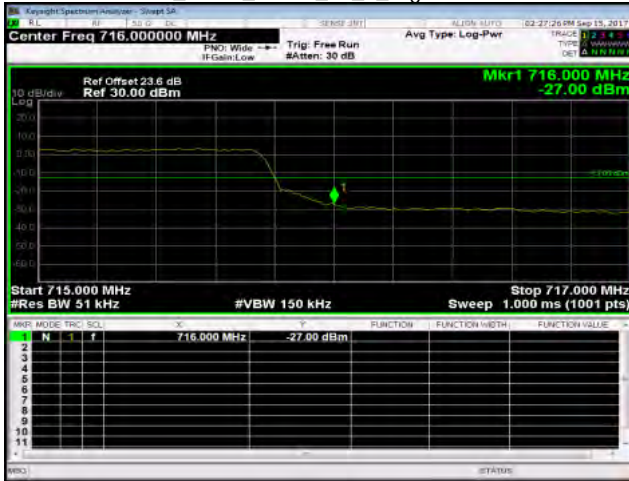
Band12_5MHz_QPSK_25_0_HighCH23155-713.5
