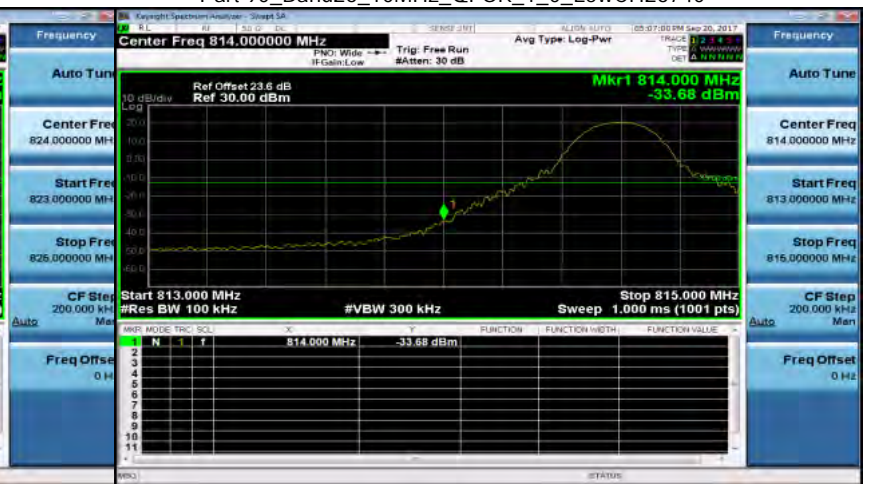
Part 90_Band26_10MHz_QPSK_1_0_LowCH26740
