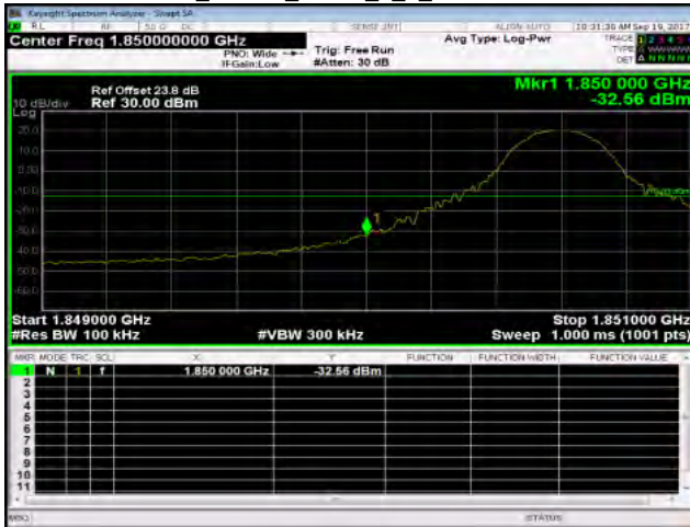
Band25_10MHz_QPSK_1_0_LowCH26090-1855
