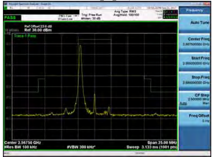
Band 7_5M_RB1,24
