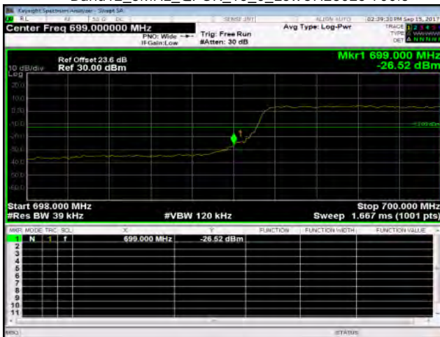
Band12_3MHz_QPSK_15_0_LowCH23025-700.5
