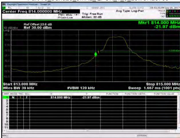
Part 90_Band26_3MHz_QPSK_1_0_LowCH26705
