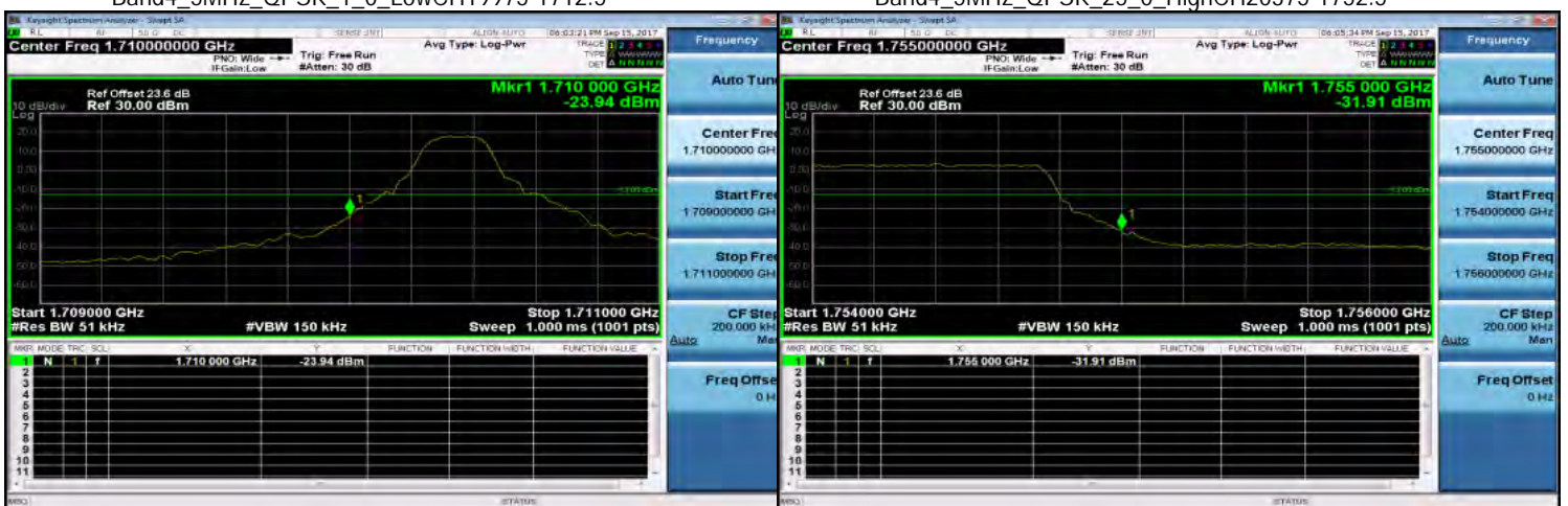
Band4_5MHz_QPSK_1_0_LowCH19975-1712.5
