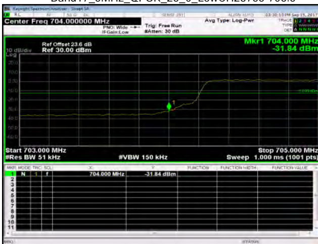
Band17_5MHz_QPSK_25_0_LowCH23755-706.5
