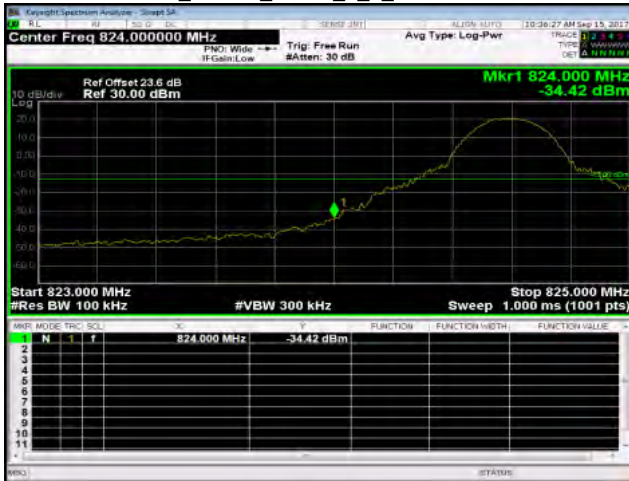
Band5_10MHz_QPSK_1_0_LowCH20450-829
