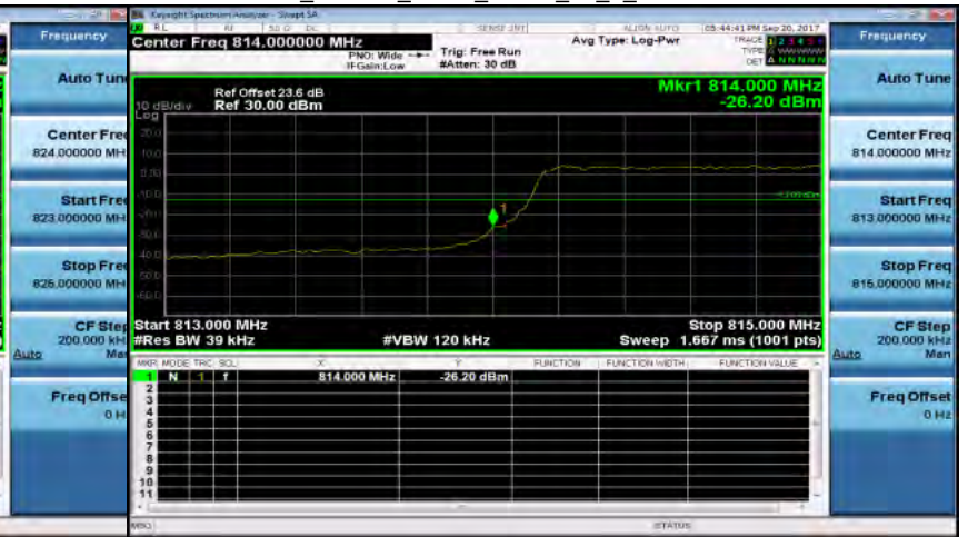
Part 90_Band26_3MHz_QPSK_15_0_LowCH26705
