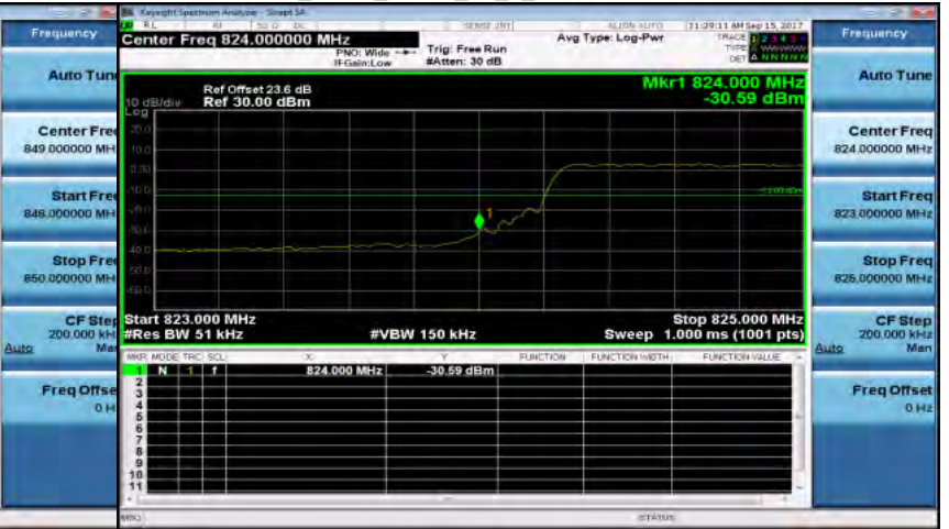
Band5_5MHz_QPSK_25_0_LowCH20425-826.5
