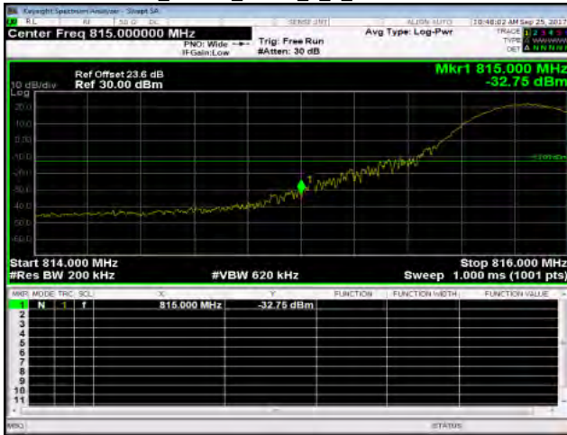
Band26_15MHz_QPSK_1_0_LowCH26775-822.5
