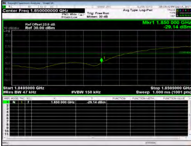
WCDMA_B2_LowCH9262-1852.4
