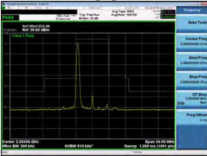
Band 7_10M_RB1,49
