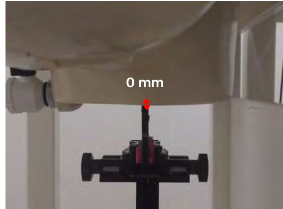
Fig.19 EUT Right side to flat phantom
