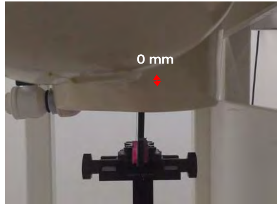
Fig.20 EUT Left side to flat phantom
