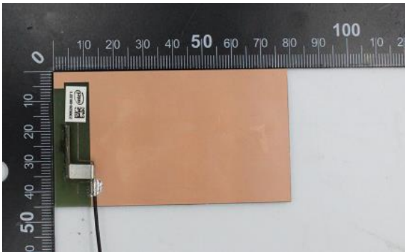
Main antenna
