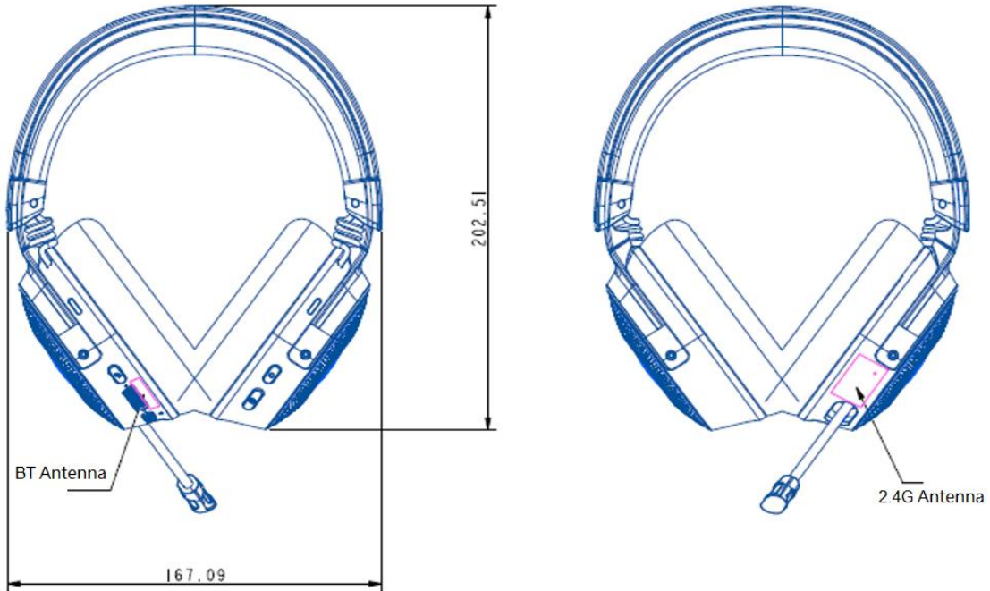
Unit: mm
