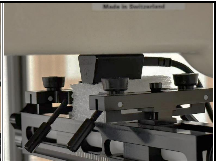
Horizontal Down of USB Dongle with 0 cm Gap
