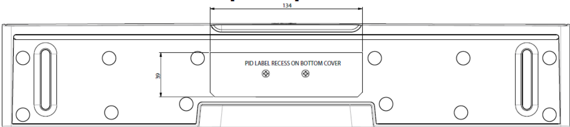
Noa T2 [Soundbar] - BOTTOM VIEW
