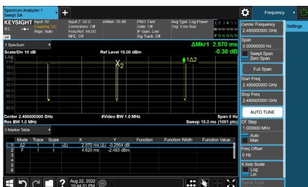
CH78 (2480MHz) DFSK(1 Mbps)- Duty Cycle
