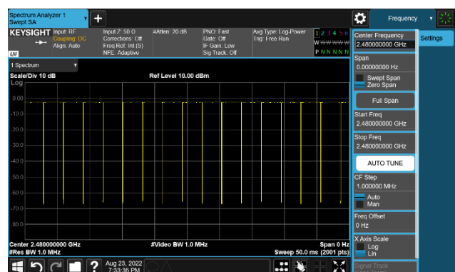
CH78 (2480MHz) DFSK(1 Mbps)- Dwell time
