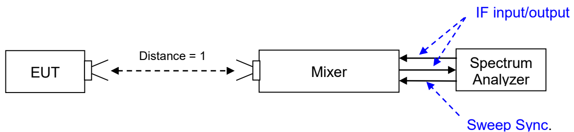
Measurement set up for EIRP
