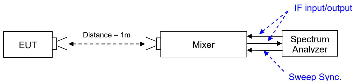
Measurement set up for Peak Output Power
