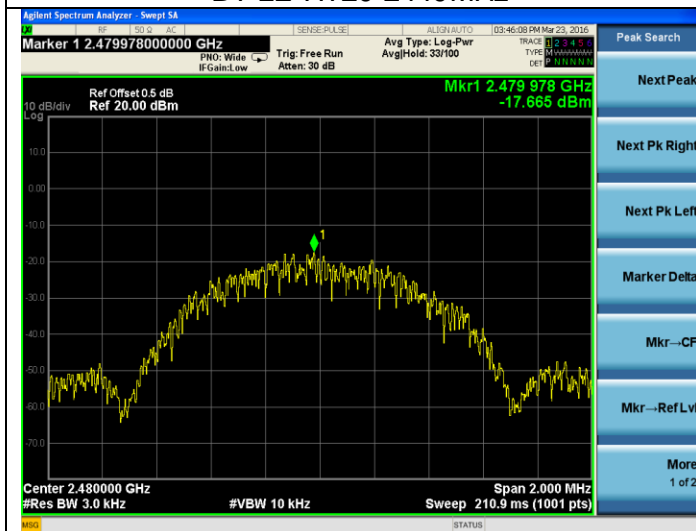
BT LE-2480MHz
