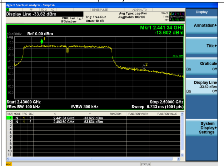
802.11n(HT40)-2452MHz
