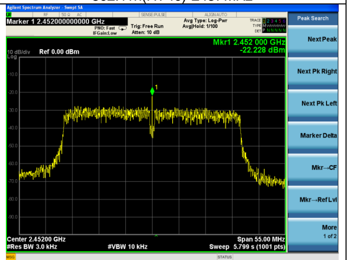
802.11n(HT40)-2452MHz
