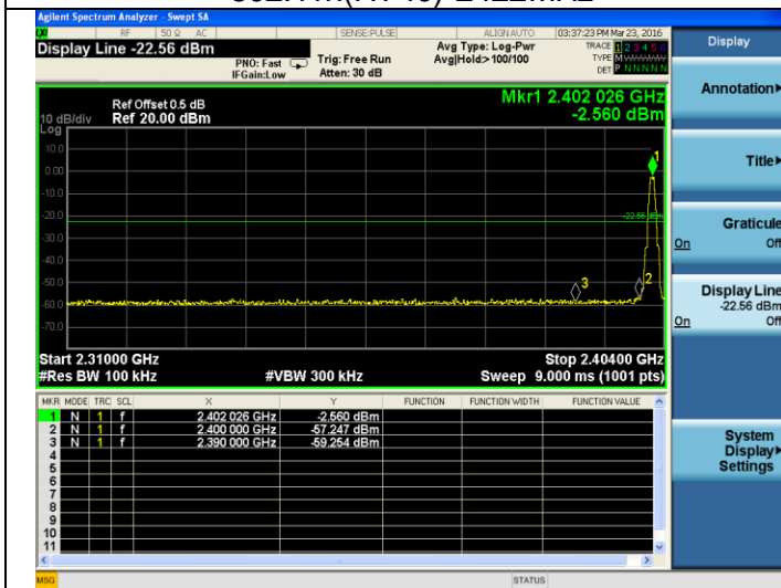
BT LE-2402MHz
