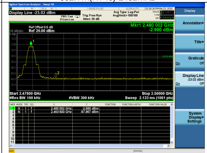
BT LE-2480MHz
