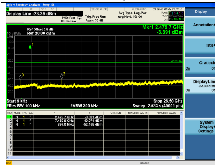
BT LE-2480MHz
