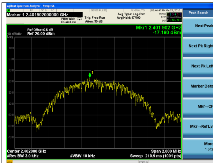
BT LE-2402MHz
