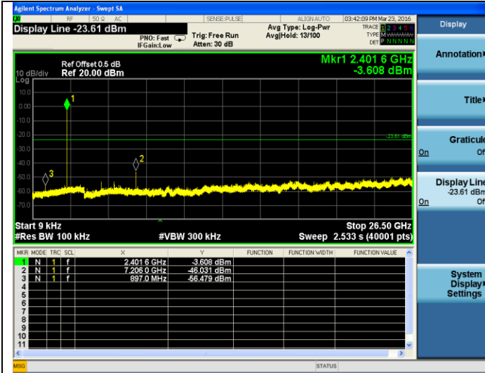
BT LE-2402MHz
