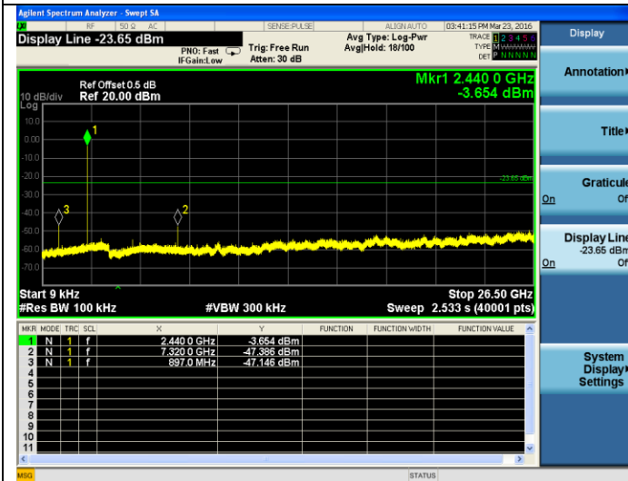
BT LE-2440MHz
