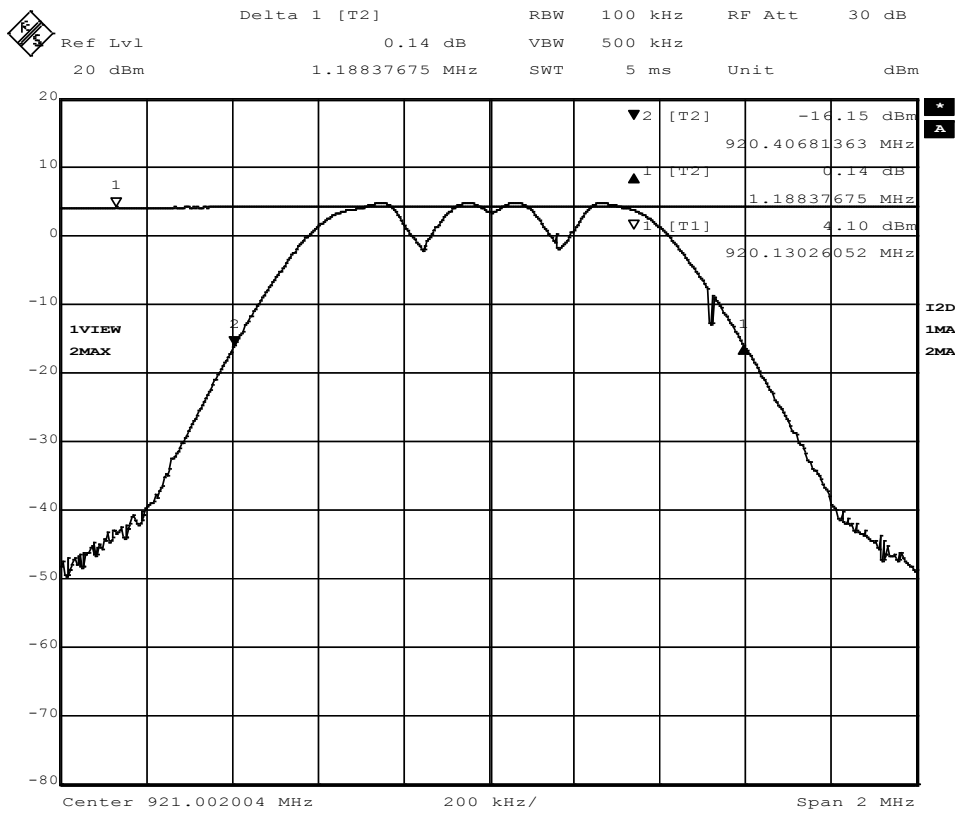
Figure 14 - 99% Occupied Bandwidth
