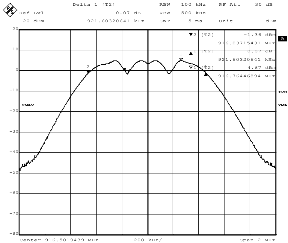
Figure 11 - 6dB Bandwidth
