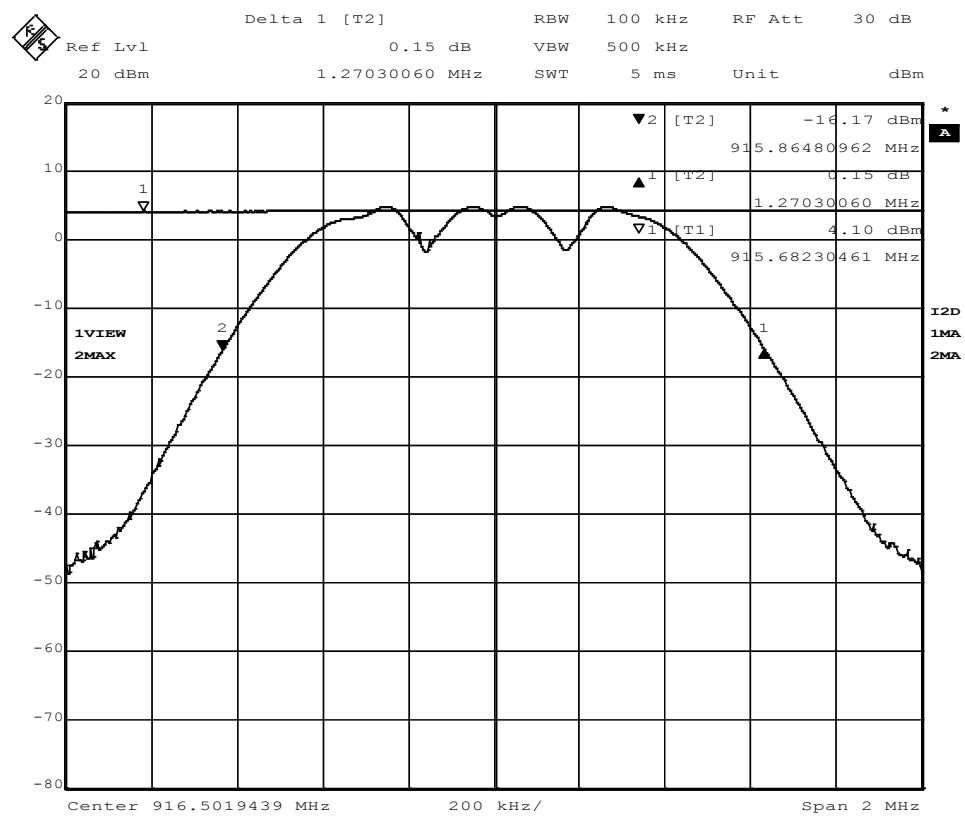
Figure 12 - 99% Occupied Bandwidth
