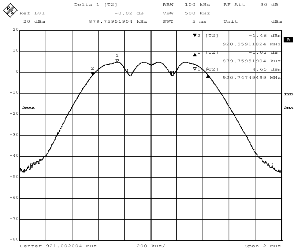
Figure 13 - 6dB Bandwidth
