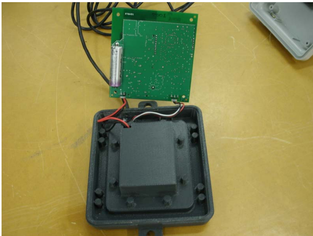
Figure 2 - Internal Photo showing back of circuit board and capacitor
