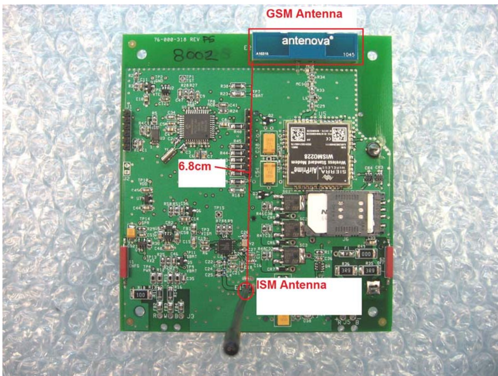
Figure 4 - Internal Photo showing GSM and ISM antennas and distance between
