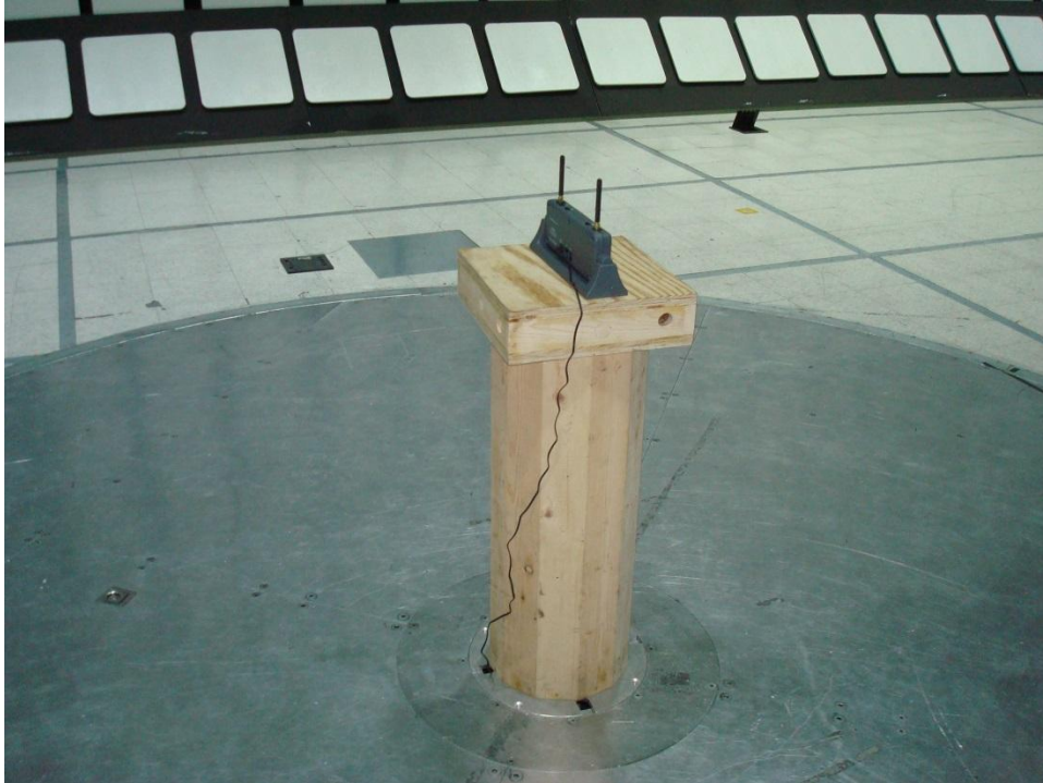
Figure 1 - Radiated Emissions Test Setup
