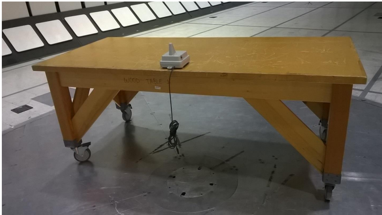
Figure 2 - Test Setup, 30MHz - 1GHz
