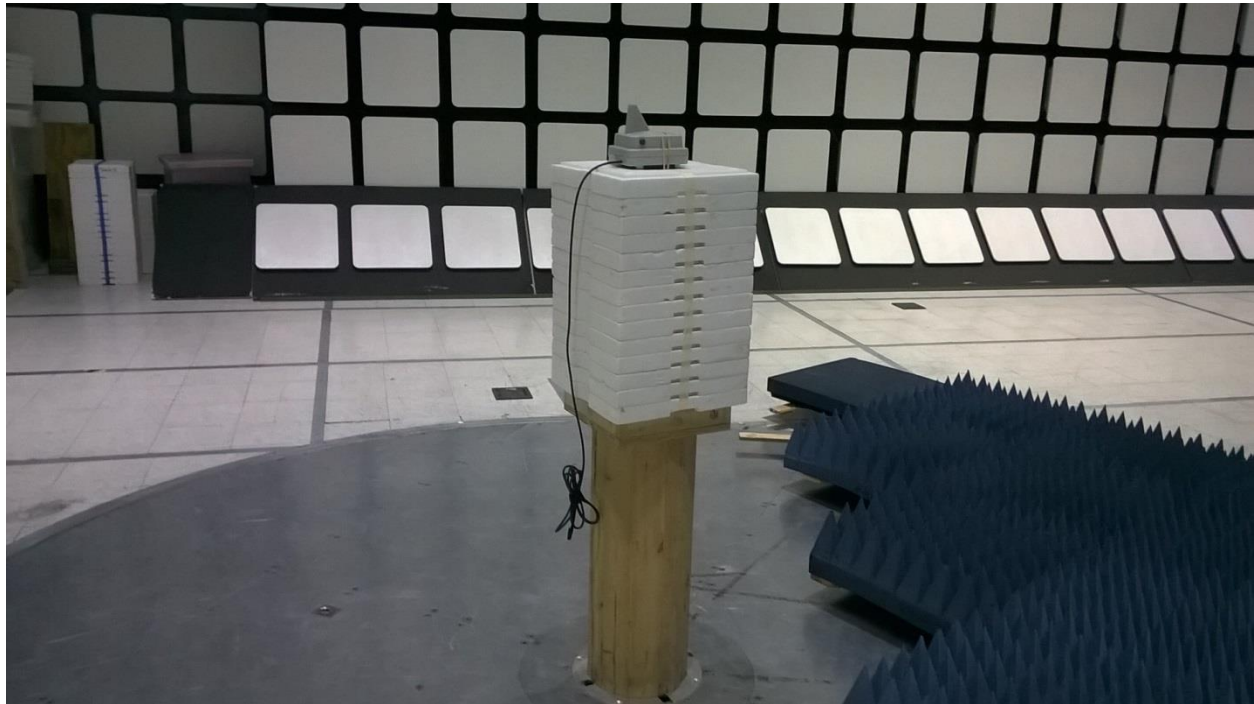
Figure 3 – Test Setup, 1GHz – 18GHz
