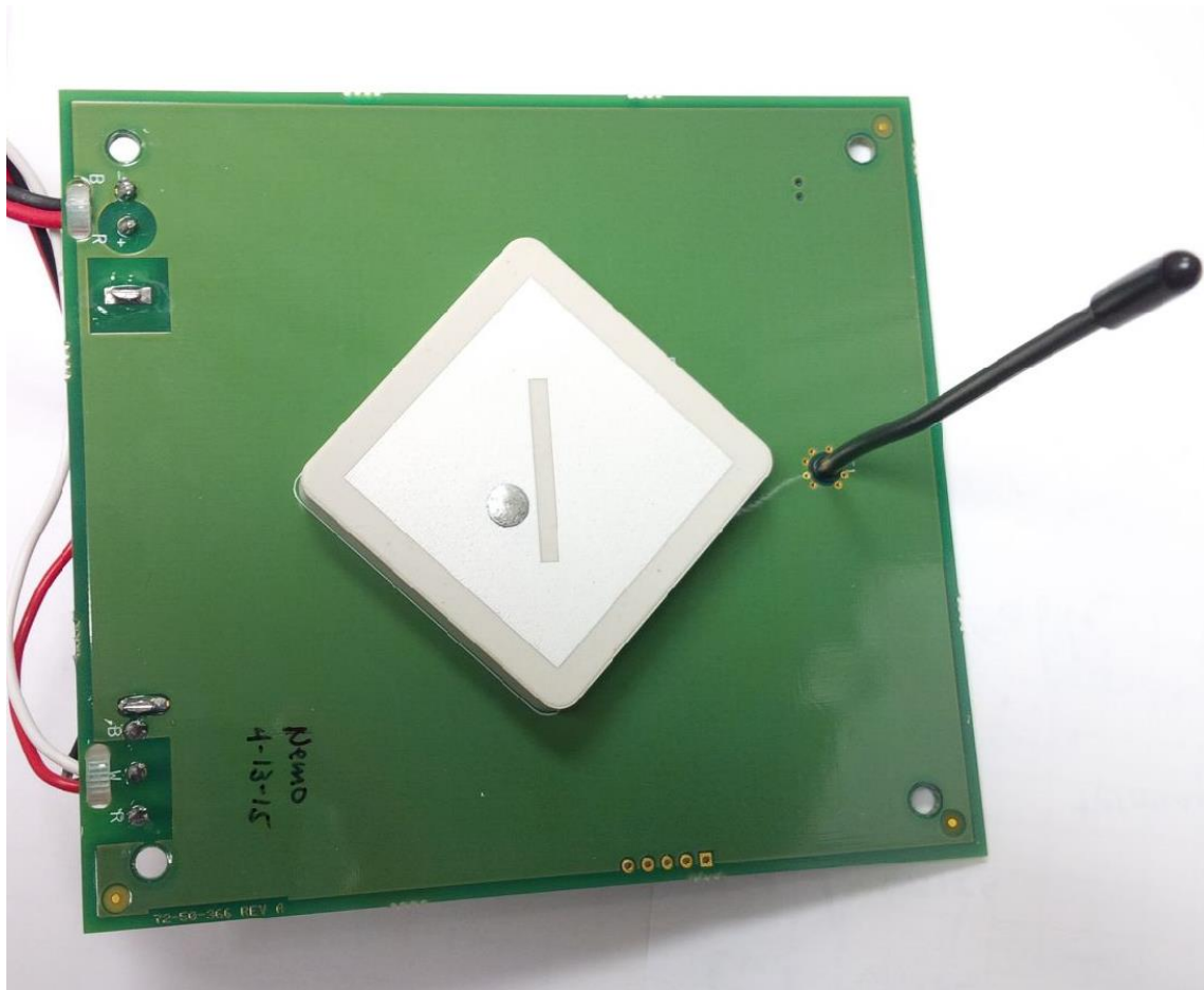
Figure 1 - 915MHz connector and 1.6 GHz satellite antenna
