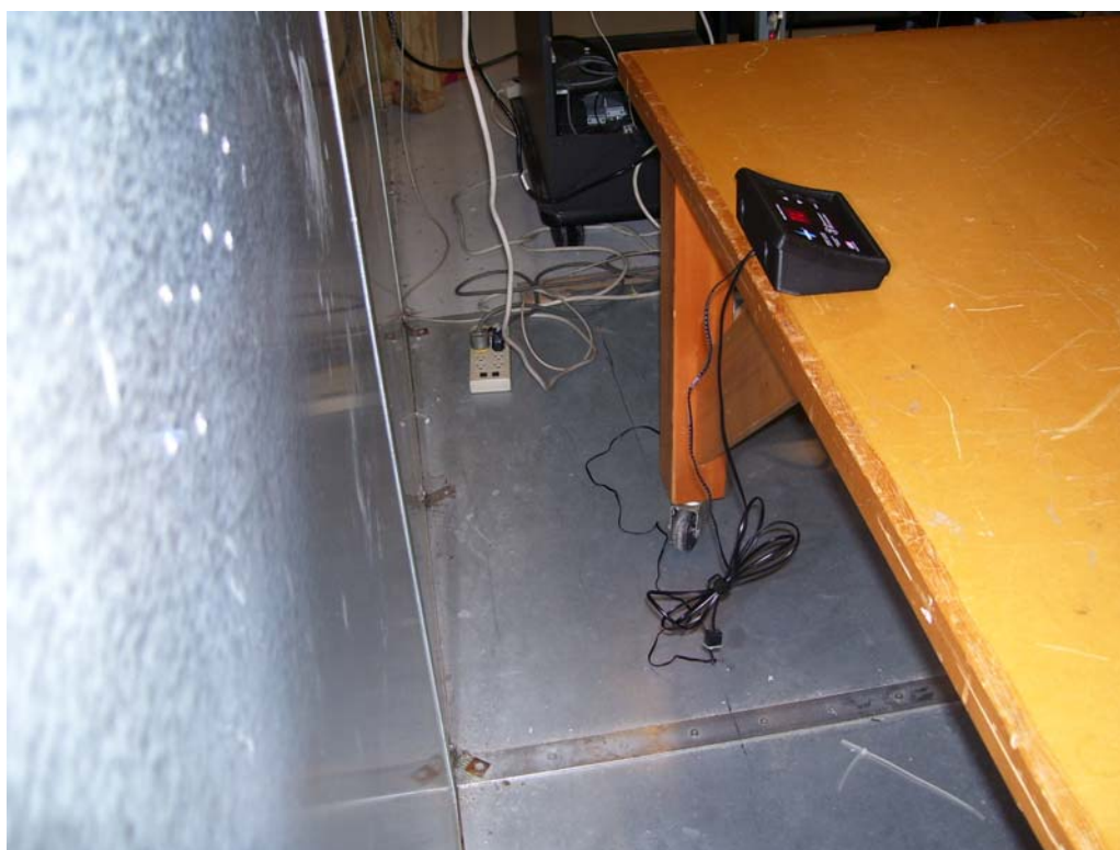
Figure 4 - Conducted Emissions Test Setup
