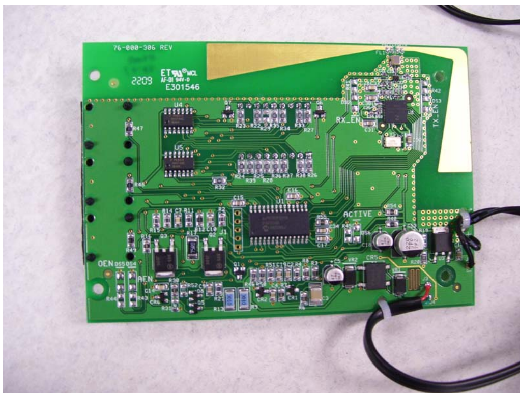
Figure 1 - EUT Internal Photo
