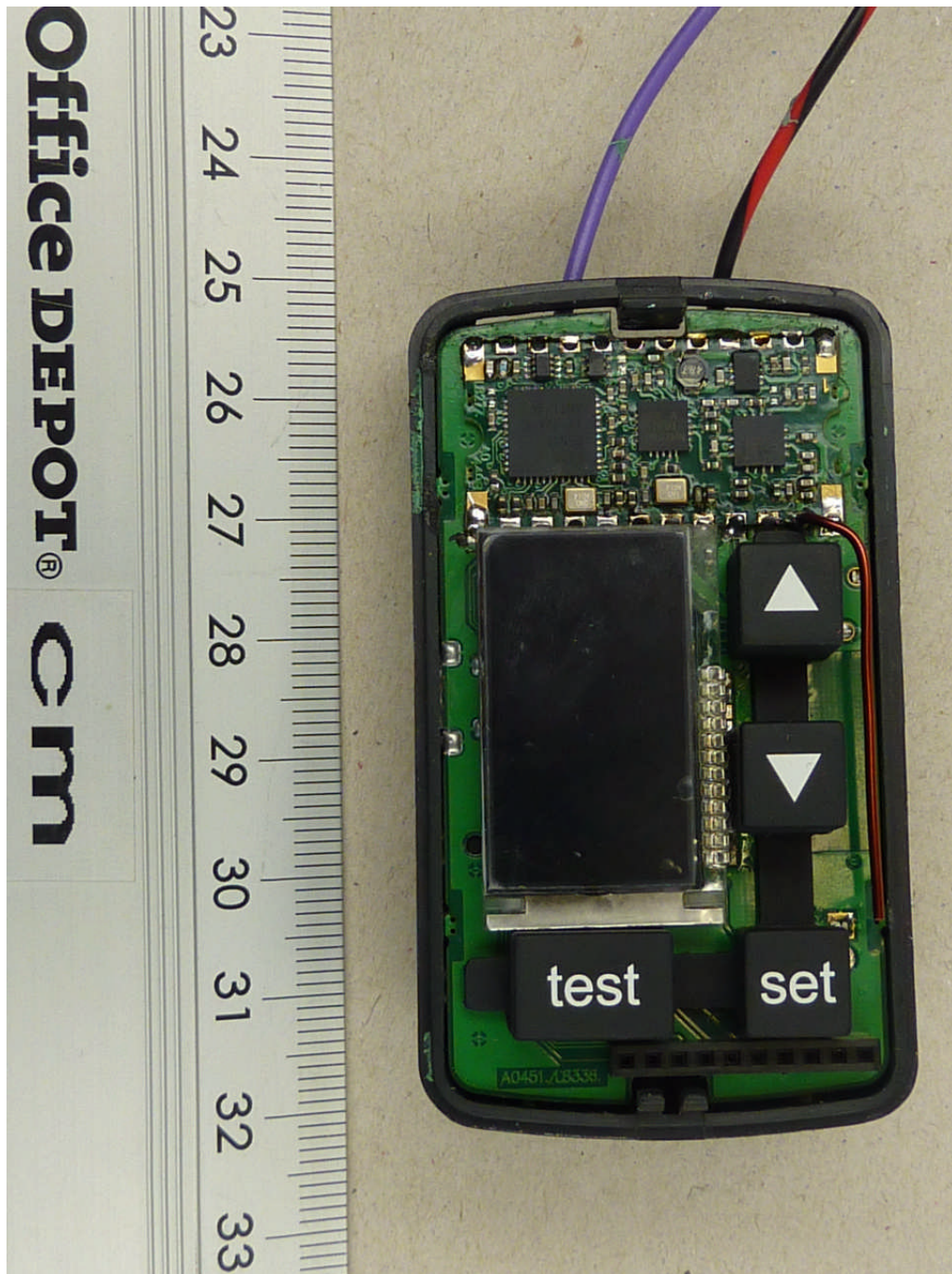
120019_c.JPG: RFS 2, internal view 1
