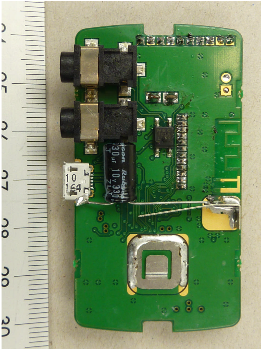
120019_e.JPG: RFS 2, PCB, top view
