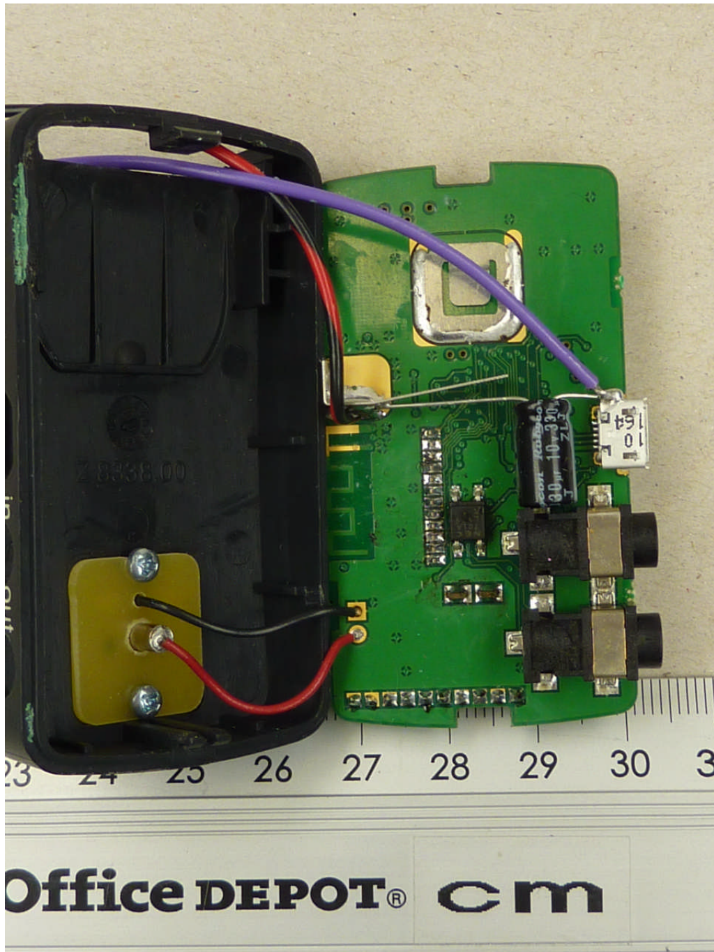
120019_d.JPG: RFS 2, internal view 2
