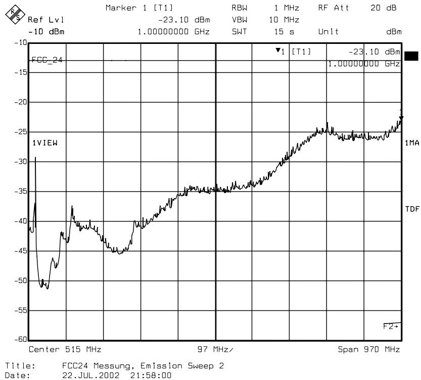
diagram 8.01: carrier on channel 512 (1850,2 MHz), TCH mode
