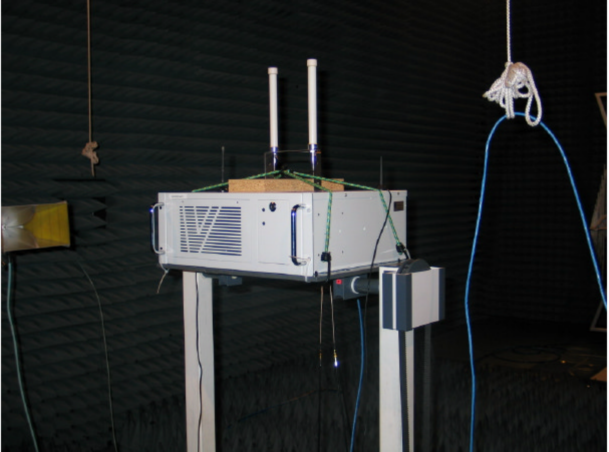
Photo 1: EUT (front and right side, set up together with two antennas AE1)
