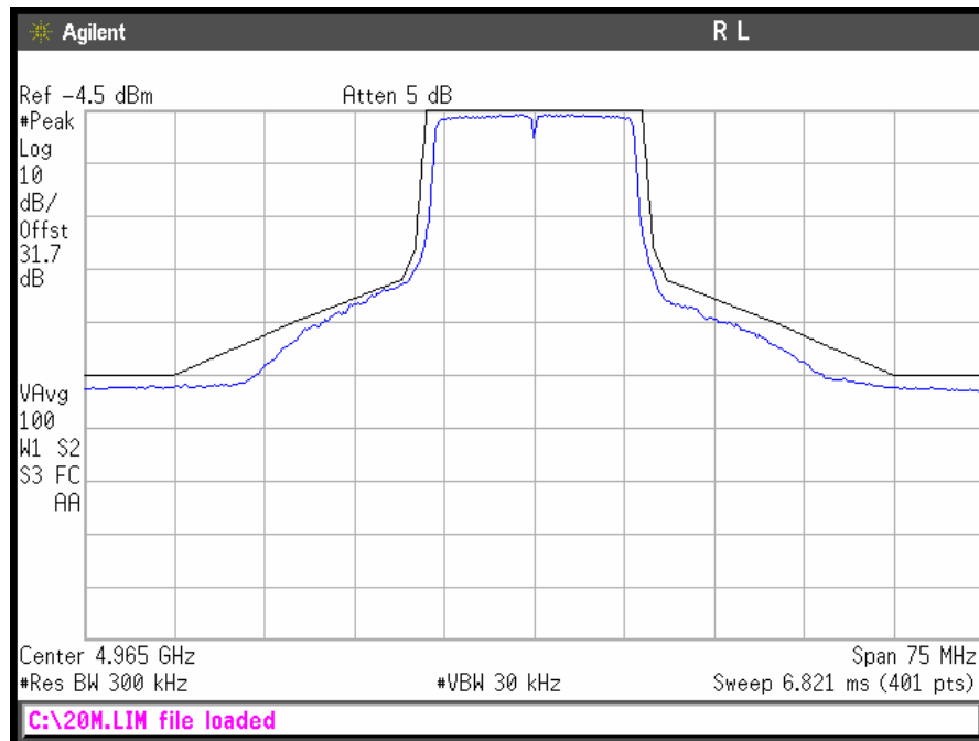
Emission Mask Mid Ch
