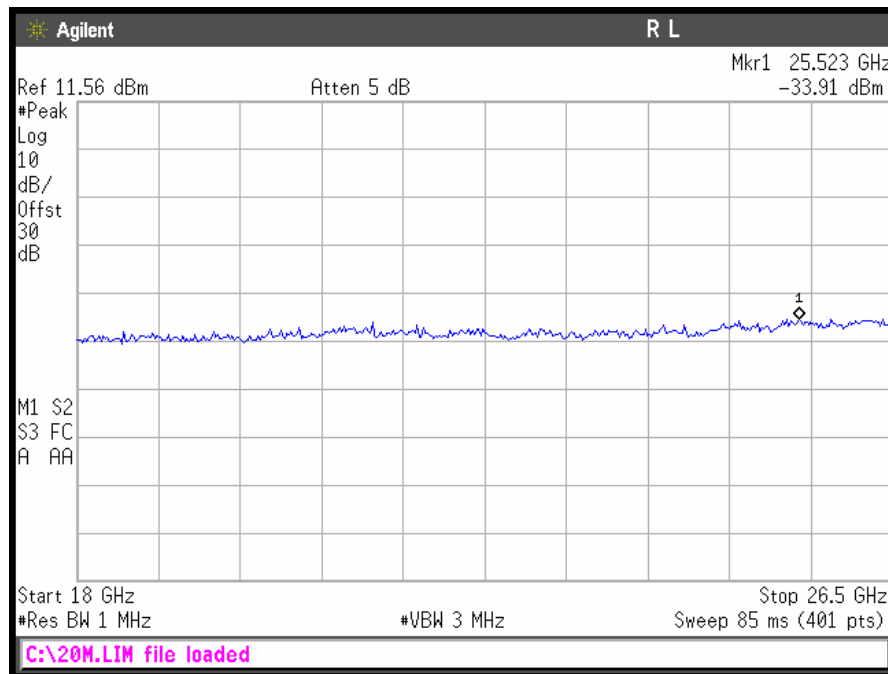
Conducted Spurious Emissions 20 MHz Hi Ch (18 GHz - 26.5 GHz)
