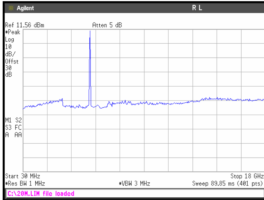
Conducted Spurious Emissions 20 MHz Hi Ch (30 MHz - 18GHz)
