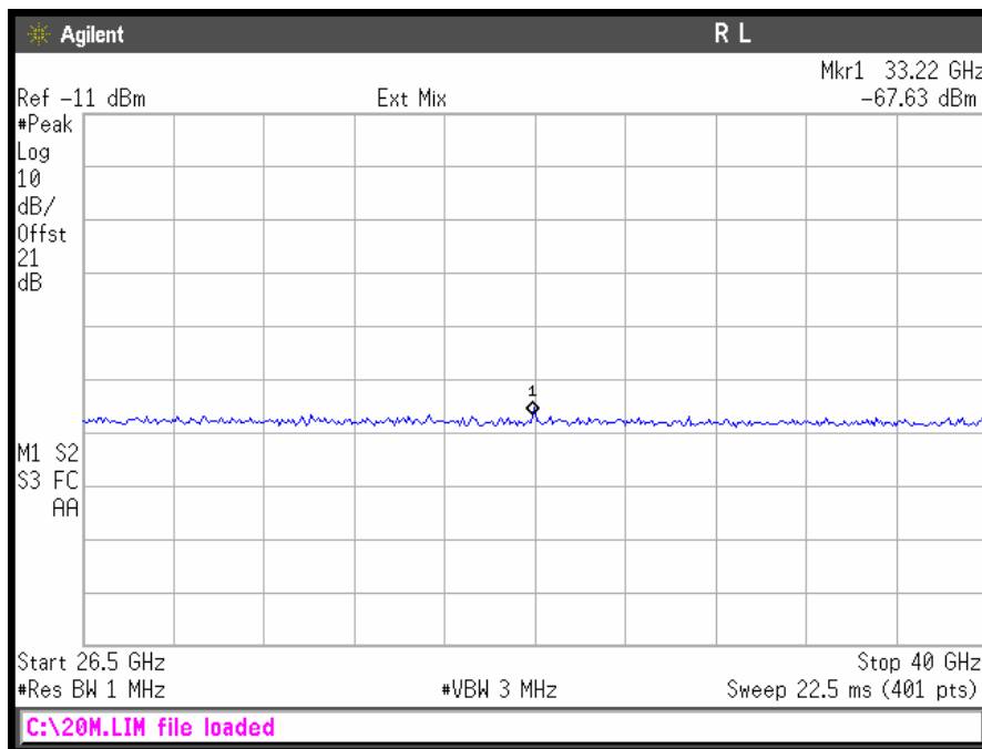
Conducted Spurious Emissions 20 MHz Mid Ch (26.5 GHz – 40 GHz)
