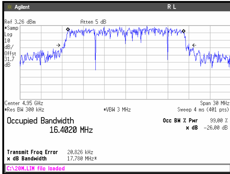
Occupied Bandwidth Low Ch
