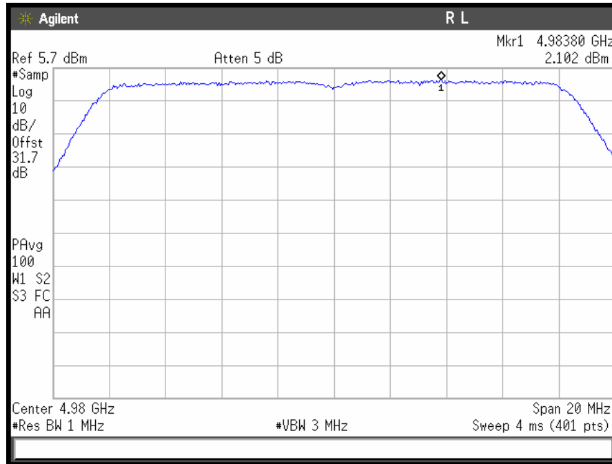
PPSD High Ch 4980MHz
