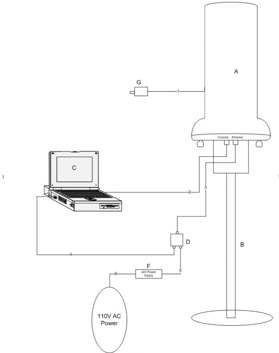
Figure 1. Block Diagram of Test Configuration (Unintentional)
