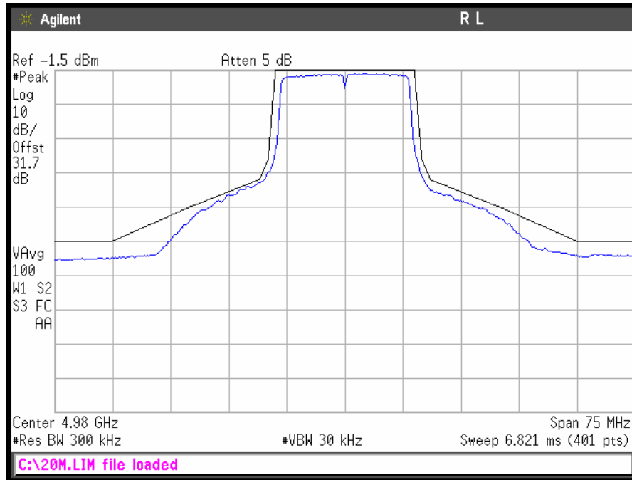
Emission Mask High Ch
