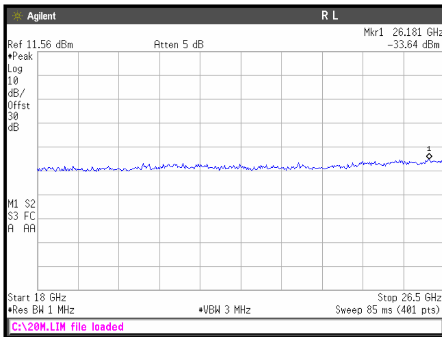
Conducted Spurious Emissions 20 MHz Mid Ch (18 GHz – 26.5 GHz)
