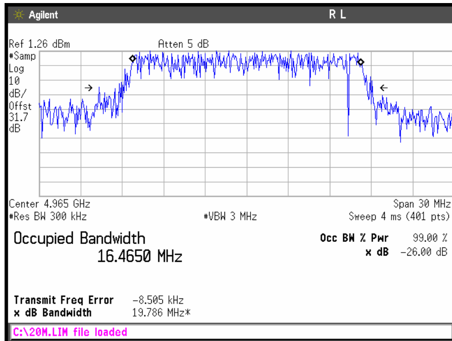
Occupied Bandwidth Mid Ch
