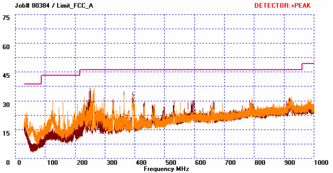
Radiated Emissions Test Plot
