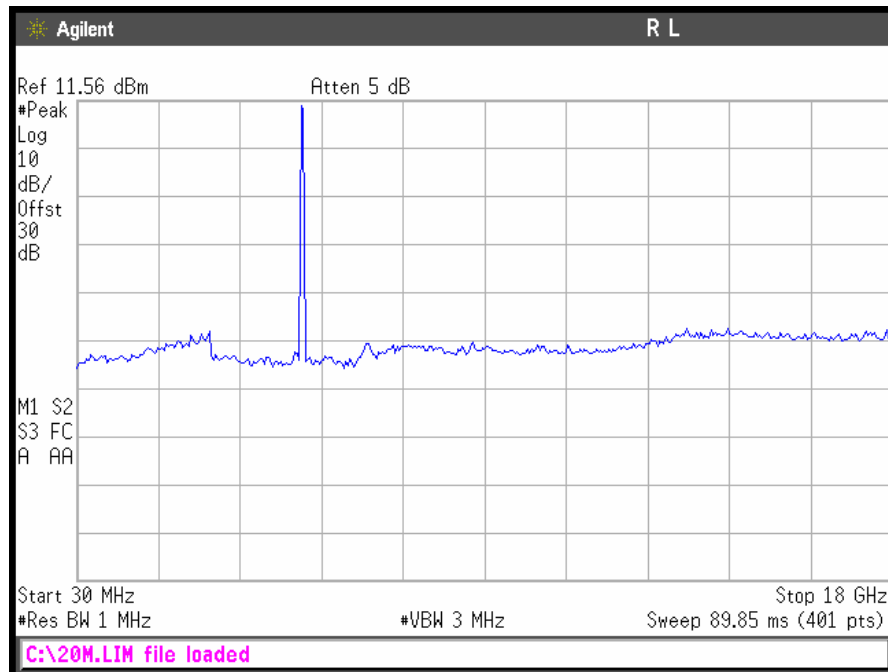
Conducted Spurious Emissions 20 MHz Mid Ch (30 MHz - 18GHz)
