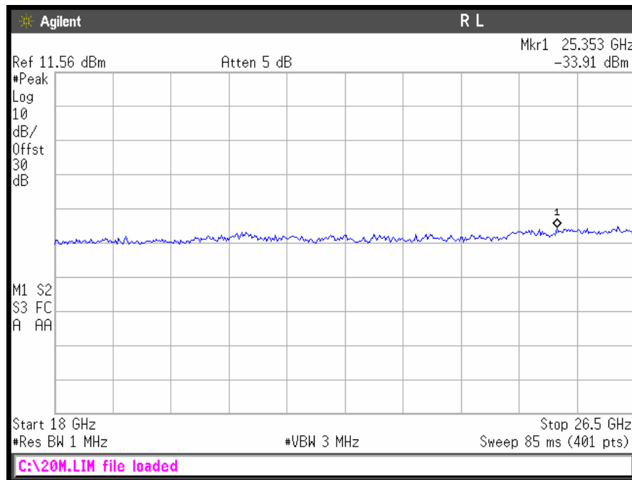
Conducted Spurious Emissions 20 MHz Low Ch (18 GHz - 26.5 GHz)
