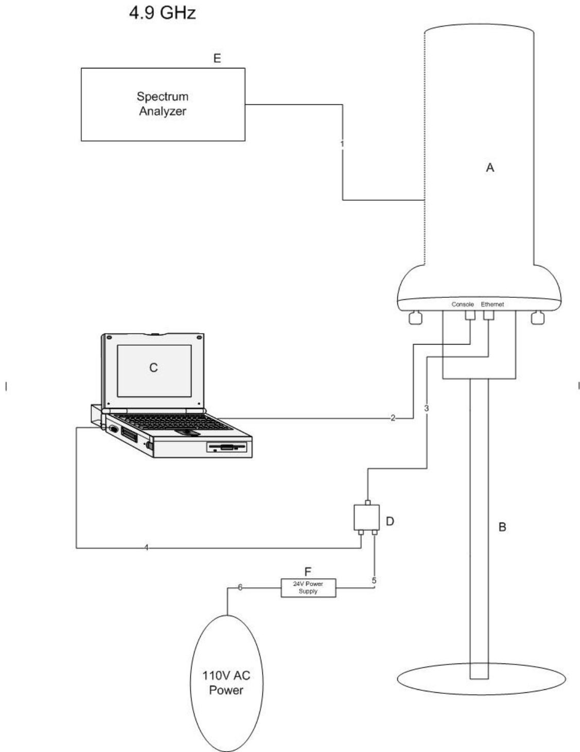
Figure 2. Block Diagram of Test Configuration (Intentional)
