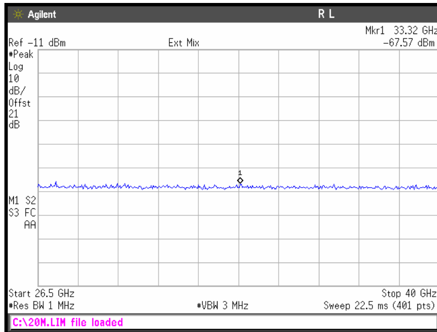
Conducted Spurious Emissions 20 MHz Hi Ch (26.5 GHz – 40 GHz)
