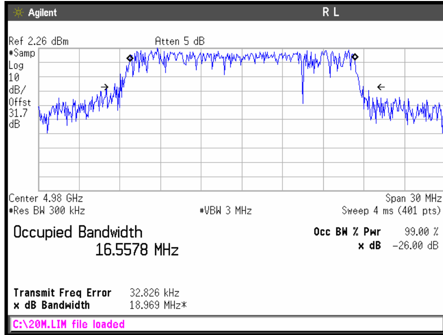
Occupied Bandwidth High Ch
