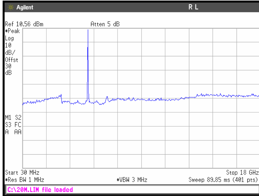
Conducted Spurious Emissions 20 MHz Low Ch (30 MHz - 18GHz)
