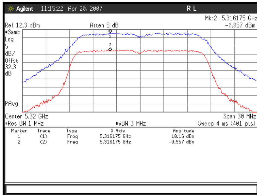
Plot 19. Peak Excursion Ratio for Low Band High Ch, 5320MHz
