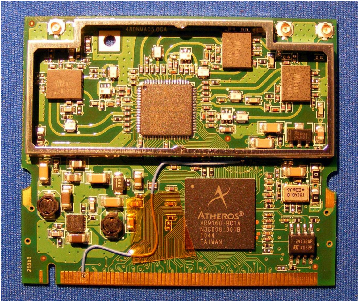
DNMA83 Front with shield removed
