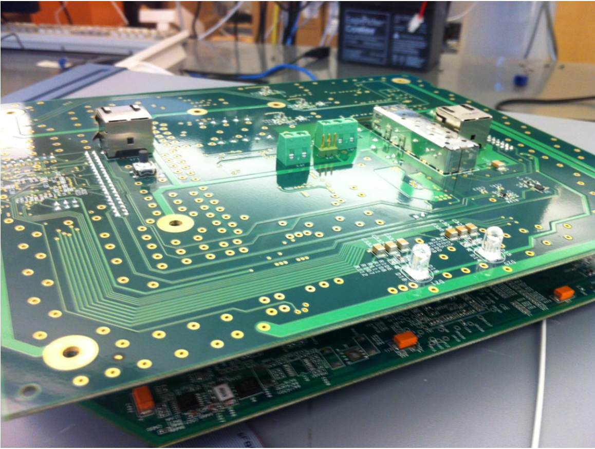
Board Set: Motherboard on Top
