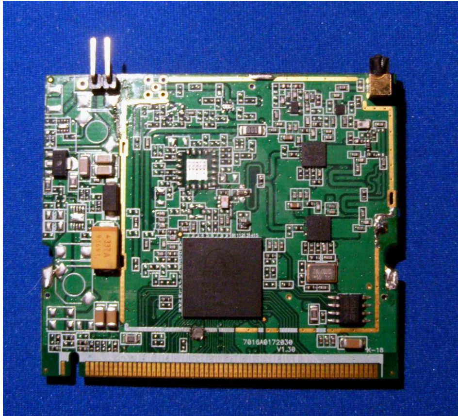
RF Assy with shield removed
