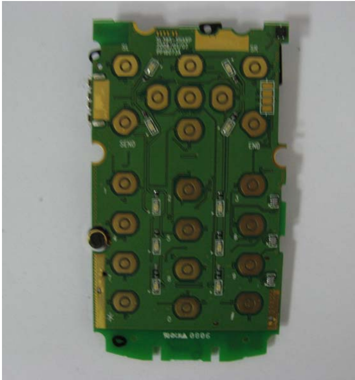
Picture 1: the top view of the PCB
