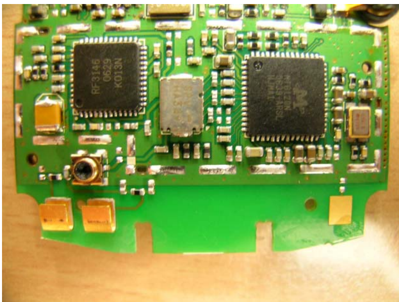
Picture 6: Radio part with the shielding cover removed—2
