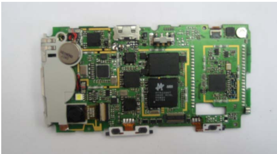
Picture 4: The back view of the PCB with the shielding cover removed
