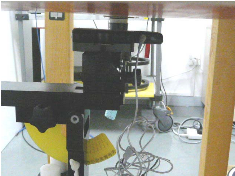
Body SAR back to the phantom, with earphone
