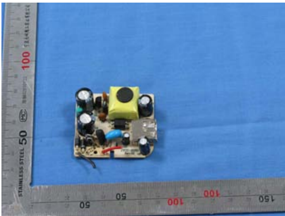
Main board of Adaptor(face)
