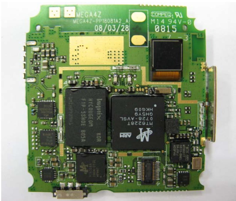
Picture 1: the top view of the PCB
