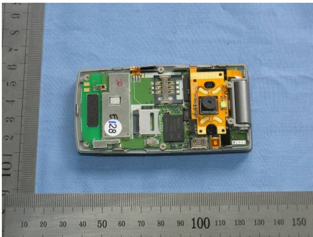
Picture 5 Mainboard (inverse)
