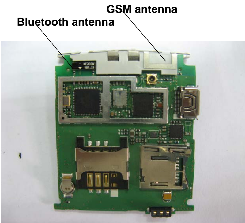
Picture 2: the back view of the PCB
